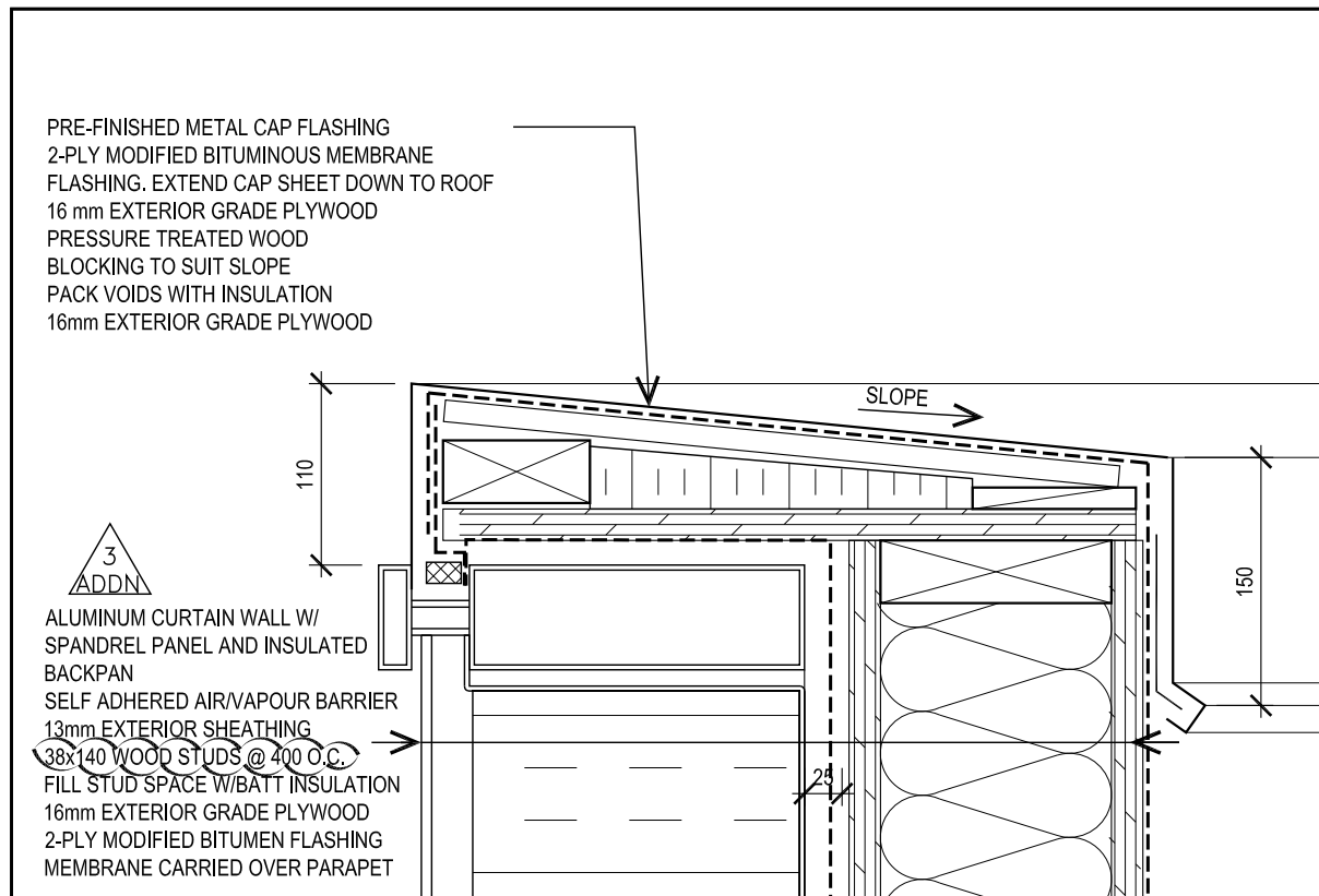
1 PARAPET CAP @ CURTAIN WALL 337 SCALE: 1:5
