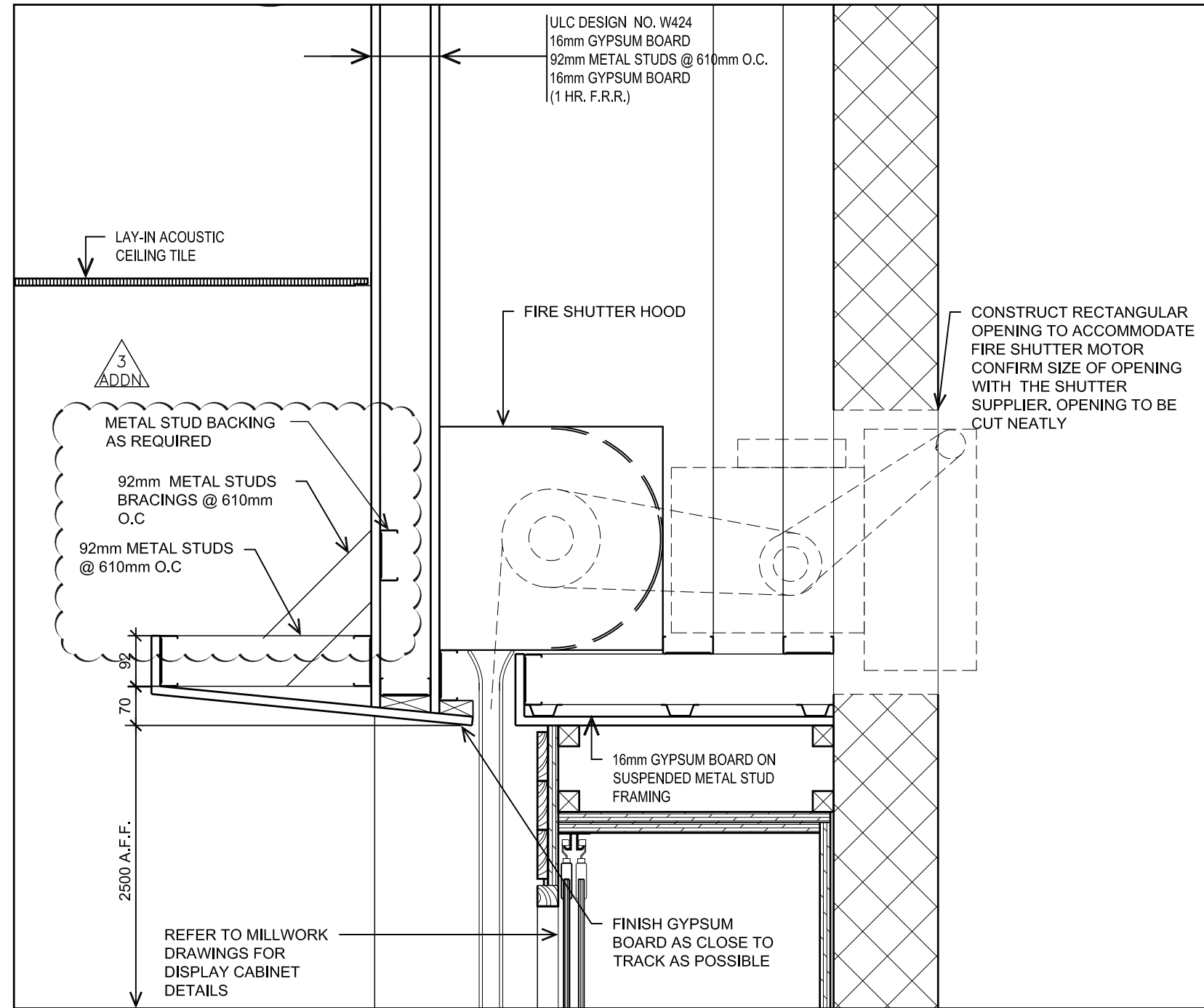
6 FIRE SHUTTER & BULKHEAD DETAIL 313 SCALE: 1:10
