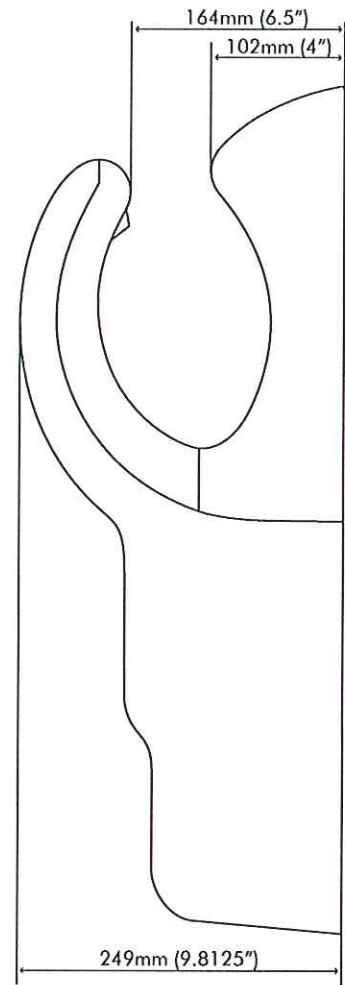
SIDE ELEVATION
