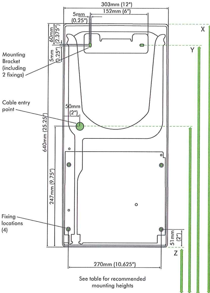
REAR ELEVATION
