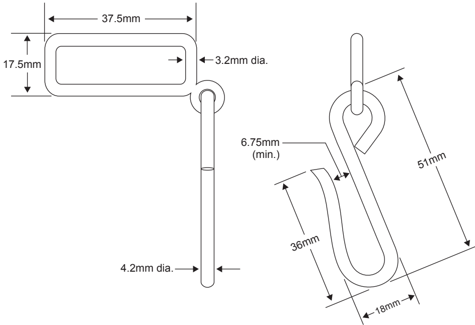
Sword Hook Assembly
