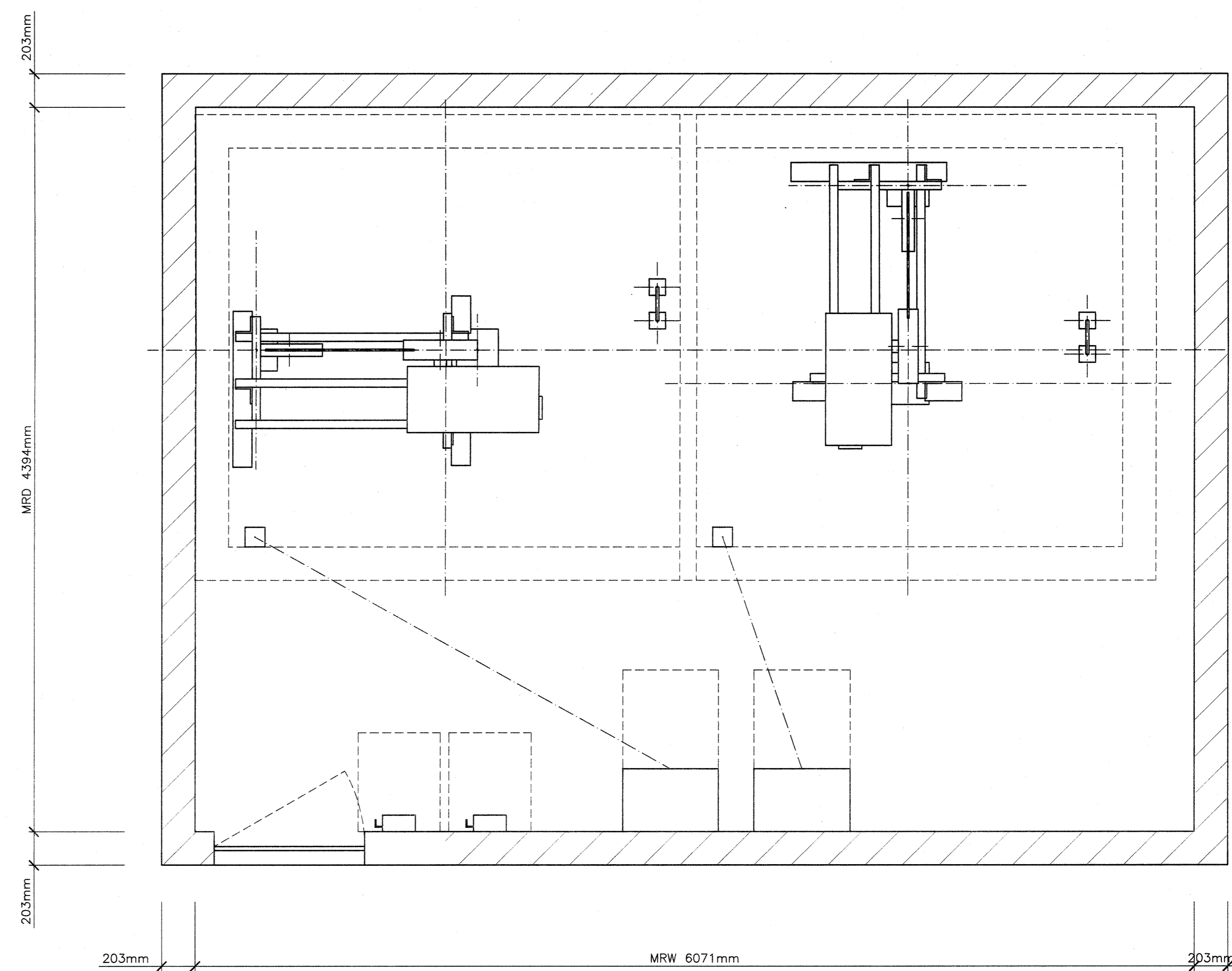
MACHINE ROOM
