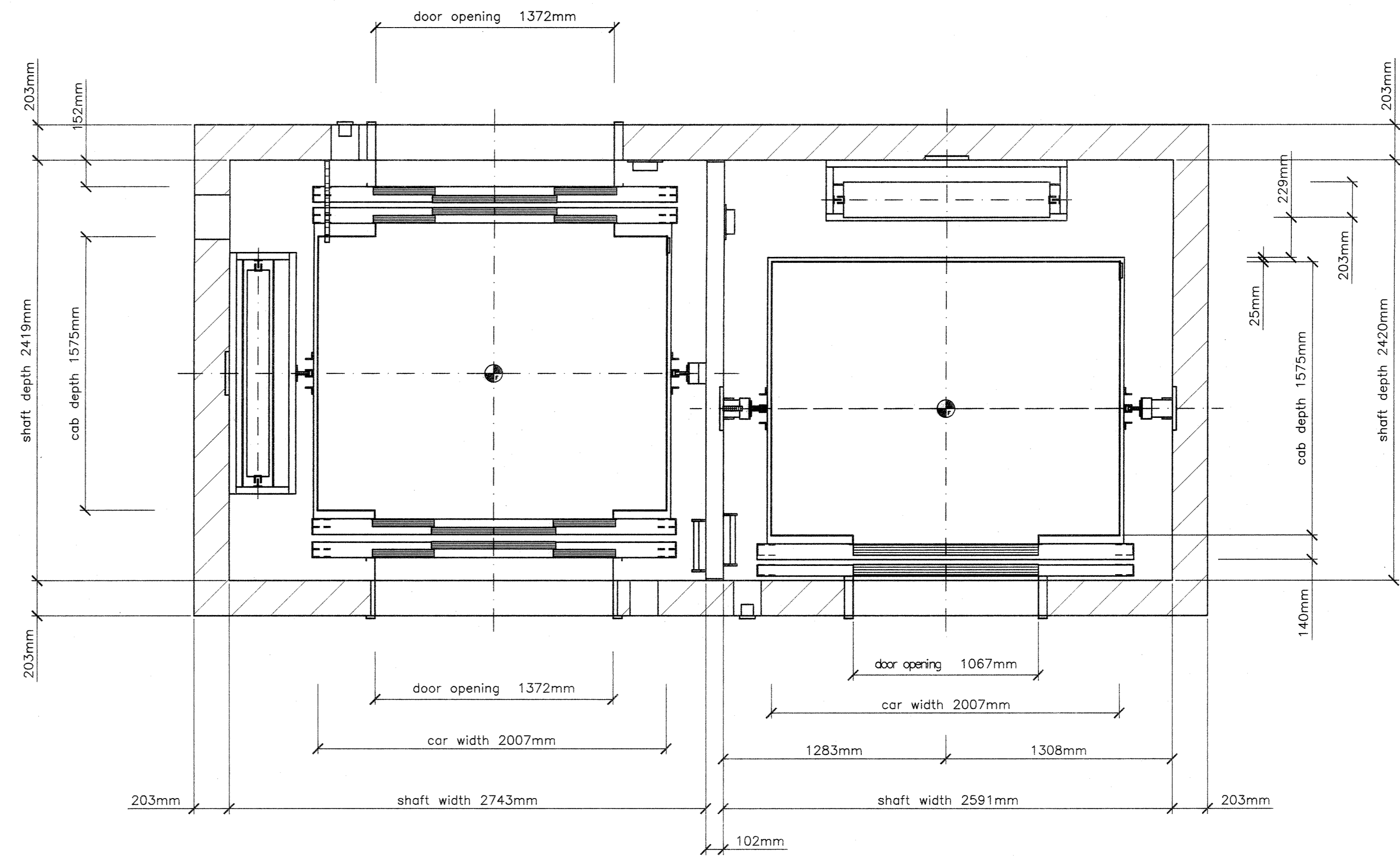
PLAN VIEW
