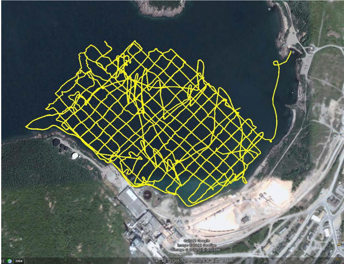
Figure 3: Submerged Aquatic Vegetation Tracks from 2012
