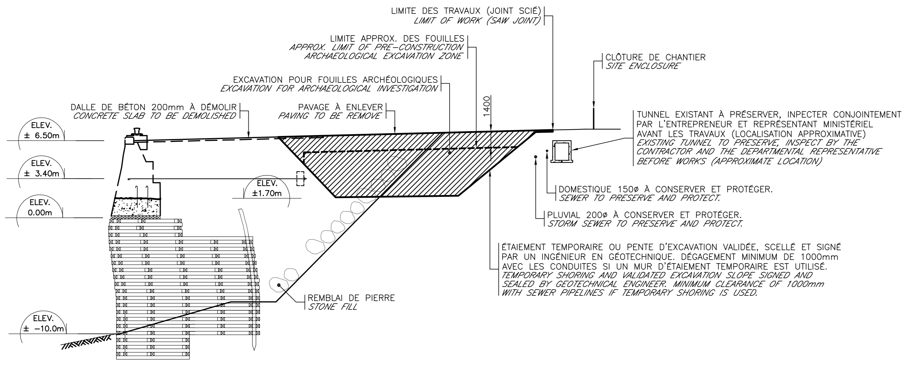
COUPE TYPE TYPICAL SECTION 48 17/17 0 10m 1: 200
