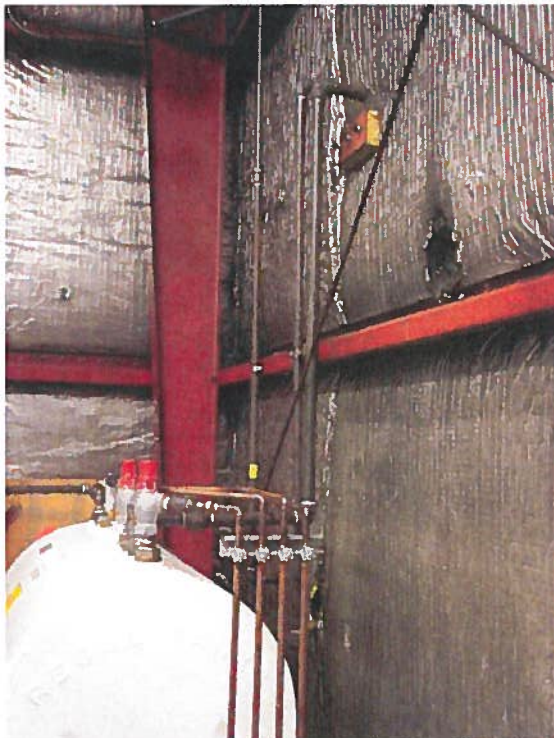
PHOTO 10: PUMPHOUSE BUILDING AND DIESEL AUXILIARY (DAY) TANK Fuel transfer and Overflow/Vent piping
