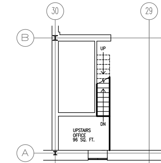
MEZZANINE FLOOR PLAN Scale: NTS
