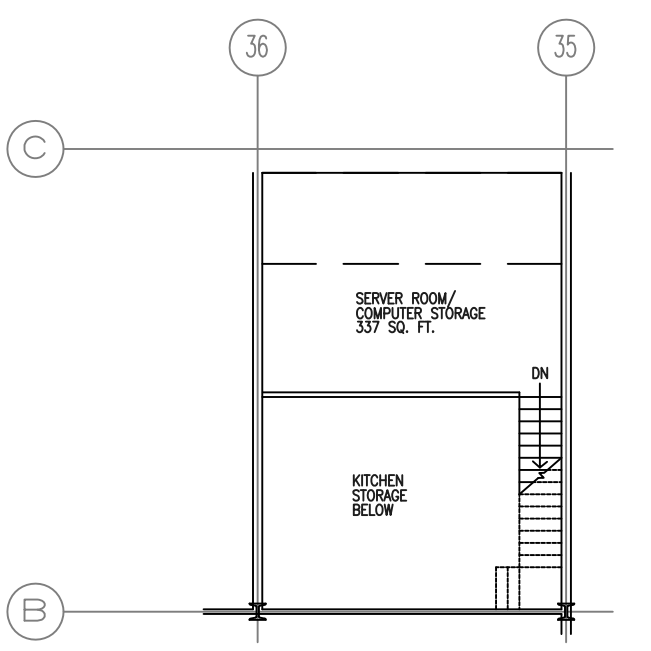
MEZZANINE FLOOR PLAN Scale: N1/8"
