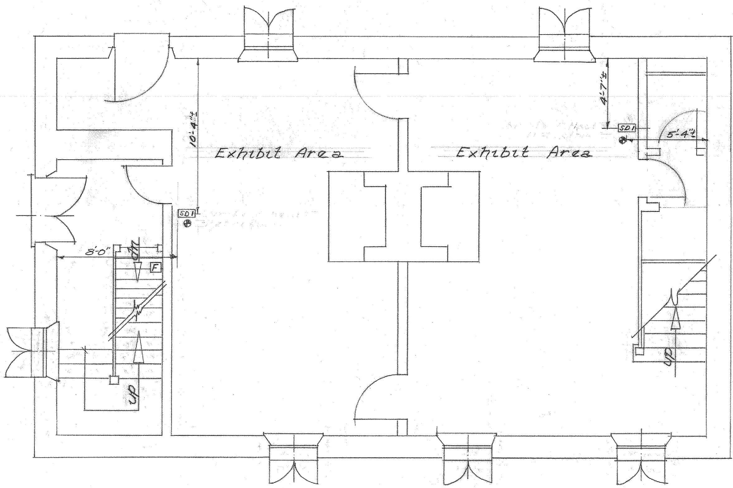
Ground Floor
