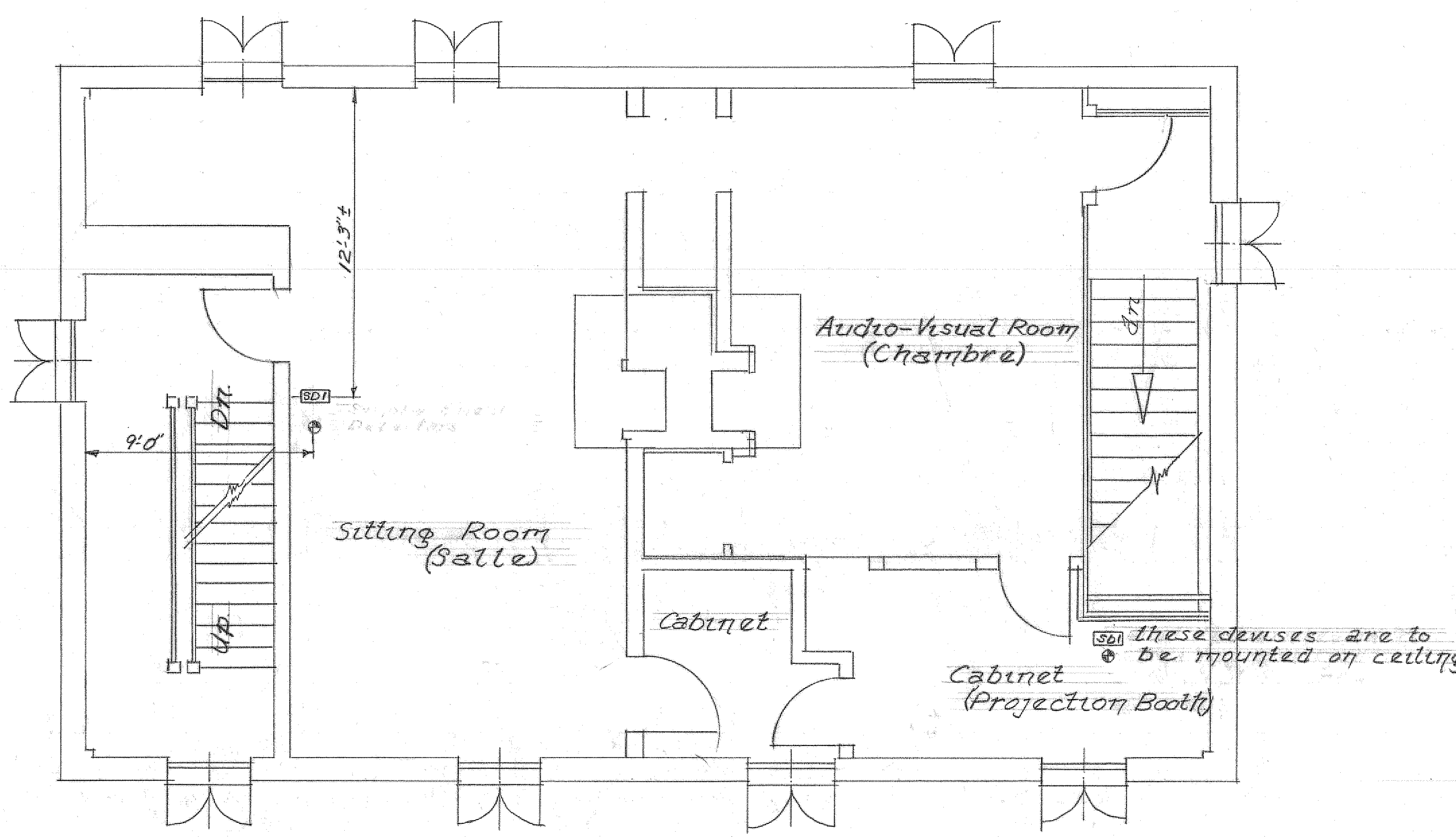
First Floor
