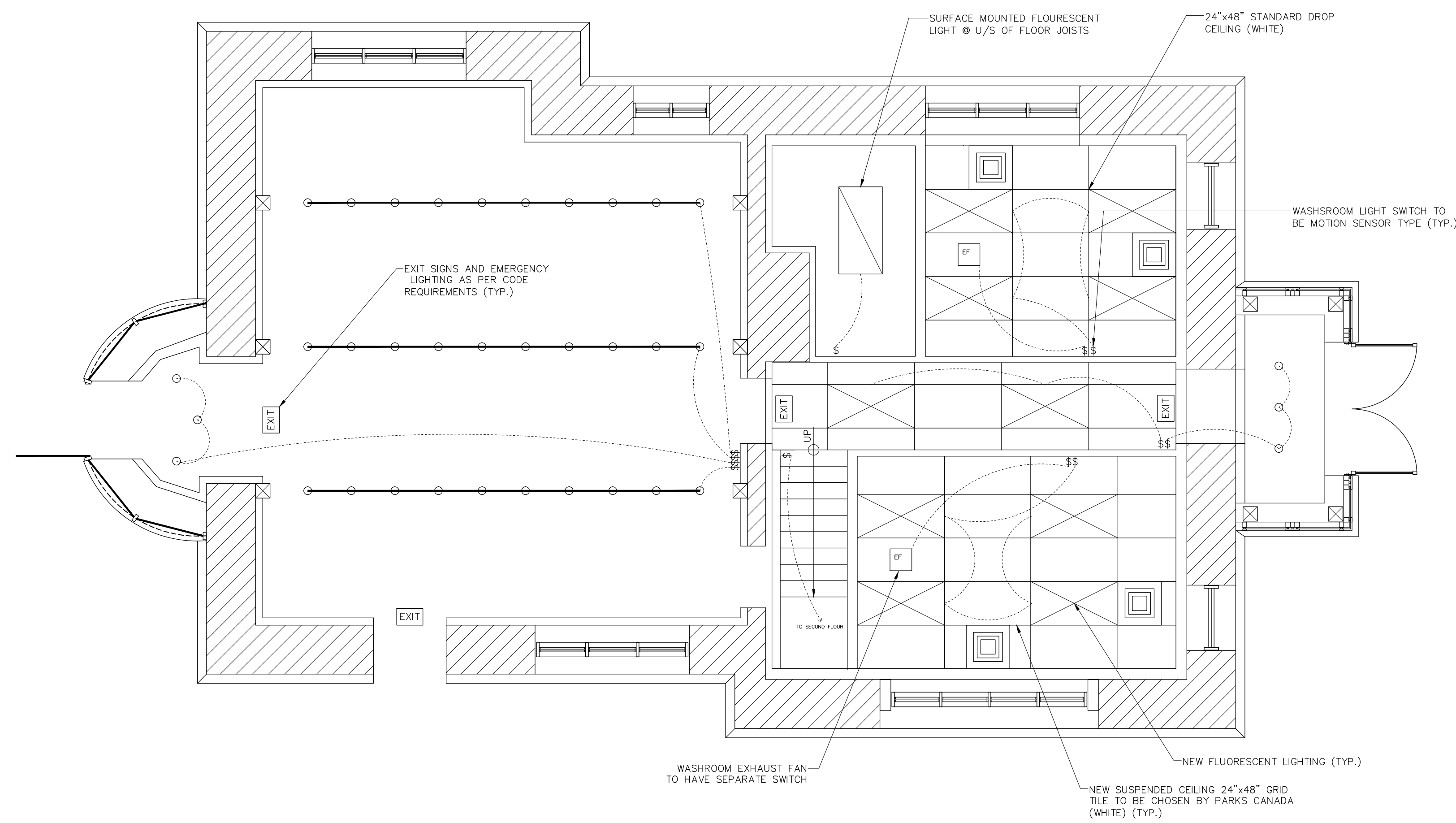
GROUND FLOOR PLAN - LIGHTING
