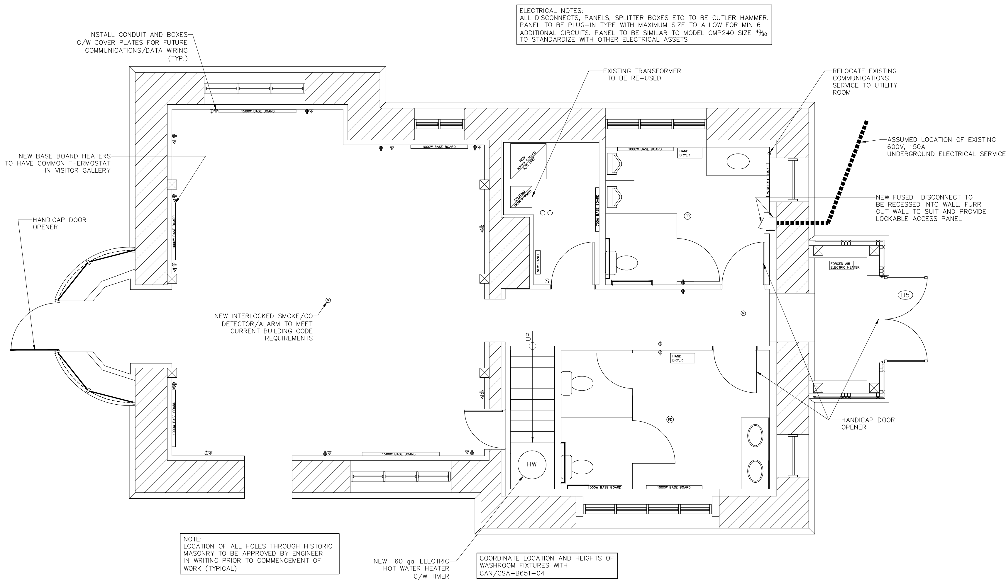
GROUND FLOOR PLAN - ELECTRICAL
