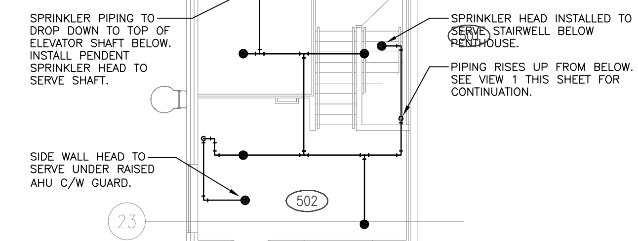
2 PENTHOUSE PLAN 1:100
