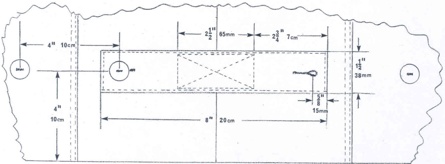
SUPPRESSION STRAP DETAIL
