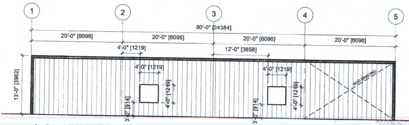
1.0 - SIDEWALL C
