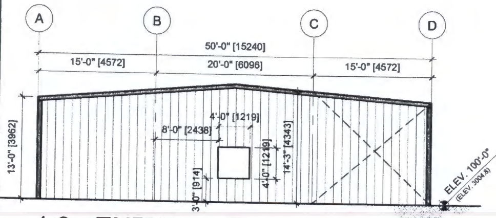
1.0 - ENDWALL D NON-EXPANDABLE END FRAME
