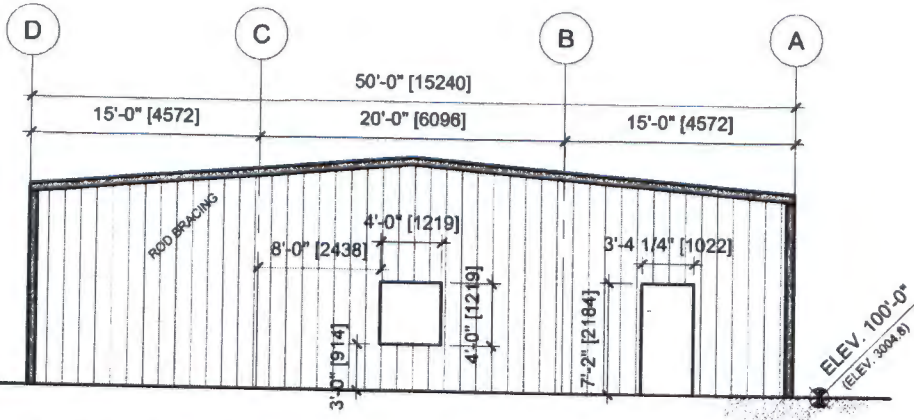
1.0 - ENDWALL B EXPANDABLE END FRAME
