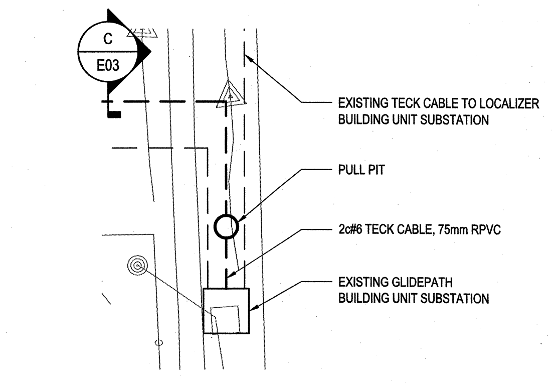
2 ENLARGED SITE PLAN SCALE 1:500
