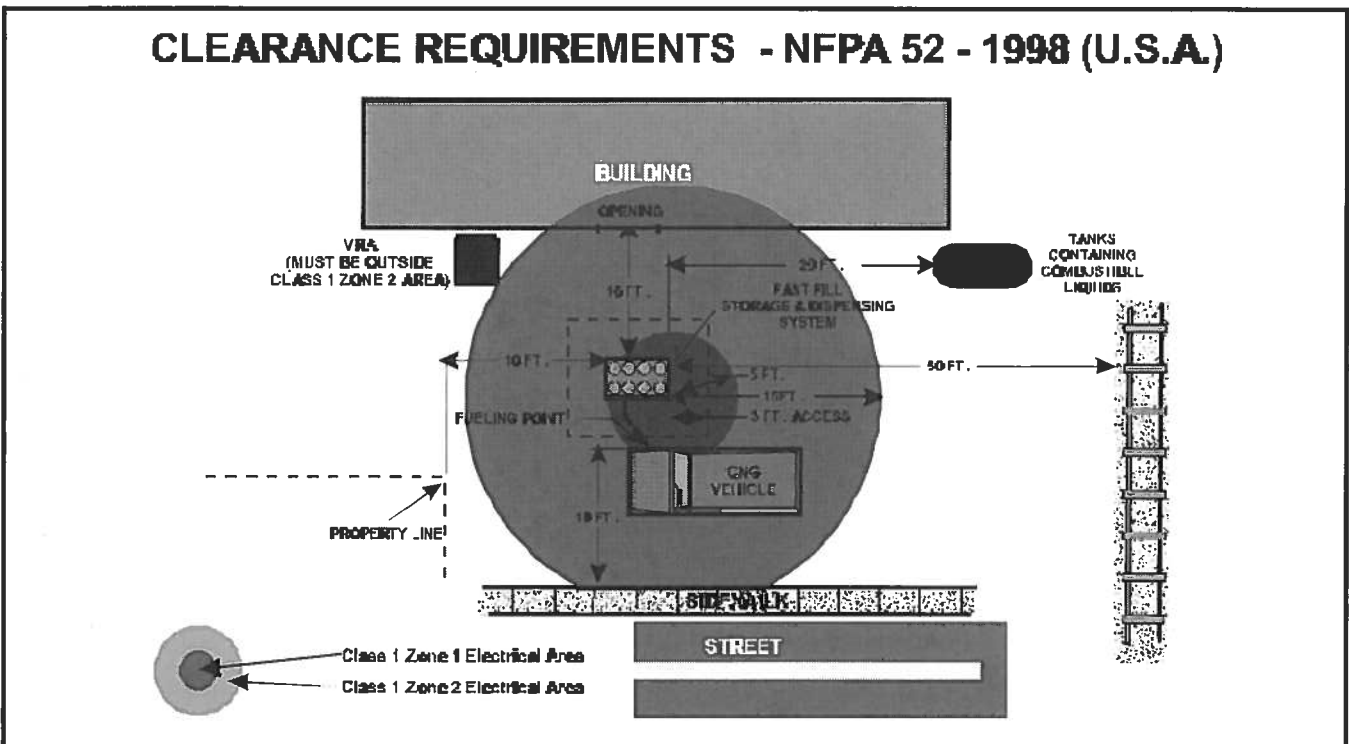
Figure 8 Location of the Fast Fill Storage System (U.S.A.)
