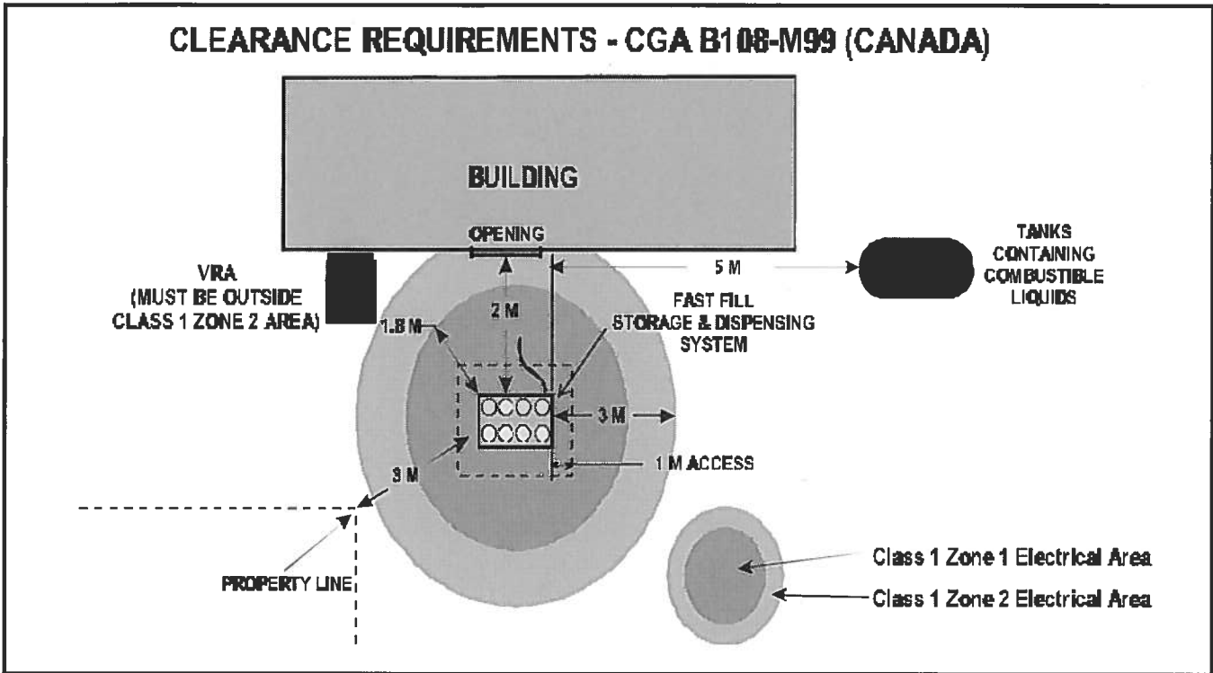
Figure 7 Location of the Fast Fill Storage System (Canada)
