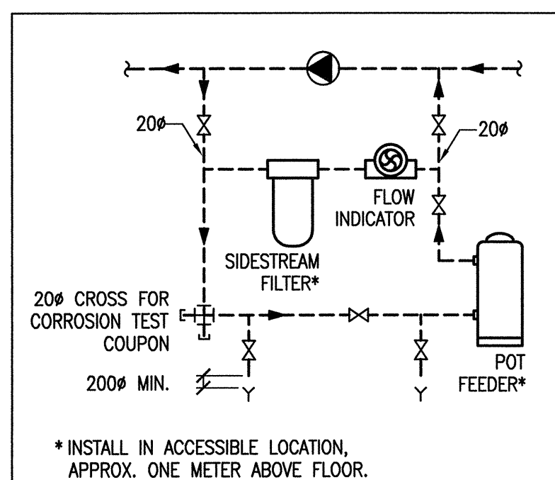
1 CHEMICAL POT FEEDER NTS
