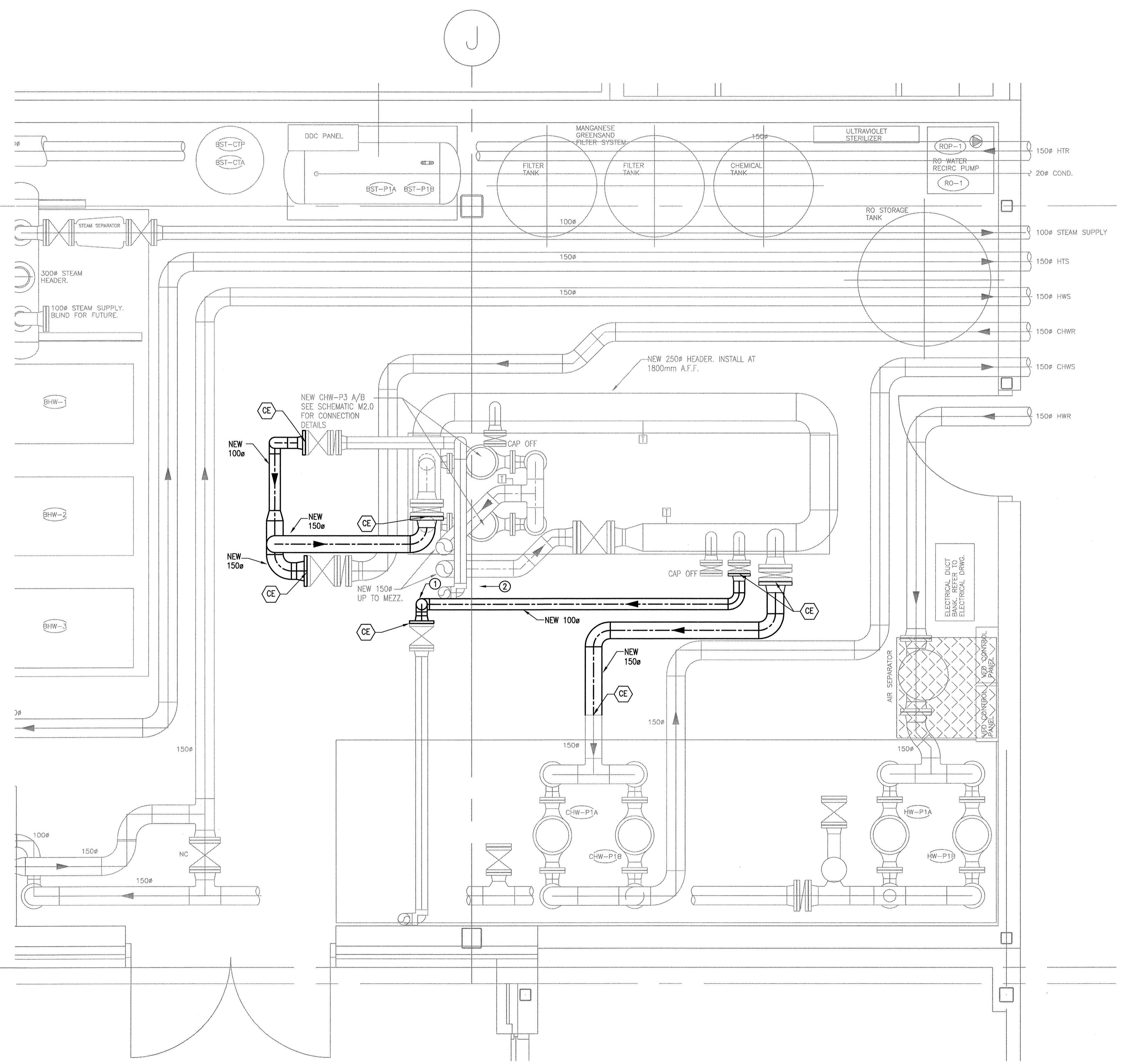
MECH ROOM PHASE 2 NEW LAYOUT PLAN 1:20
