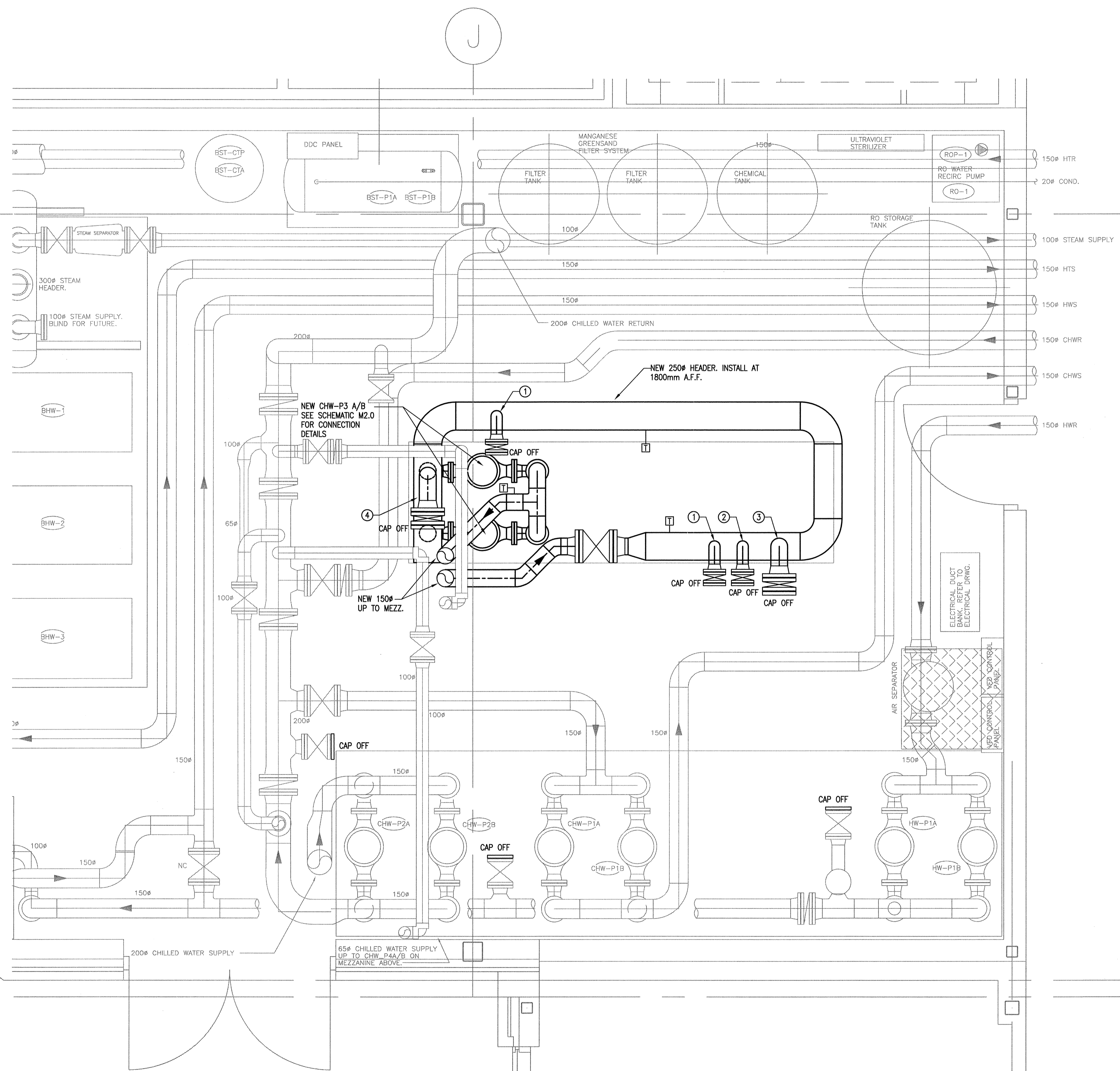
MECH ROOM PHASE 1 NEW LAYOUT PLAN
