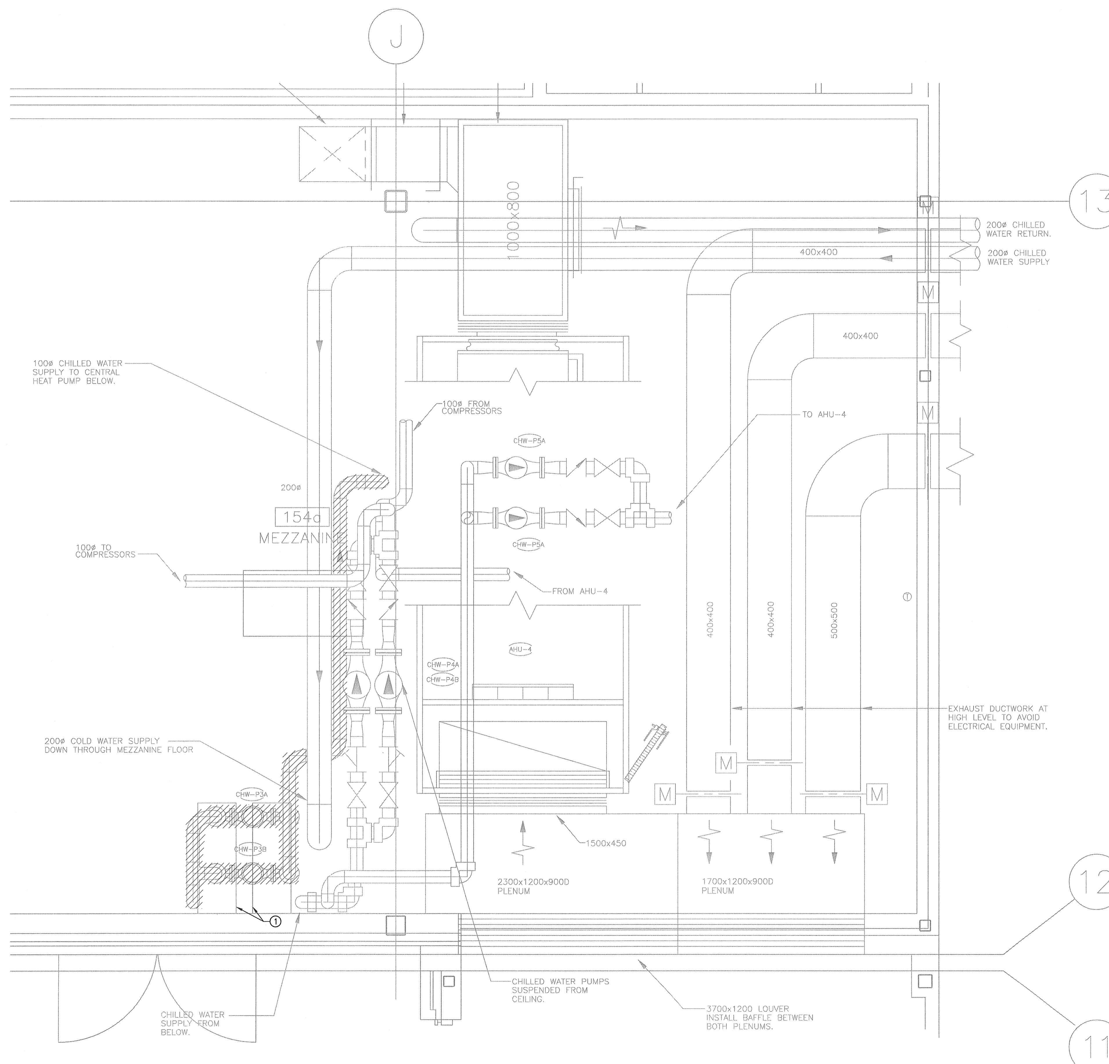
MEZZANINE PHASE 1 DEMOLITION PLAN 1:20
