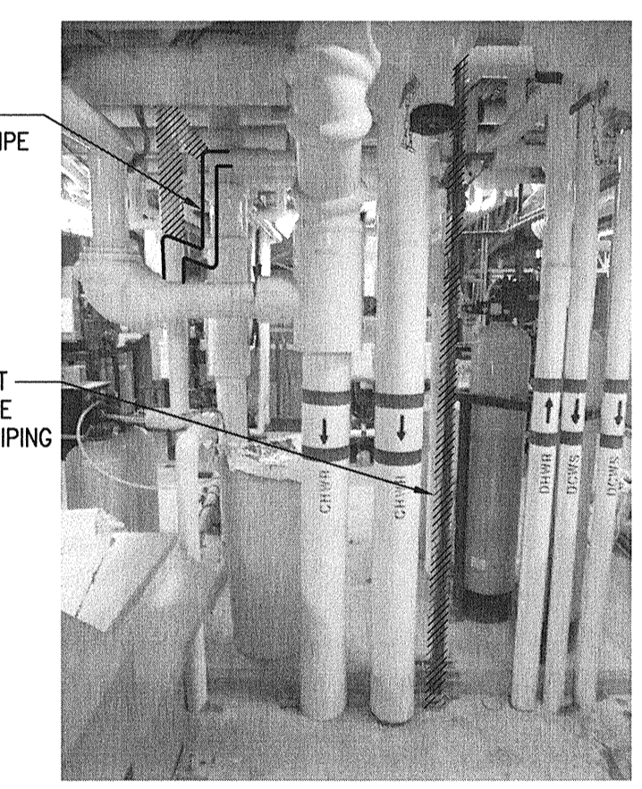
PHOTO #1 - PIPE ROUTING N.T.S.
