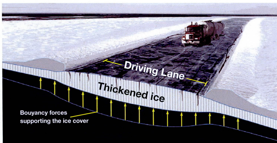
Figure 24 Effect of cleared road on ice thickness
