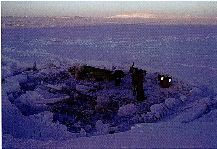
Figure 7 Breakthrough of a D10 Caterpillar tractor following formation of a circumferential crack pattern
