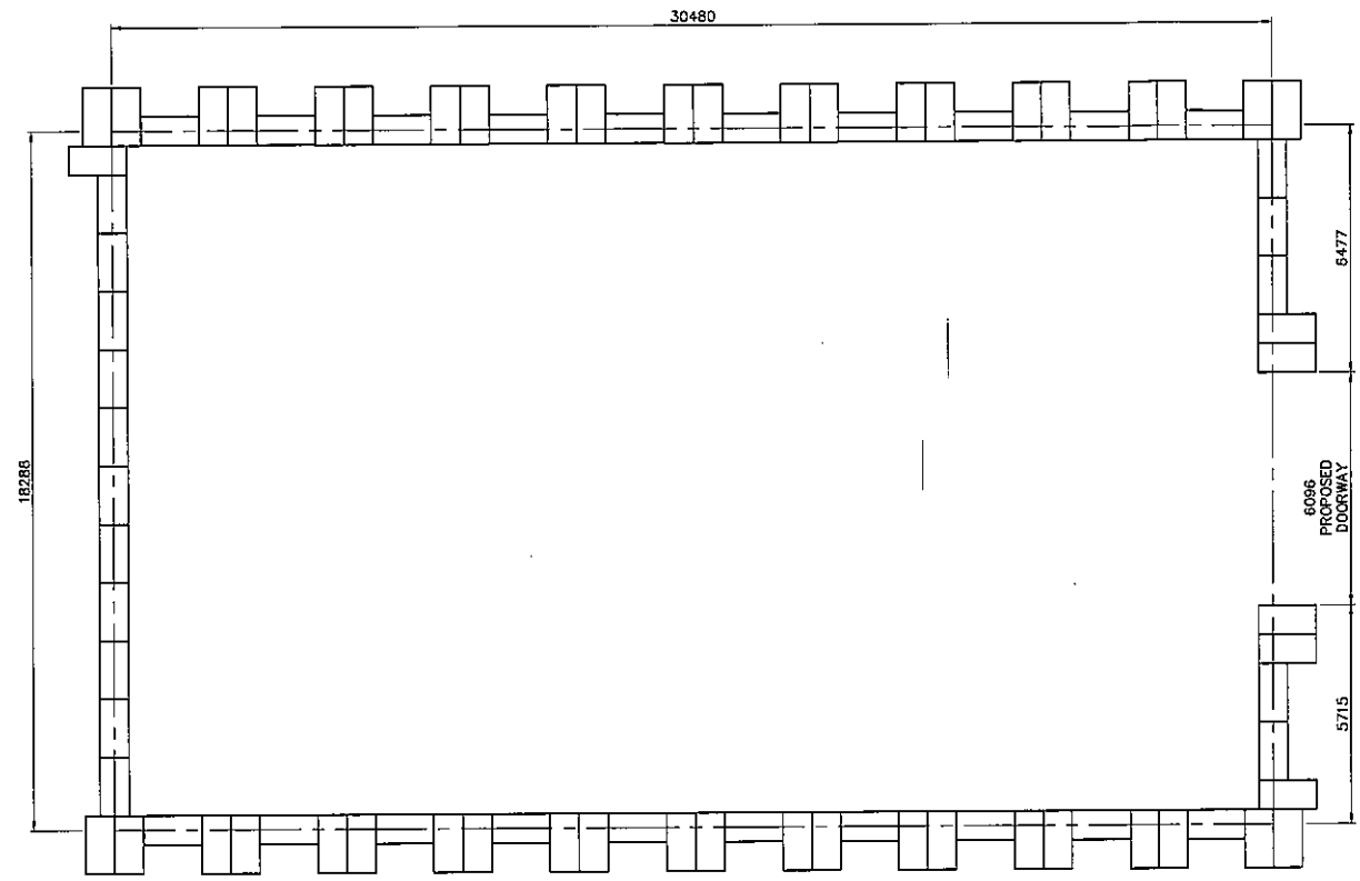
LOCK BLOCK LAYOUT 1:100
