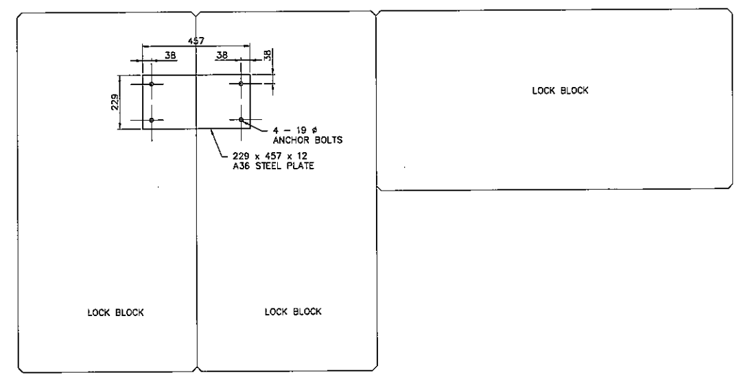
PLATING DETAIL 1:10
