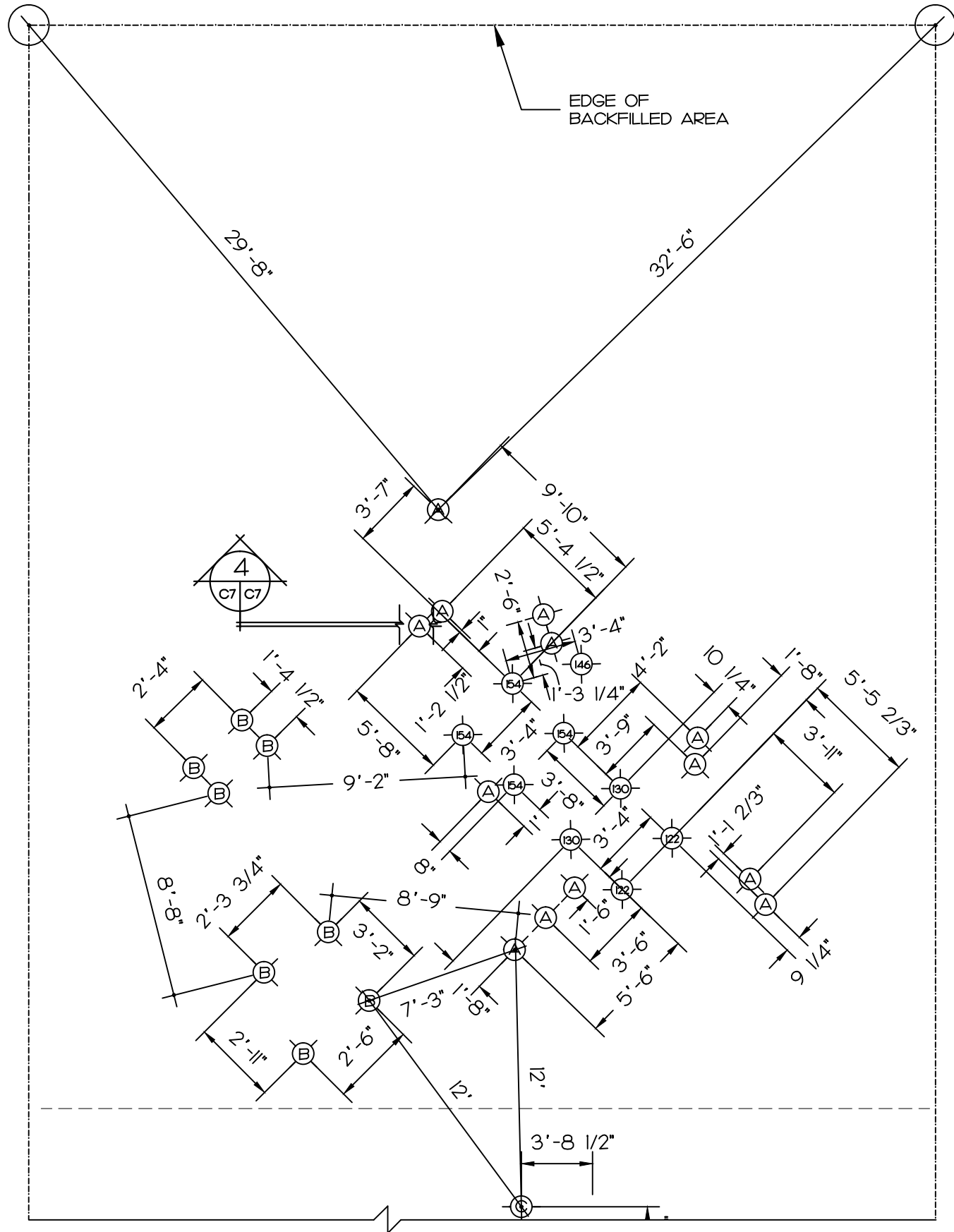
FOOTING LOCATIONS - NORTH SECTION
