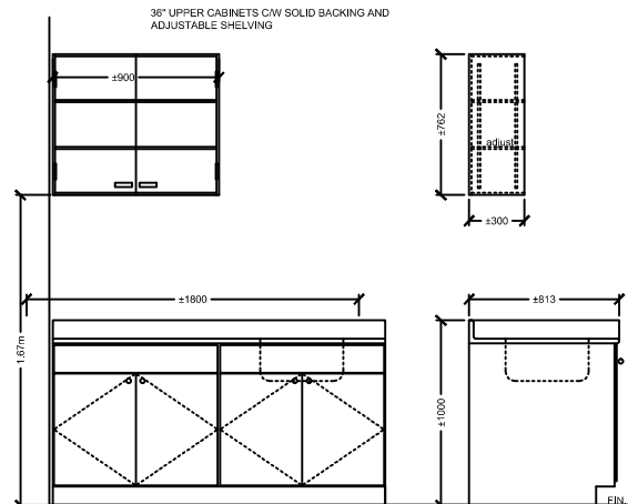
5 SAMPLING COUNTER 302 SCALE: 1:20
