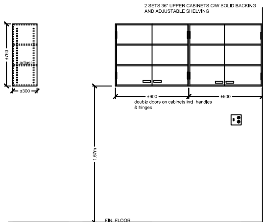
6 DESK / WORKSTATION 302 SCALE: 1:20
