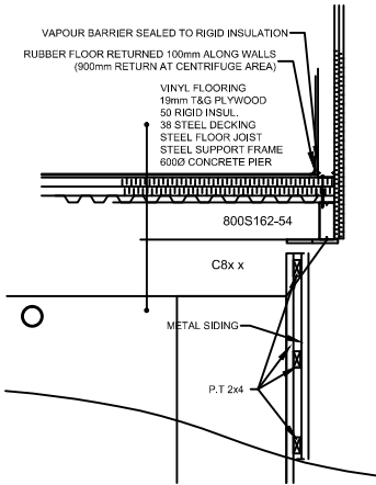
4 FLOOR DETAILS 302 SCALE: 1:20
