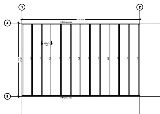
6 ROOF FRAMING 301 SCALE: 1:20
