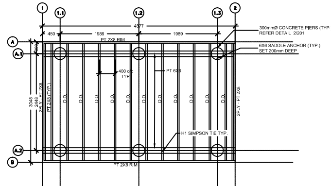
7 FLOOR FRAMING 301 SCALE: 1:20
