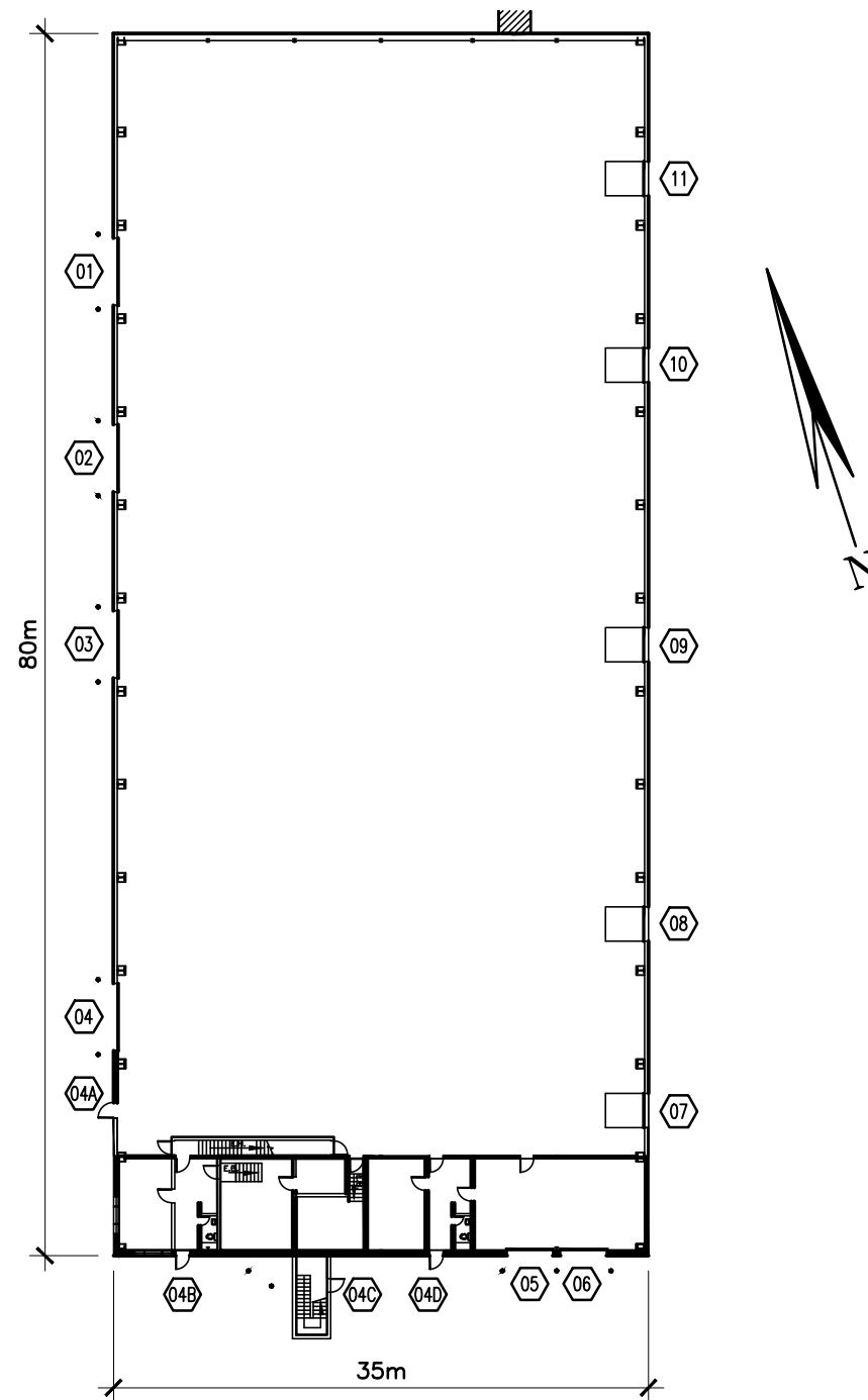
PLAN AGRANDI #2 (RDC)
