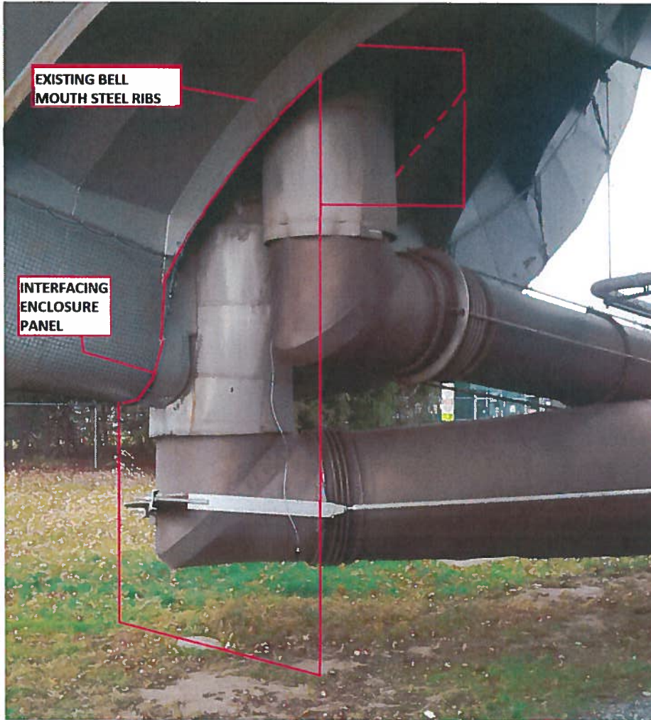
Figure 4. Enclosure / Wind Tunnel Interfacing.
