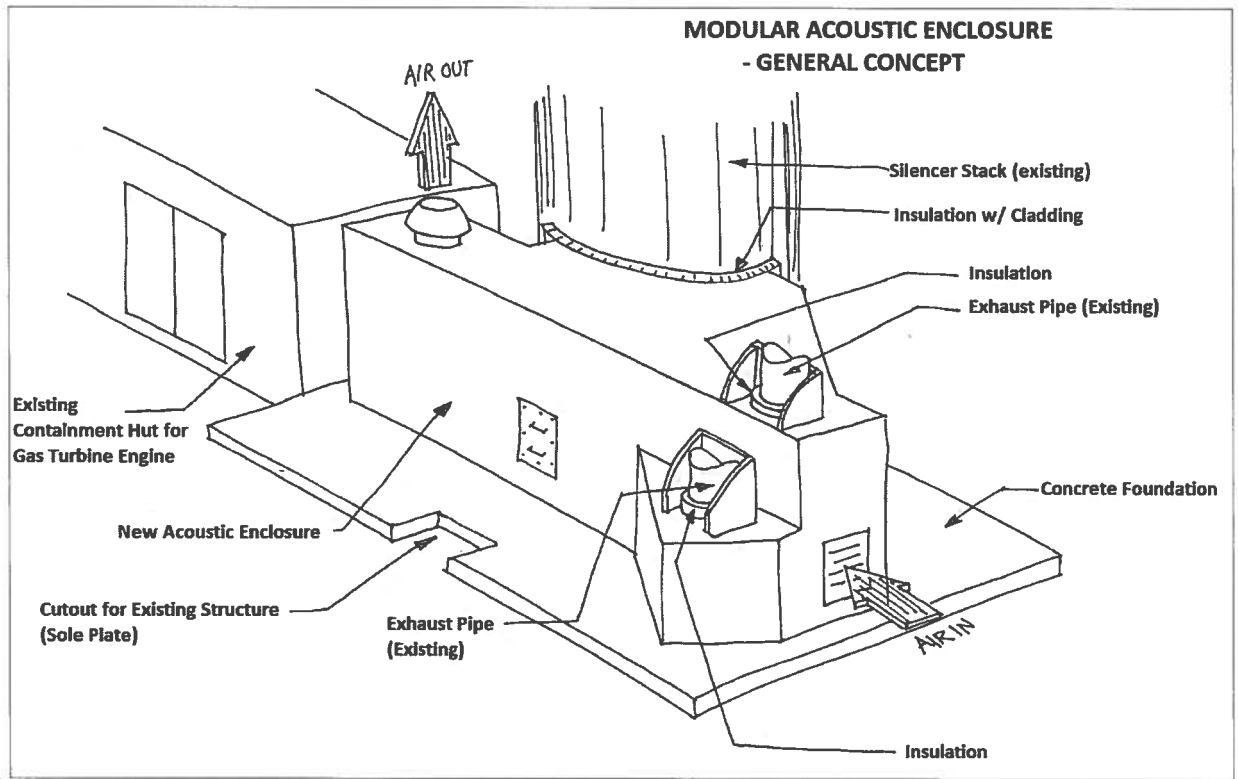
Figure 3 – Enclosure Concept Sketch.
