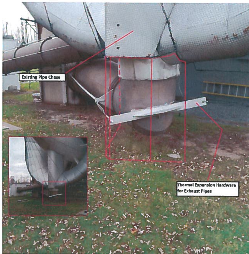
Figure 5. Portion of Enclosure under pipe chase.
