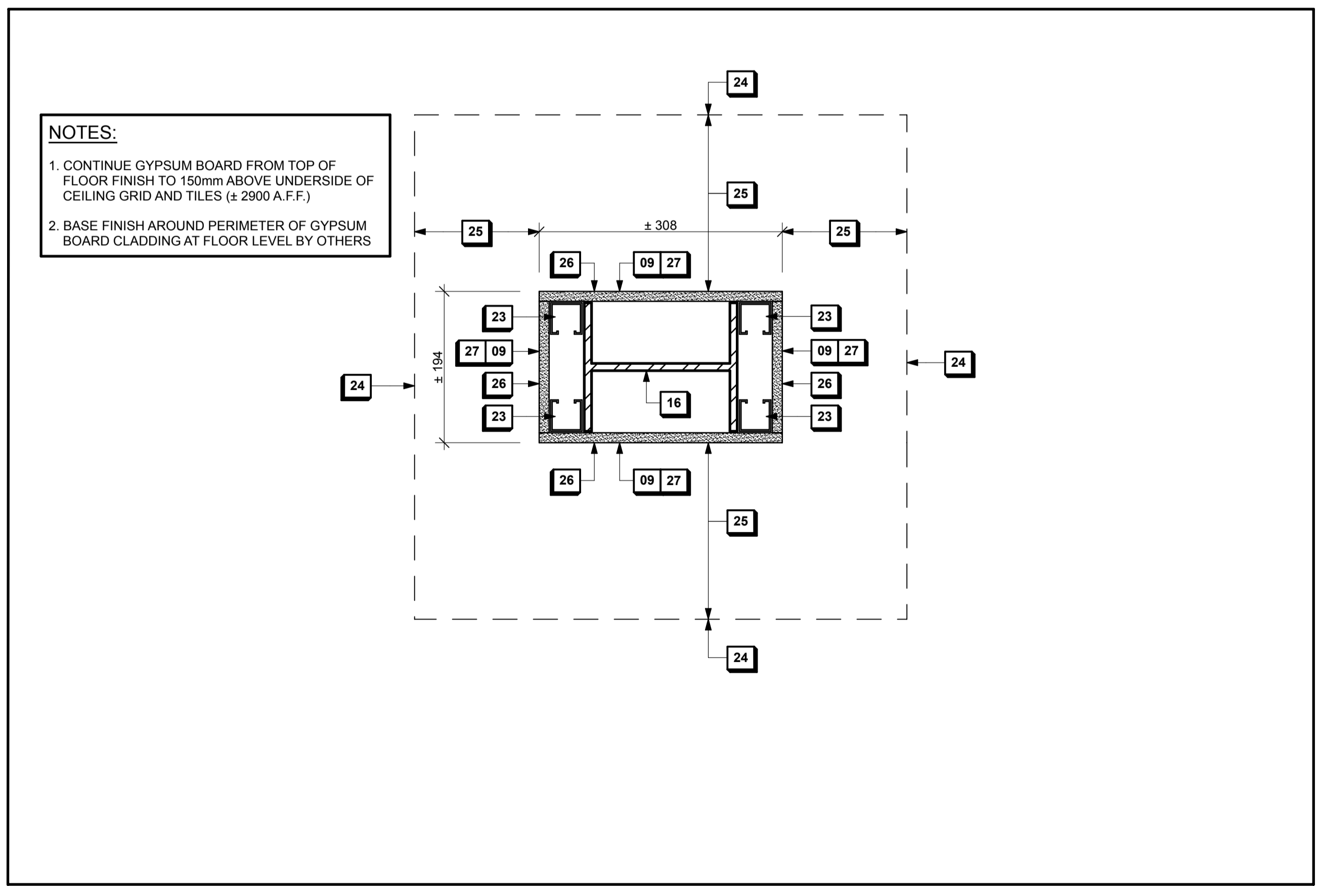
2 A03 NEW COLUMN FINISH - PLAN DETAIL SCALE: 1:5
