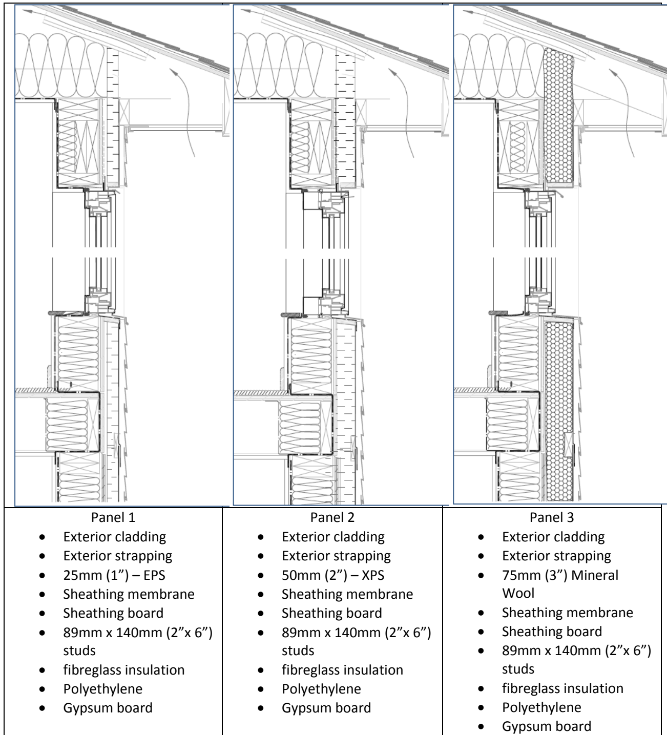
Figure 1 – Exterior Insulated Wall Assemblies
