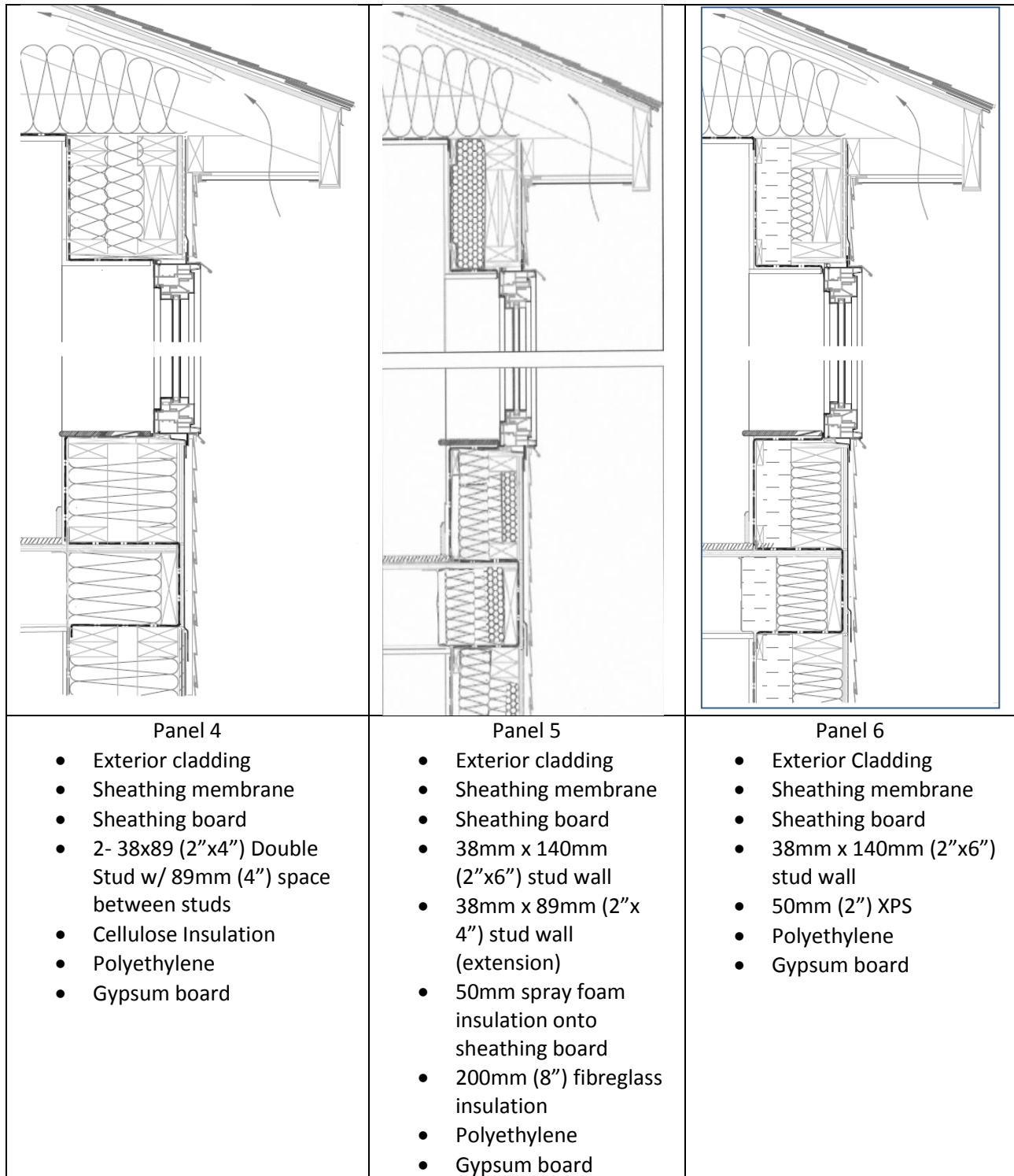
Figure 2 – Interior Insulated Wall Assemblies
