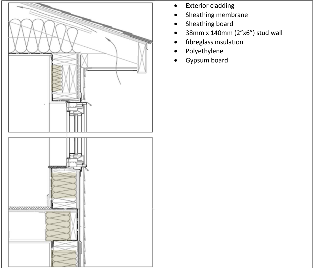
Figure 3 – Reference Wall
