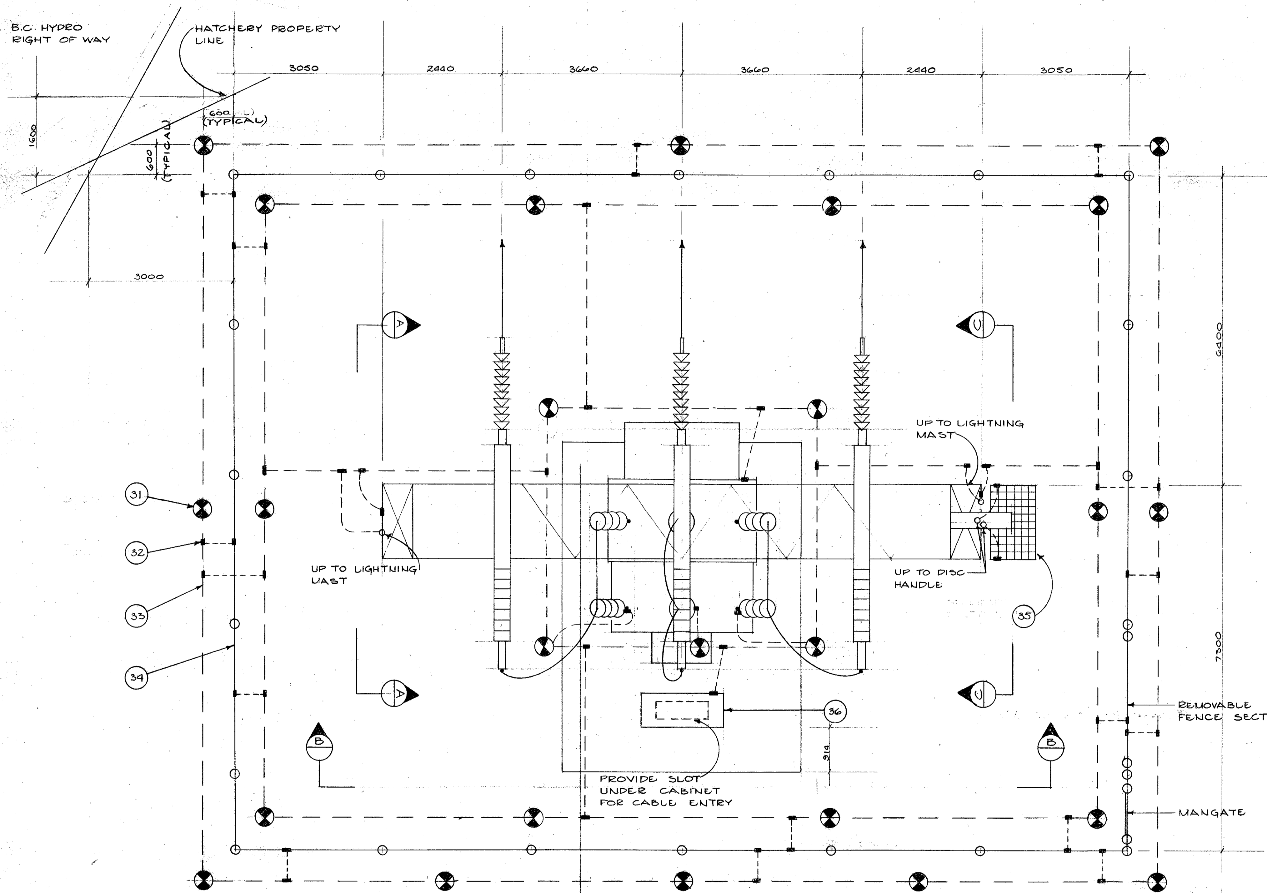
LAYOUT AND GROUNDING SCALE 1/4" = 1'-0"
