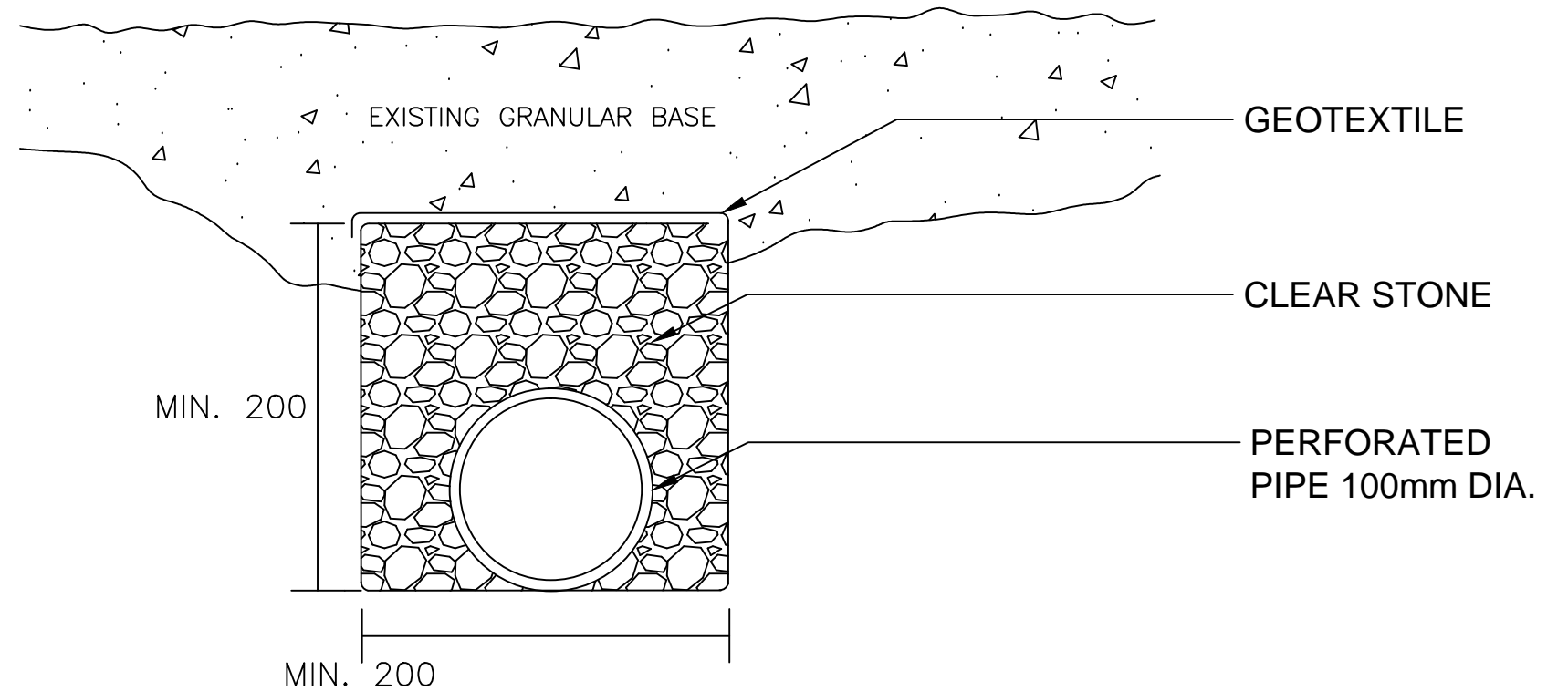
SUBSURFACE DRAIN DETAIL N.T.S.
