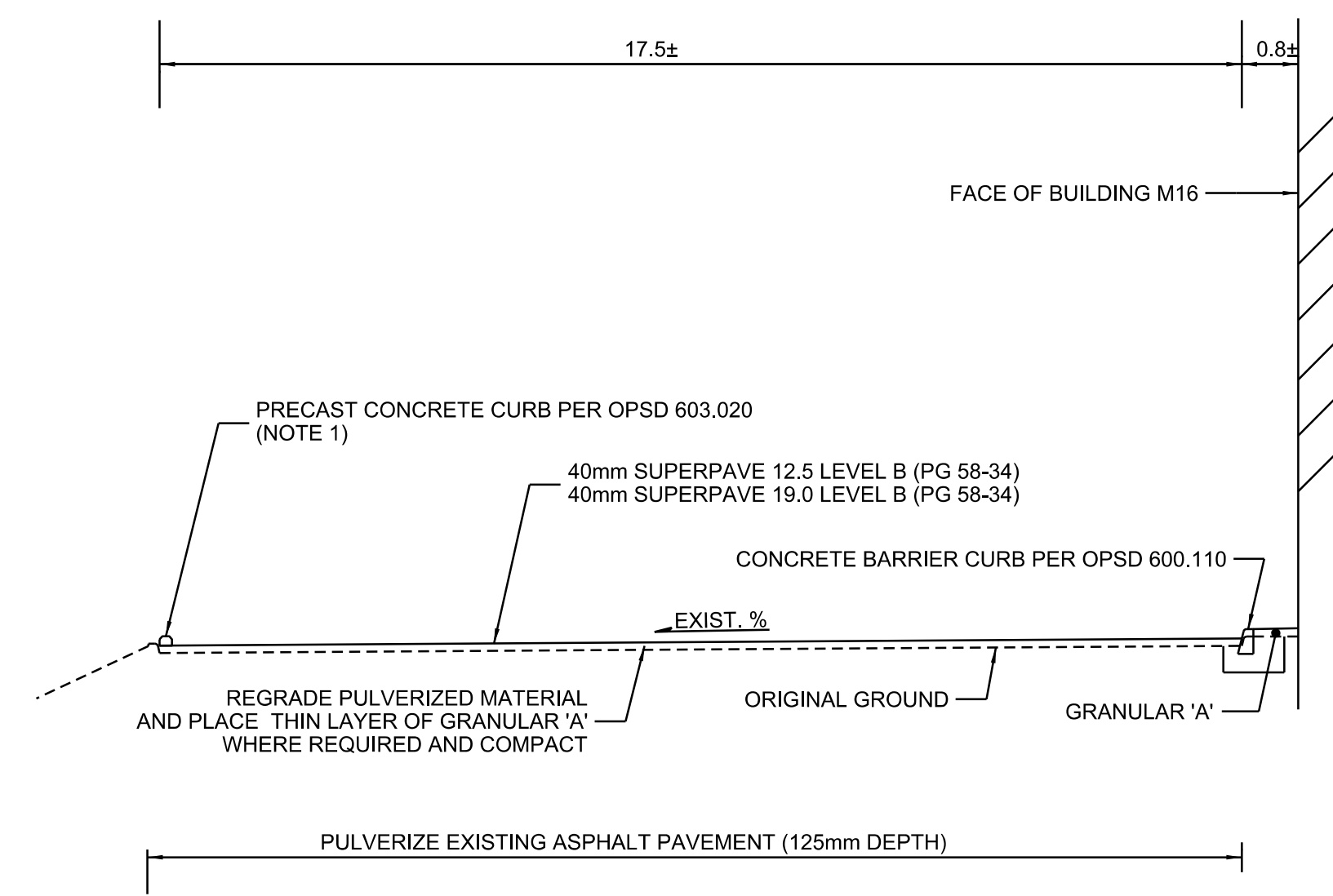
SECTION B-B
