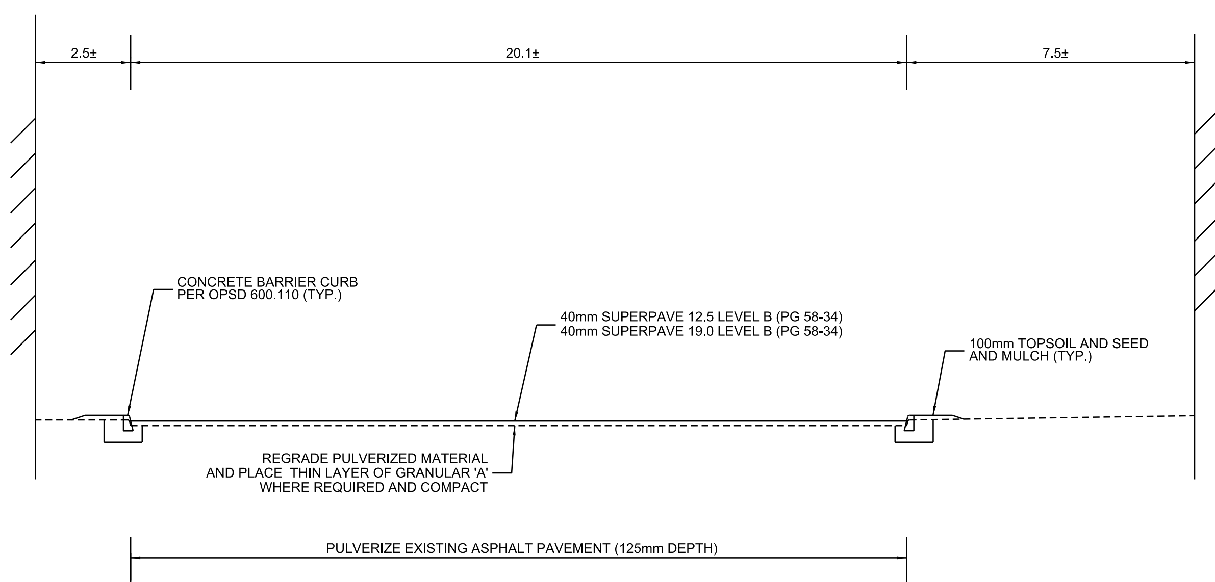
SECTION C-C
