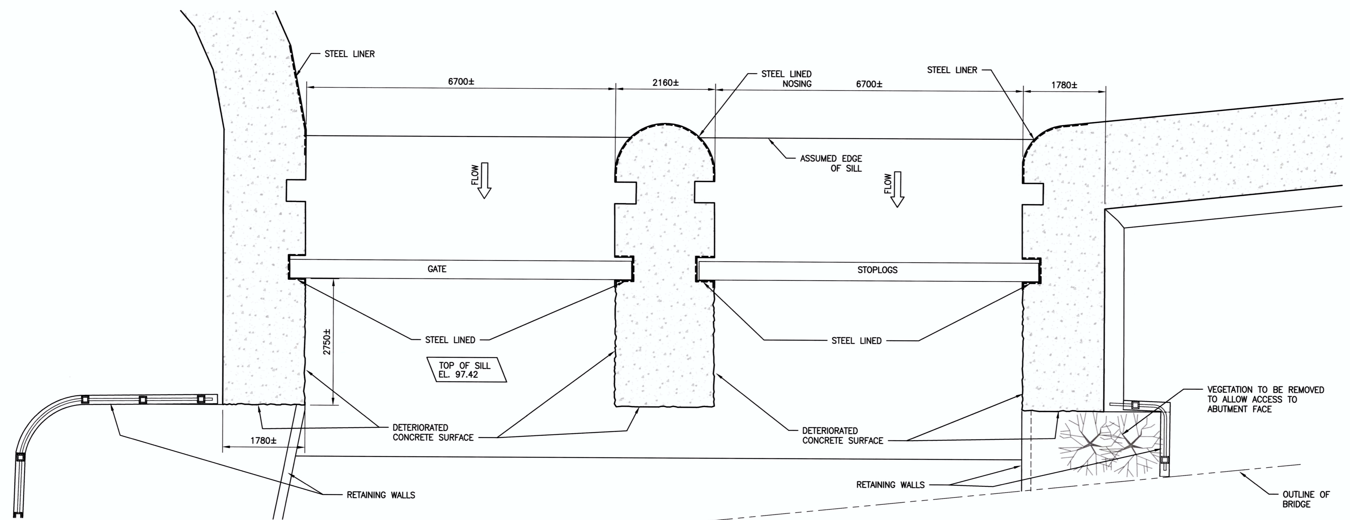
PLAN BELOW EL. 103.38 SCALE: 1:50
