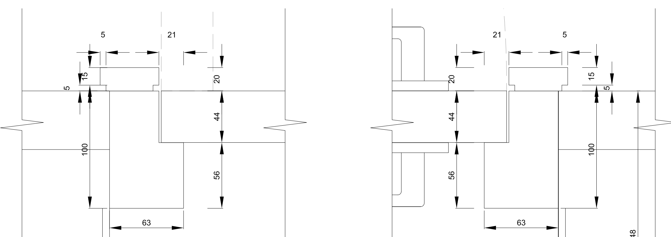
DETAIL 1 SCALE 1:2
