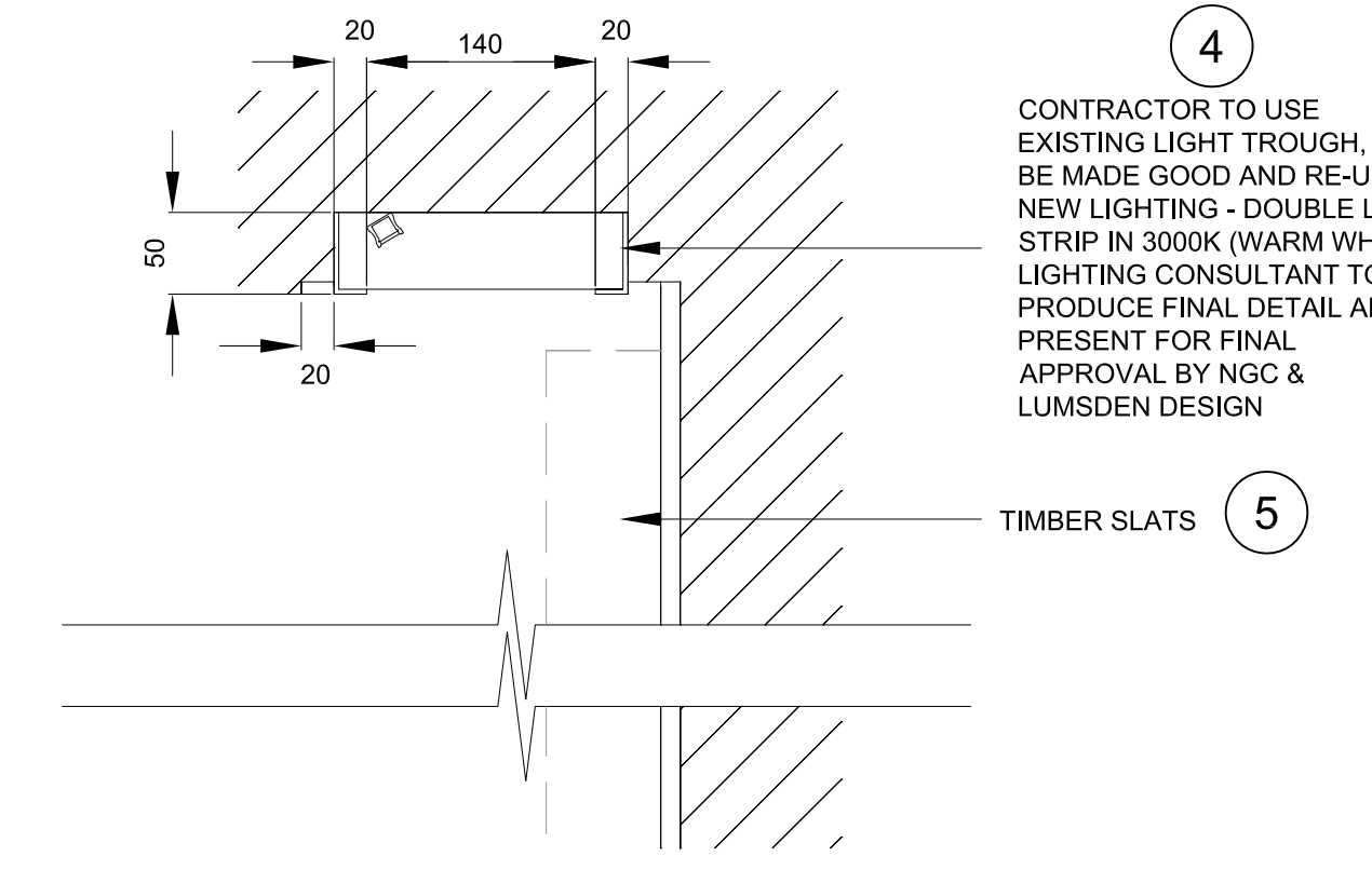
DETAIL 1 SCALE 1:5
