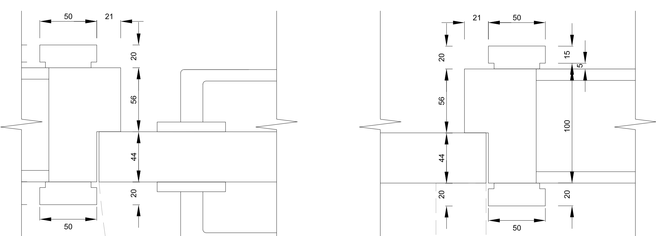
14 21 DETAIL 9 SCALE 1:2
