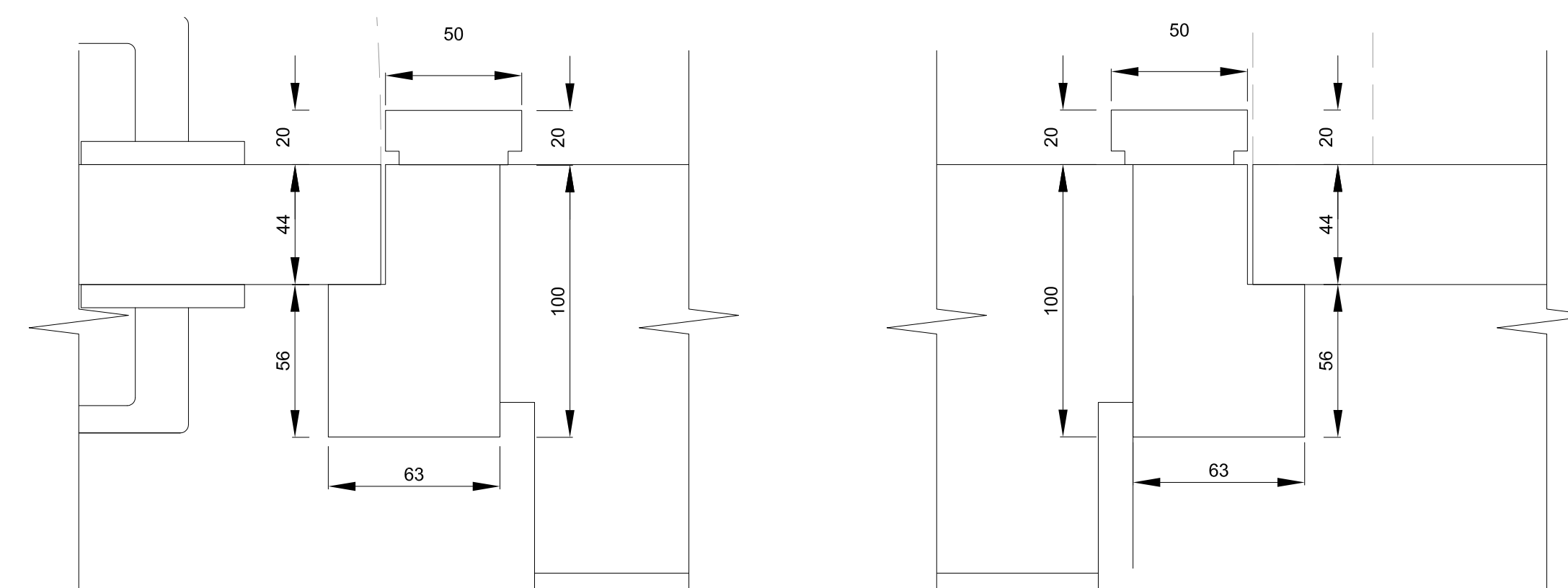
23 21 DETAIL 11 SCALE 1:2
