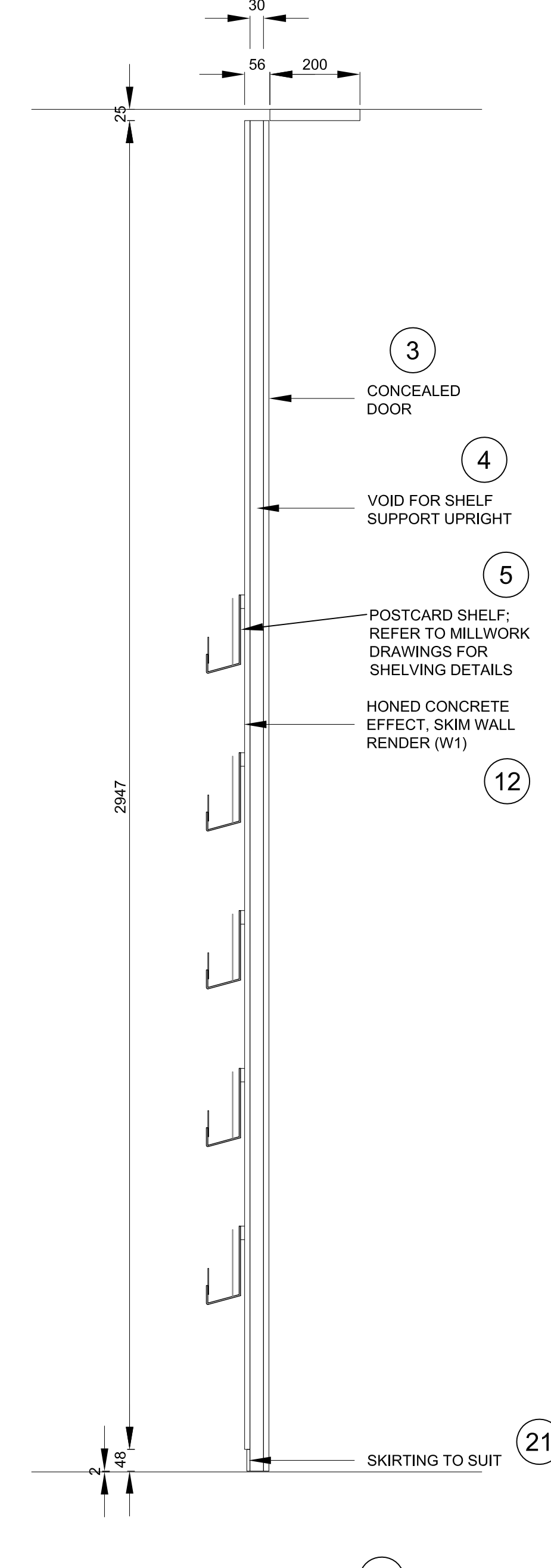
SECTION BB
