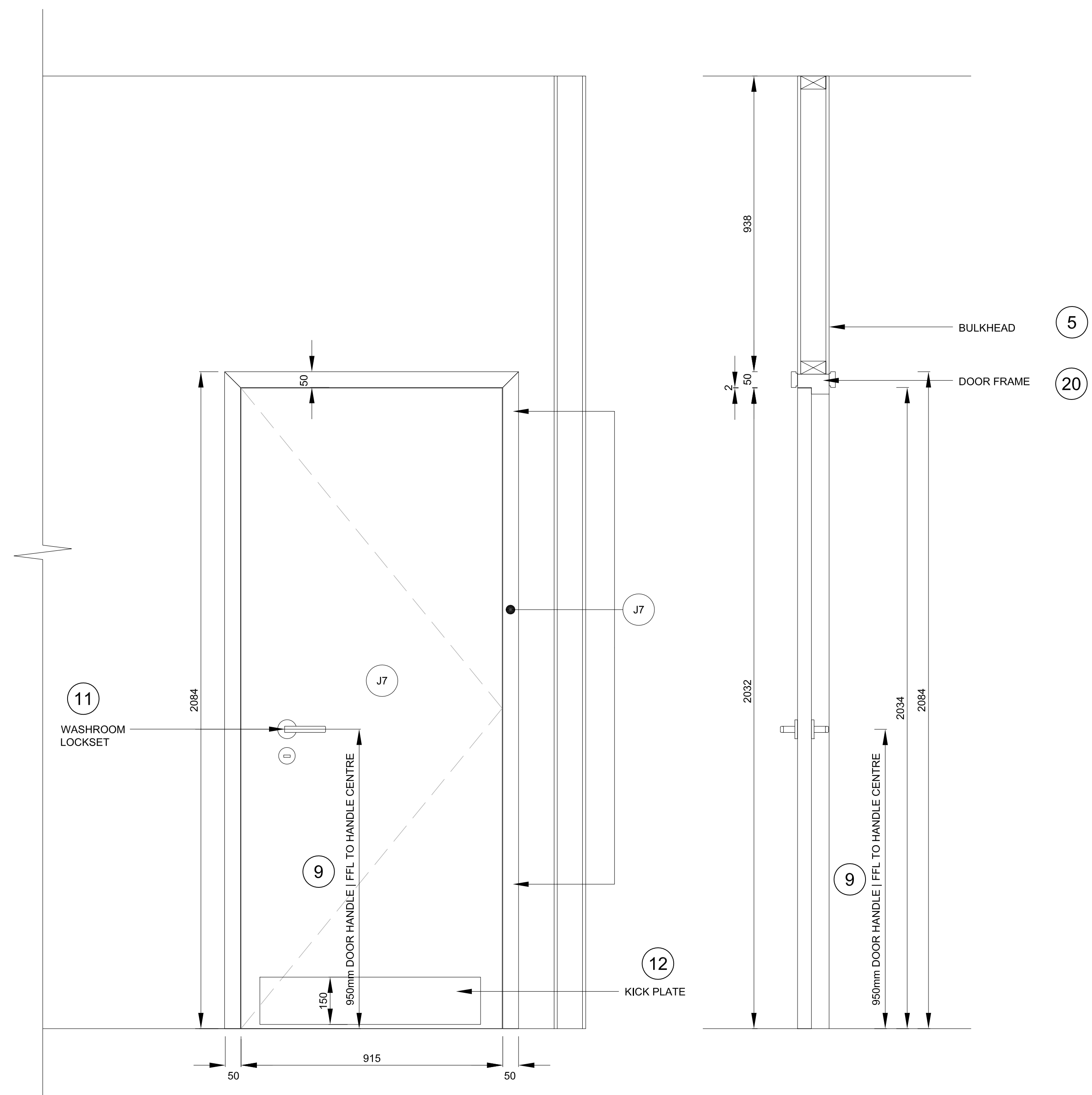
FRONT ELEVATION I
