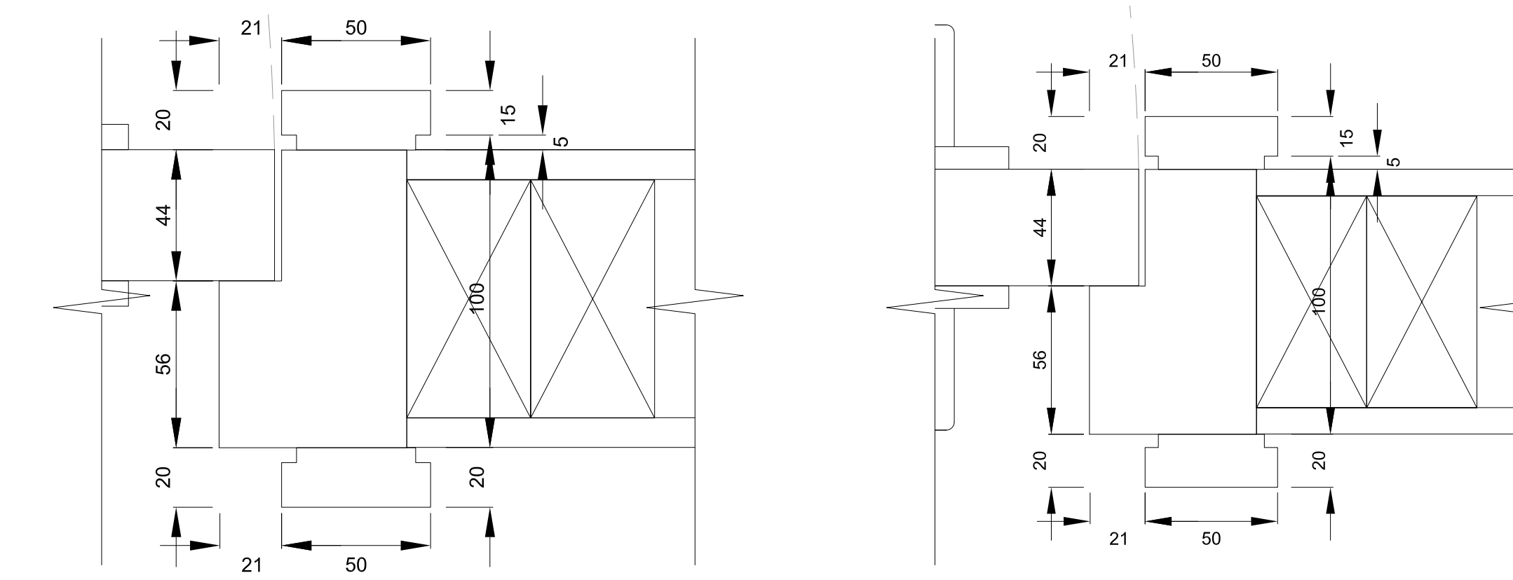
DETAIL 3 SCALE 1:2
