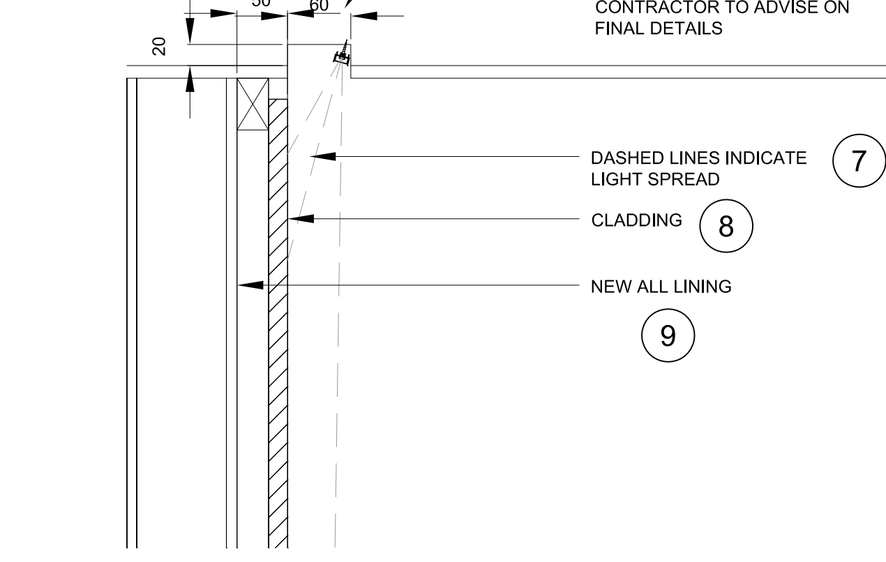
DETAIL 2 SCALE 1:5
