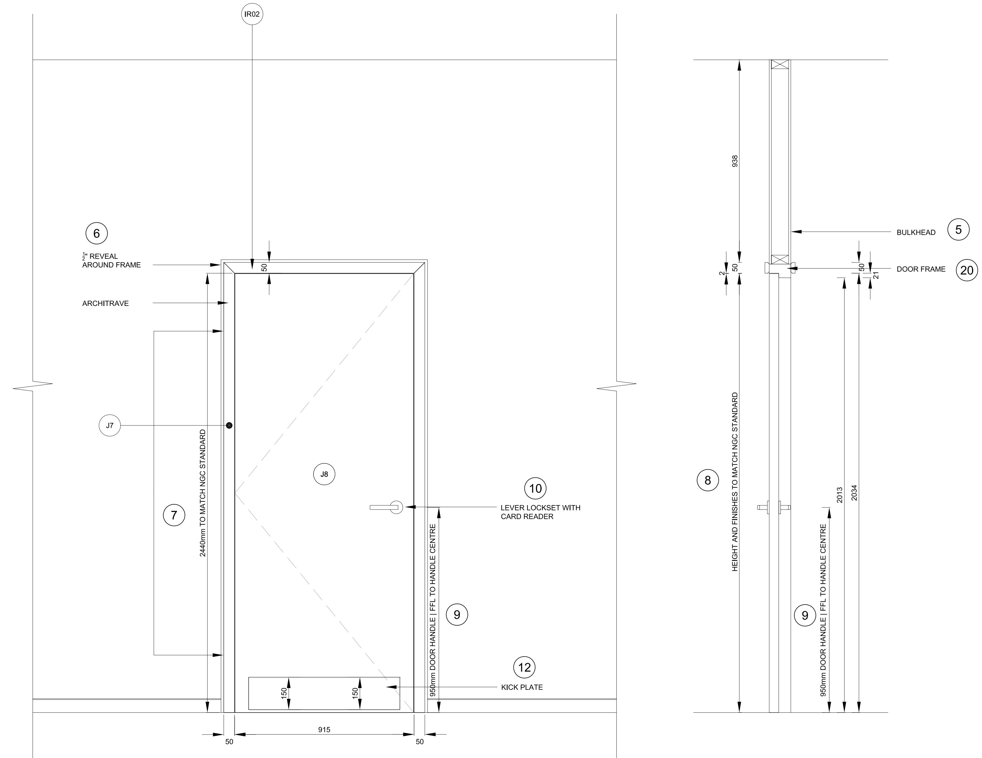
FRONT ELEVATION K
