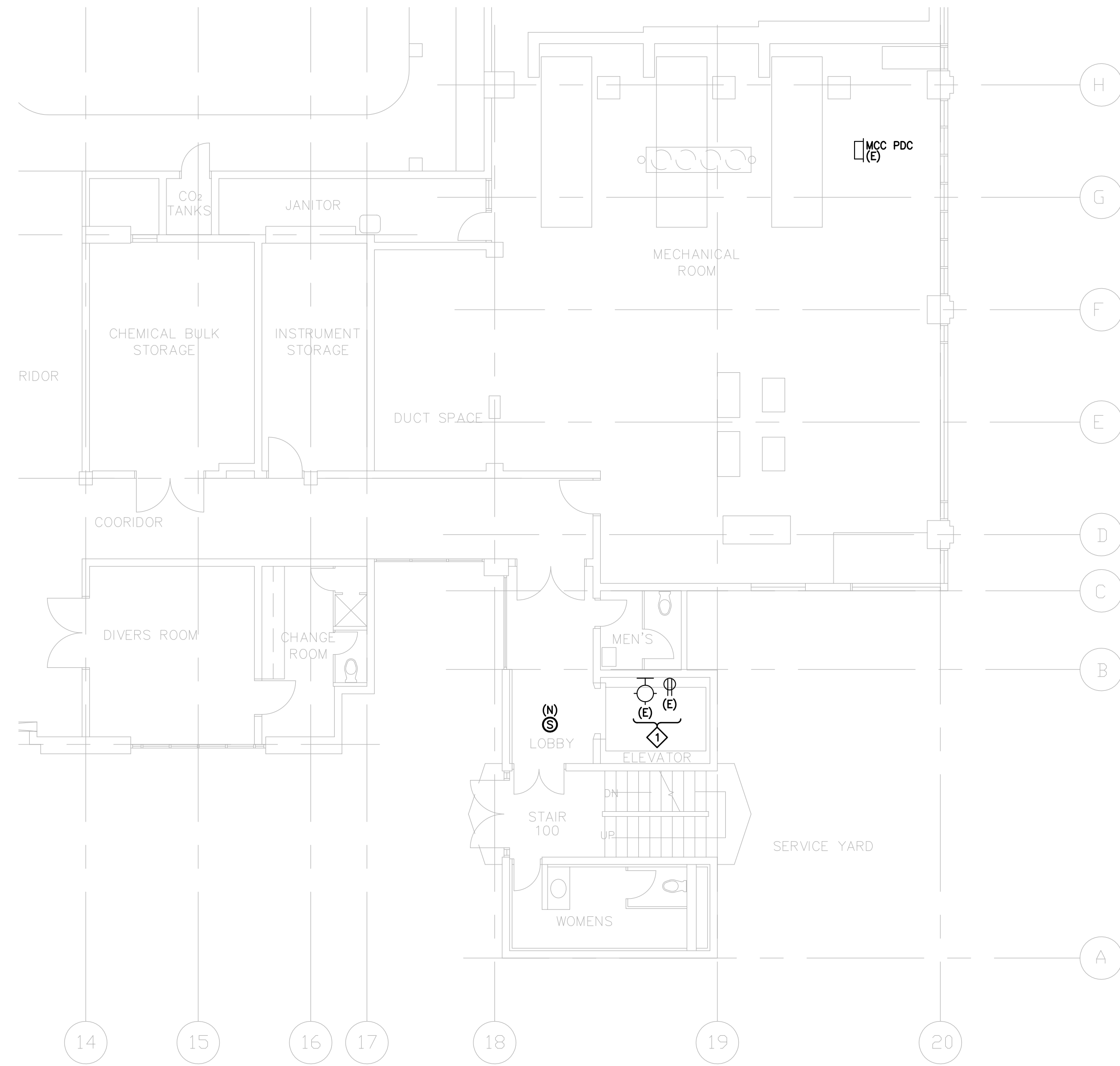
WAREHOUSE & SERVICE FLOOR PLAN
