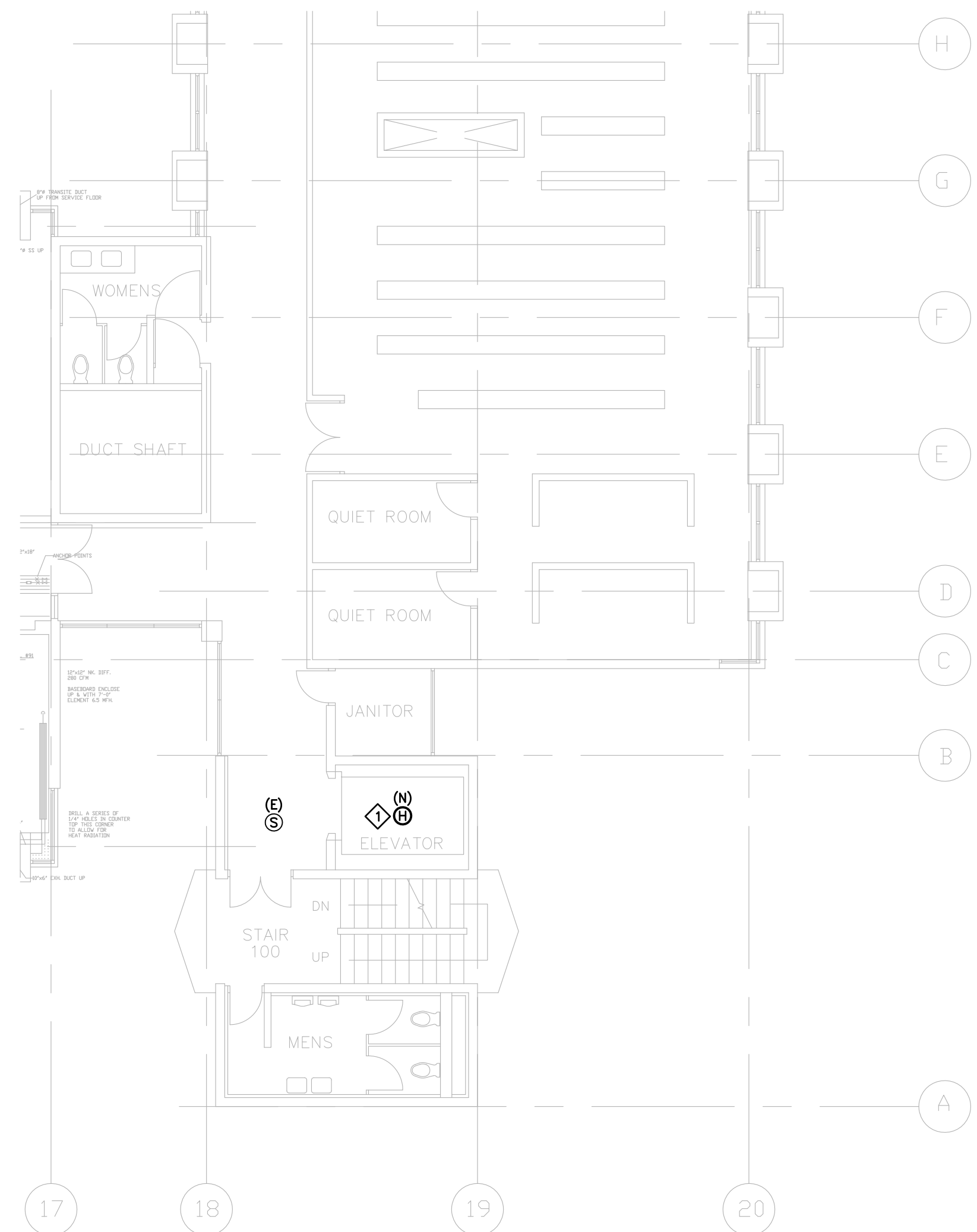
THIRD FLOOR PLAN SCALE: 1:100
