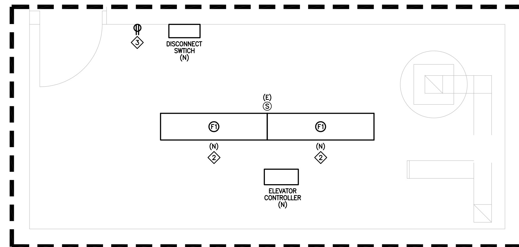
B CONTROL ROOM ENLARGEMENT SCALE: 1:25
