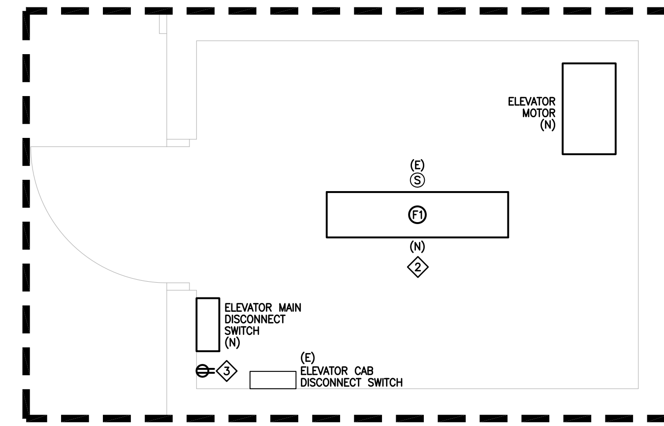
A MECHANICAL ROOM ENLARGEMENT SCALE: 1:25
