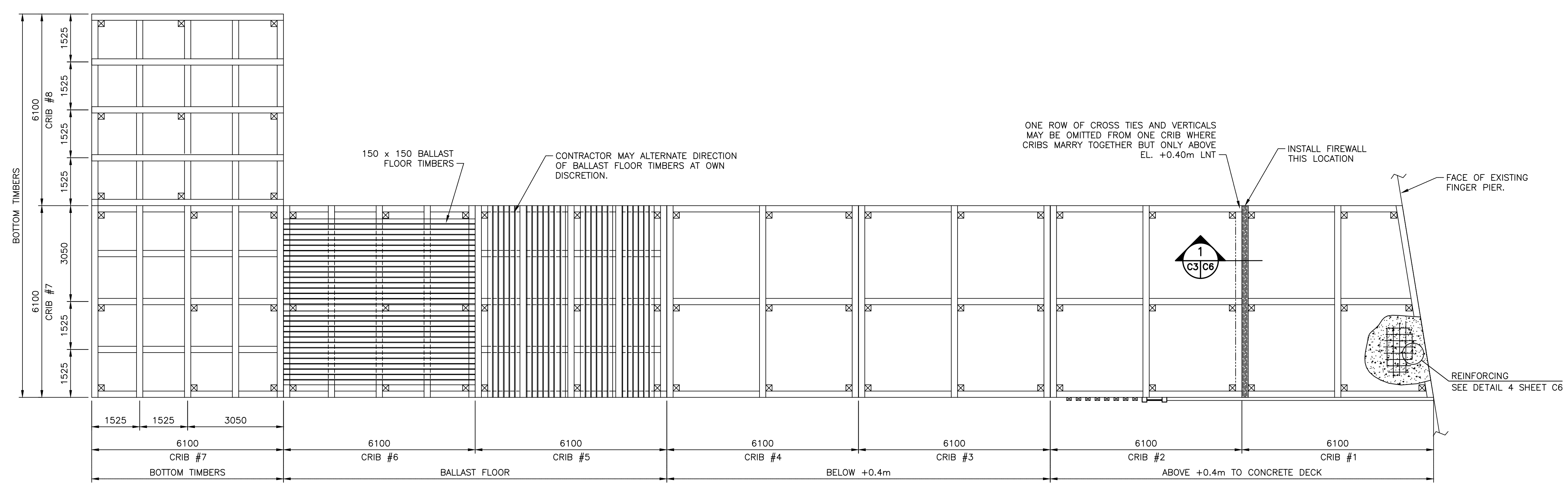
WHARF CONSTRUCTION PLAN SCALE : 1:75
