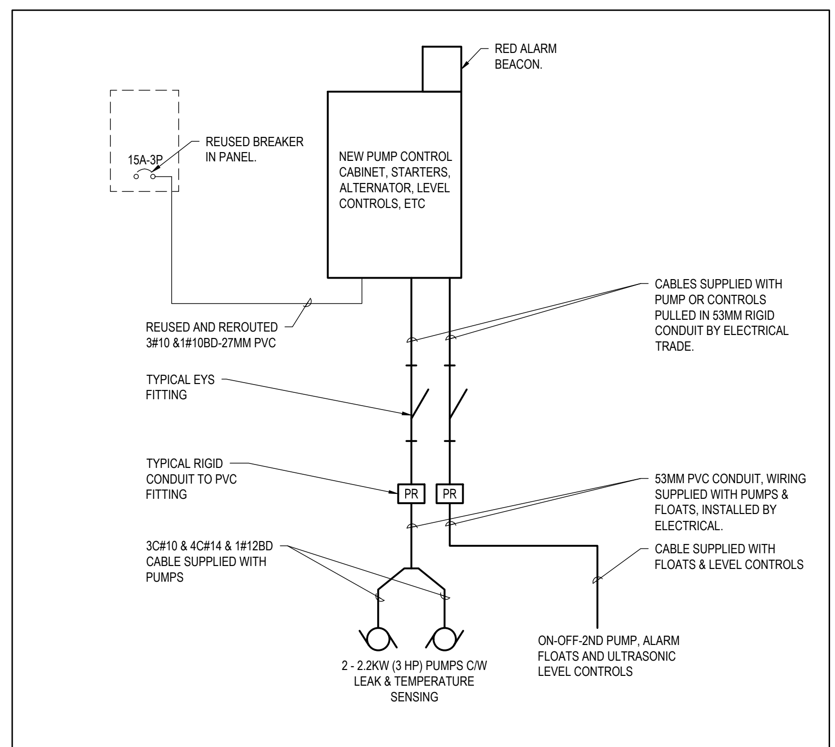
2 NEW PUMP CONTROLS SCALE: NTS
