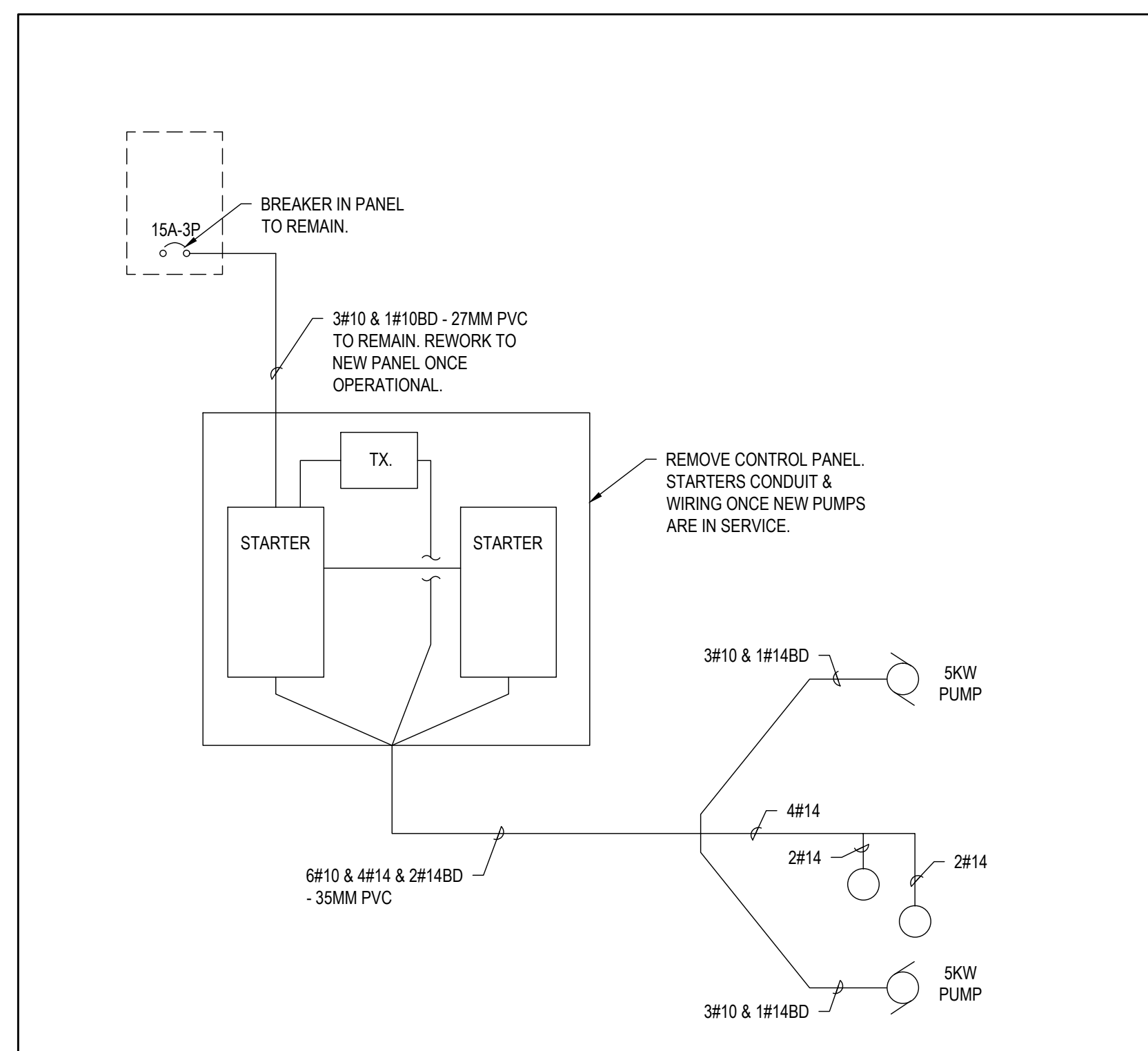
1 EXISTING PUMP CONTROLS SCALE: NTS
