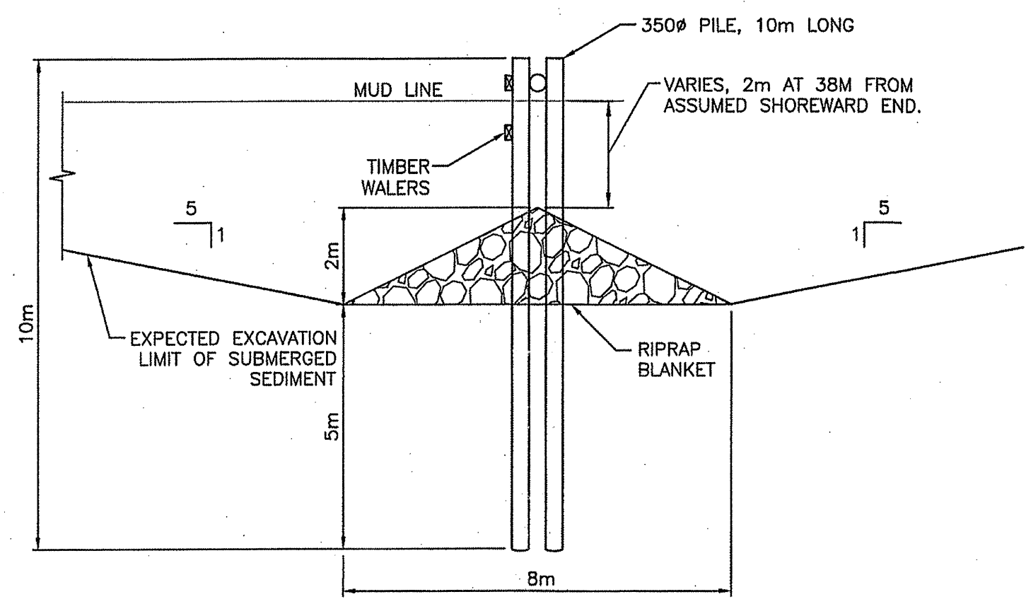
TYPICAL EXPECTED SECTION SCALE 1:100
