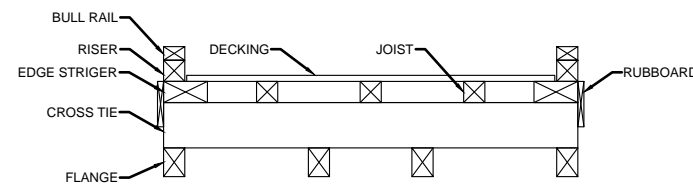
TYPICAL CROSS SECTION AND COMPONENTS FOR EXISTING FLOATS L & J SCALE 1:50
