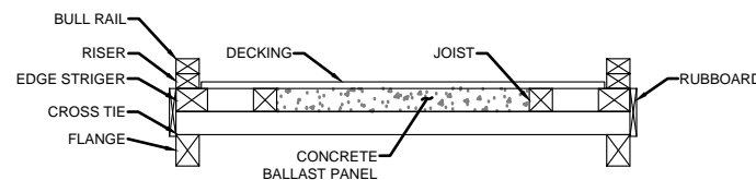
TYPICAL BALLASTED FLOAT CROSS SECTION FOR EXISTING FLOATS E & F SCALE 1:50
