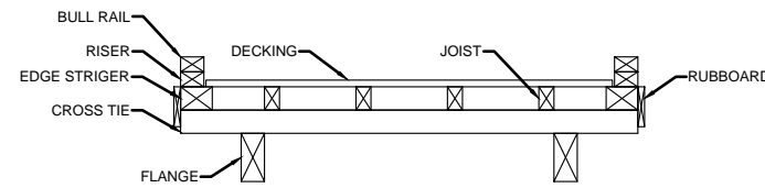
TYPICAL CROSS SECTION AND COMPONENTS FOR EXISTING FLOAT K SCALE 1:50
