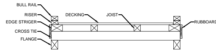
TYPICAL CROSS SECTION AND COMPONENTS FOR EXISTING FLOATS A, B, C & D SCALE 1:50
