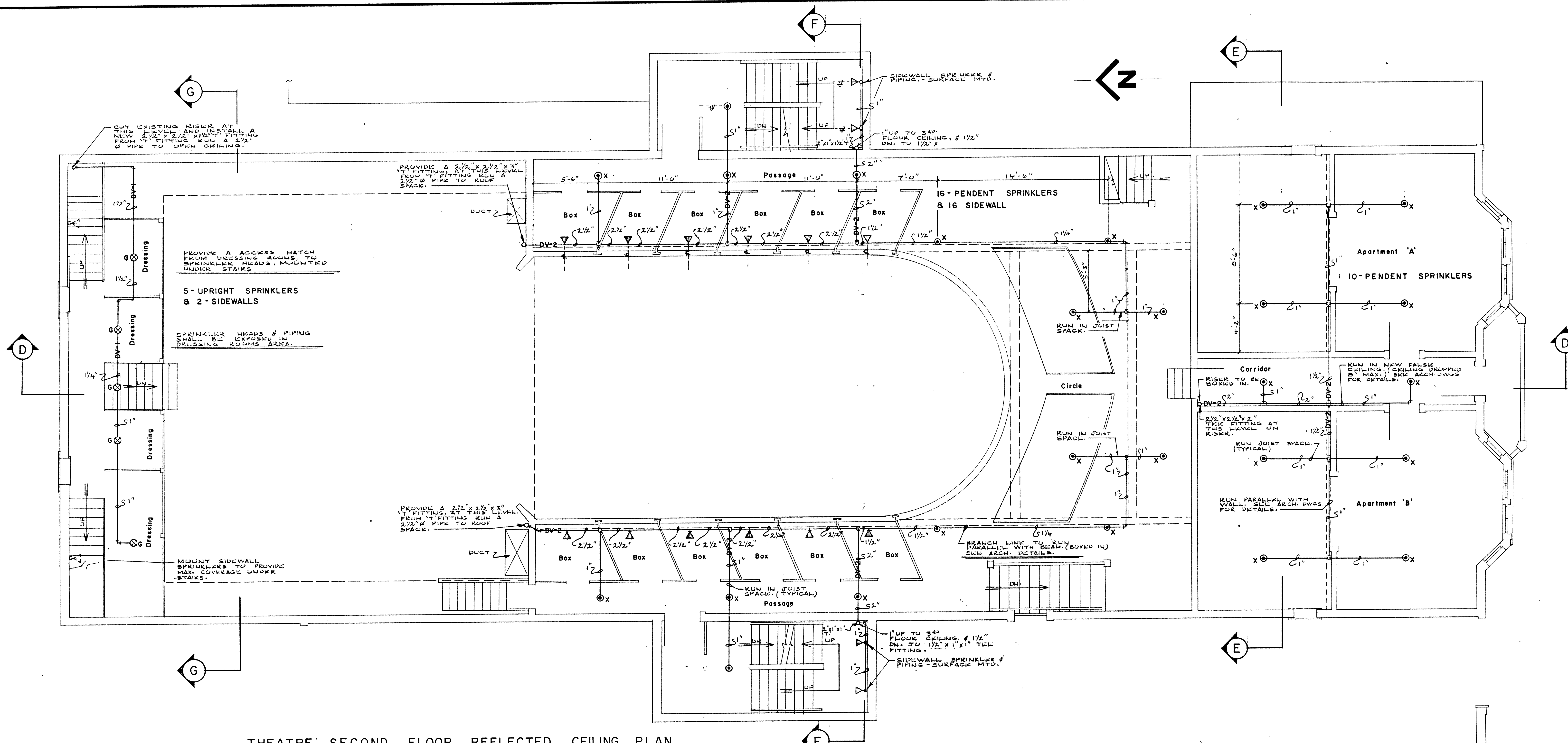
THEATRE: SECOND FLOOR REFLECTED CEILING PLAN SCALE: 1/4" = 1'-0"
