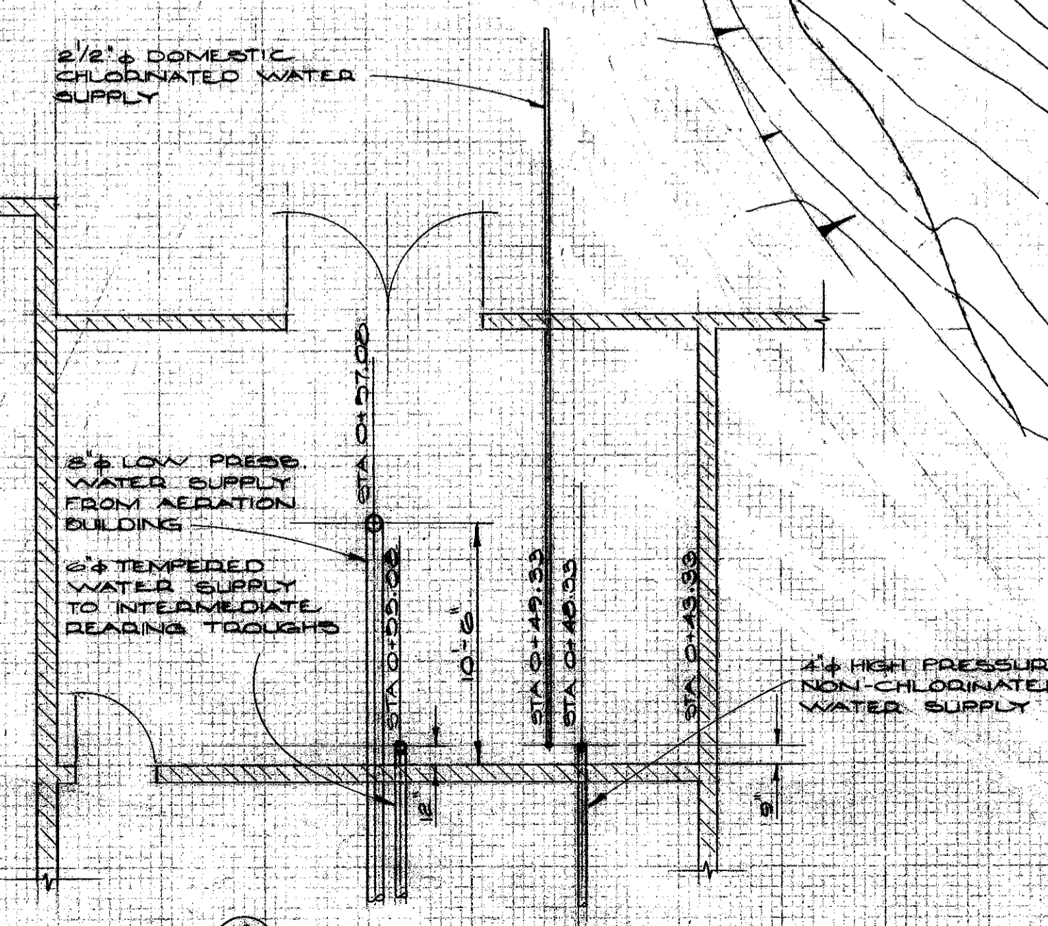
DETAIL B MECHANICAL ROOM PIPE LAYOUT SCALE: 3/16" = 1'-0"
