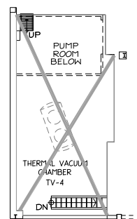
PLAN - MEZZANINE LEVEL - ELEV. 71.51m
