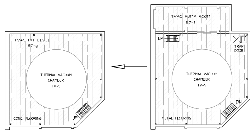
PLAN - PIT LEVEL LEVEL - ELEV. 61.42m
