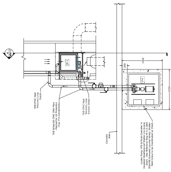
Detail: Pump Shelter Location 1-25
