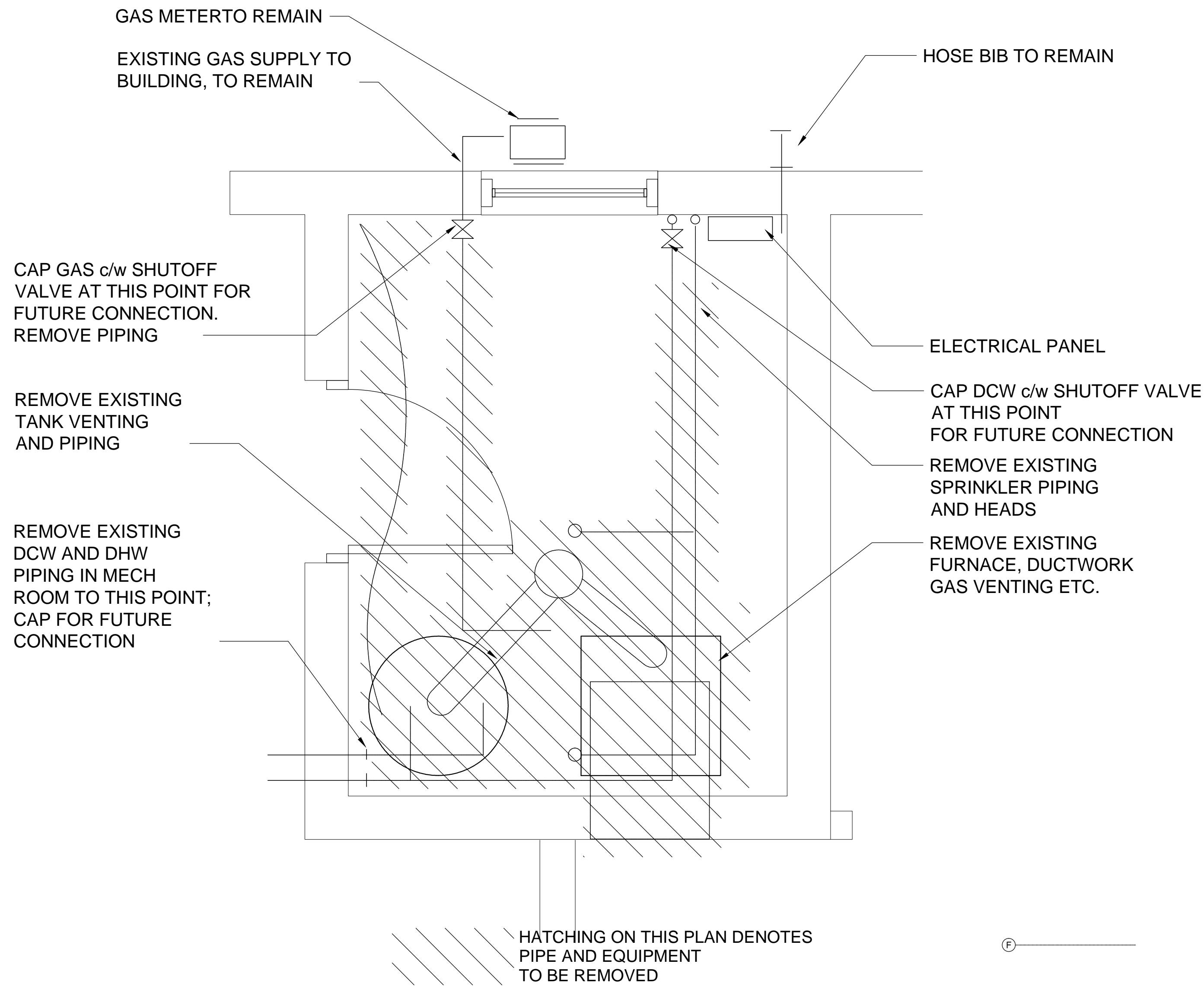
DEMOLITION PLAN - MECHANICAL ROOM SCALE 1:15
