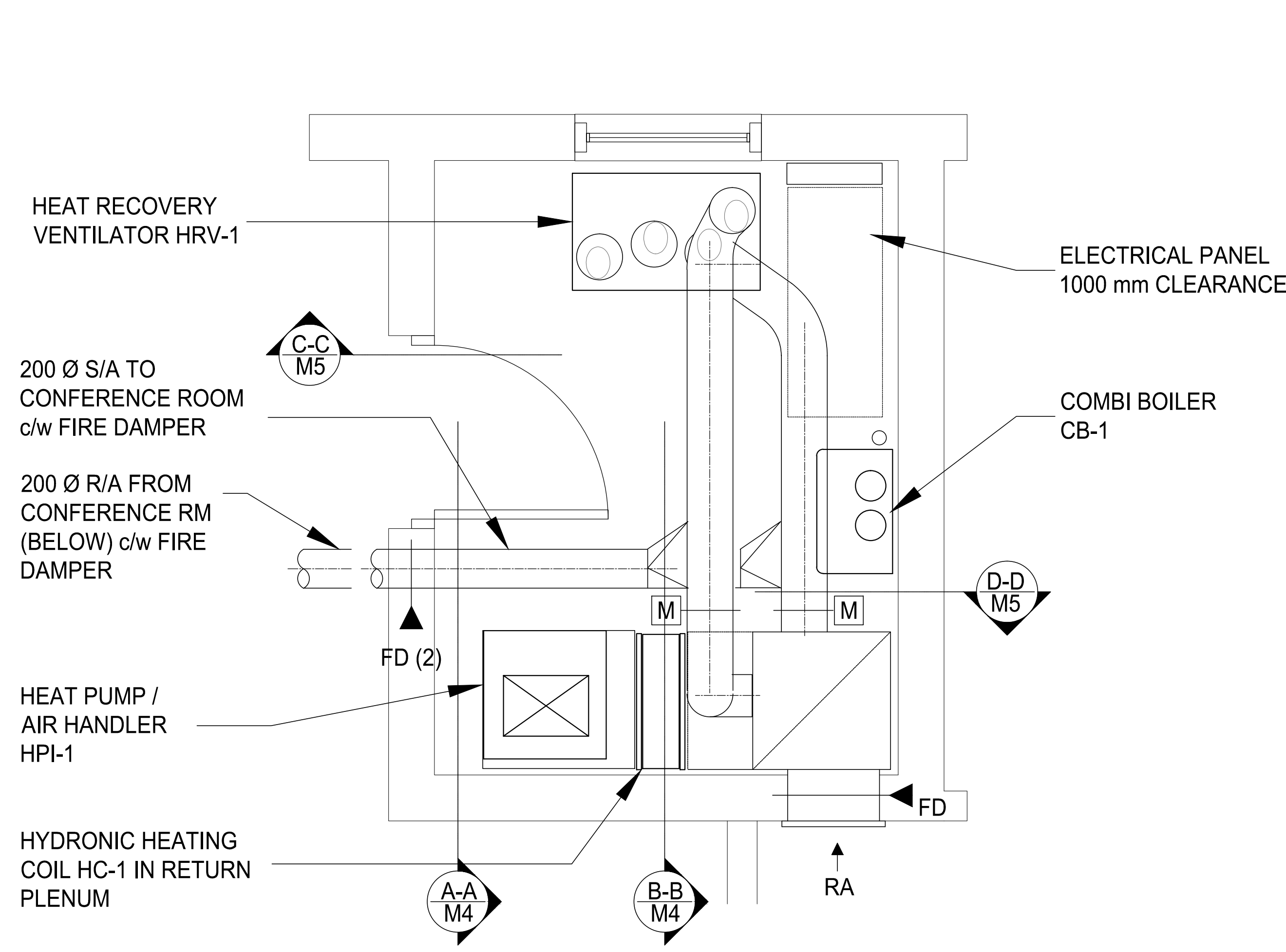
MECHANICAL ROOM PLAN AT 2200 AFF SCALE 1:16
