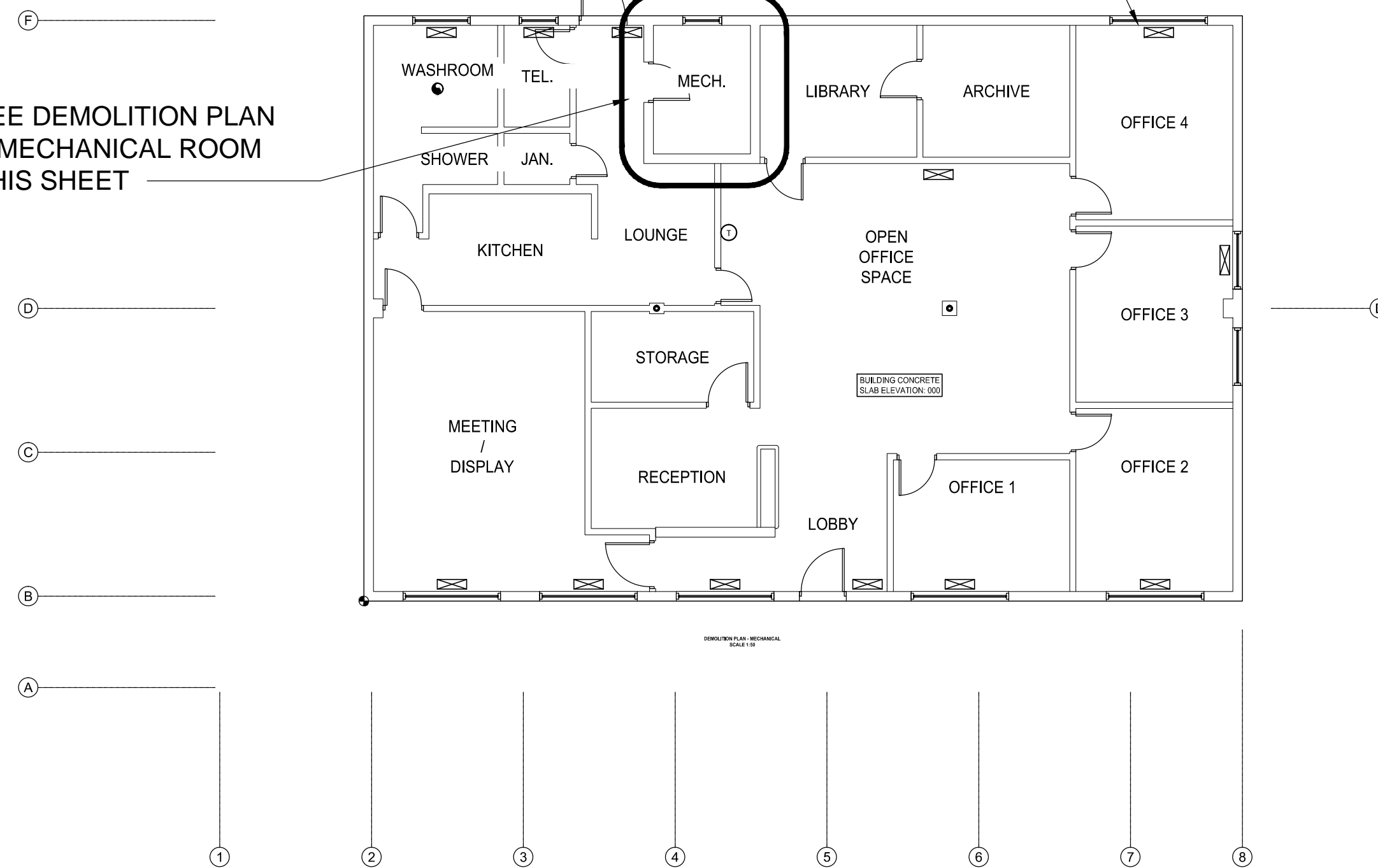
DEMOLITION PLAN
