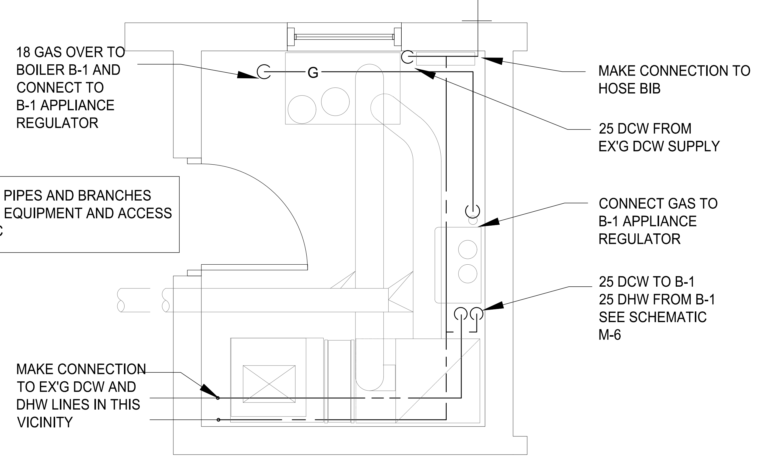
MECHANICAL ROOM PLAN - PLUMBING SCALE 1:16
