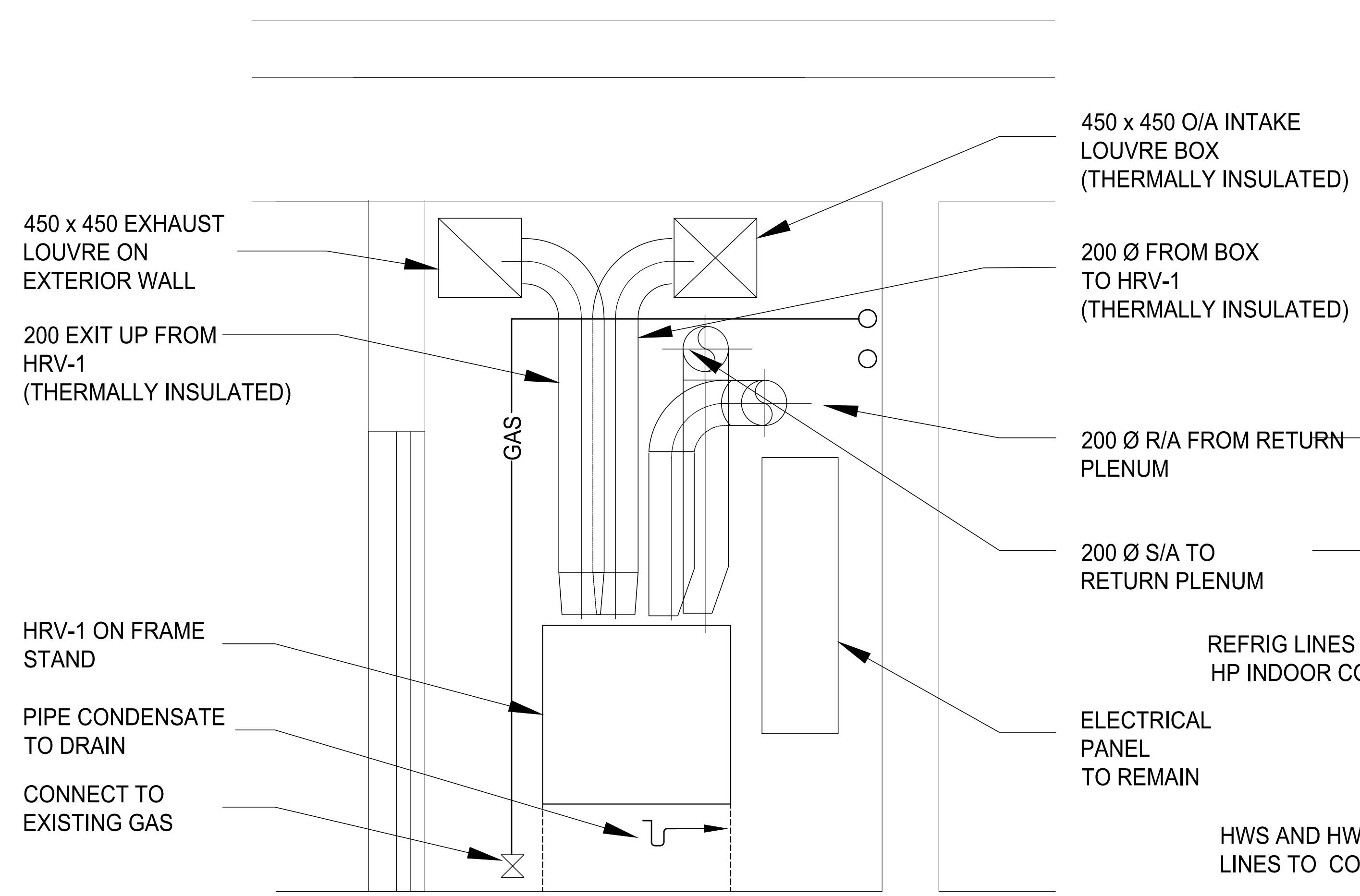
C-C MECHANICAL ROOM SECTION SCALE 1:16
