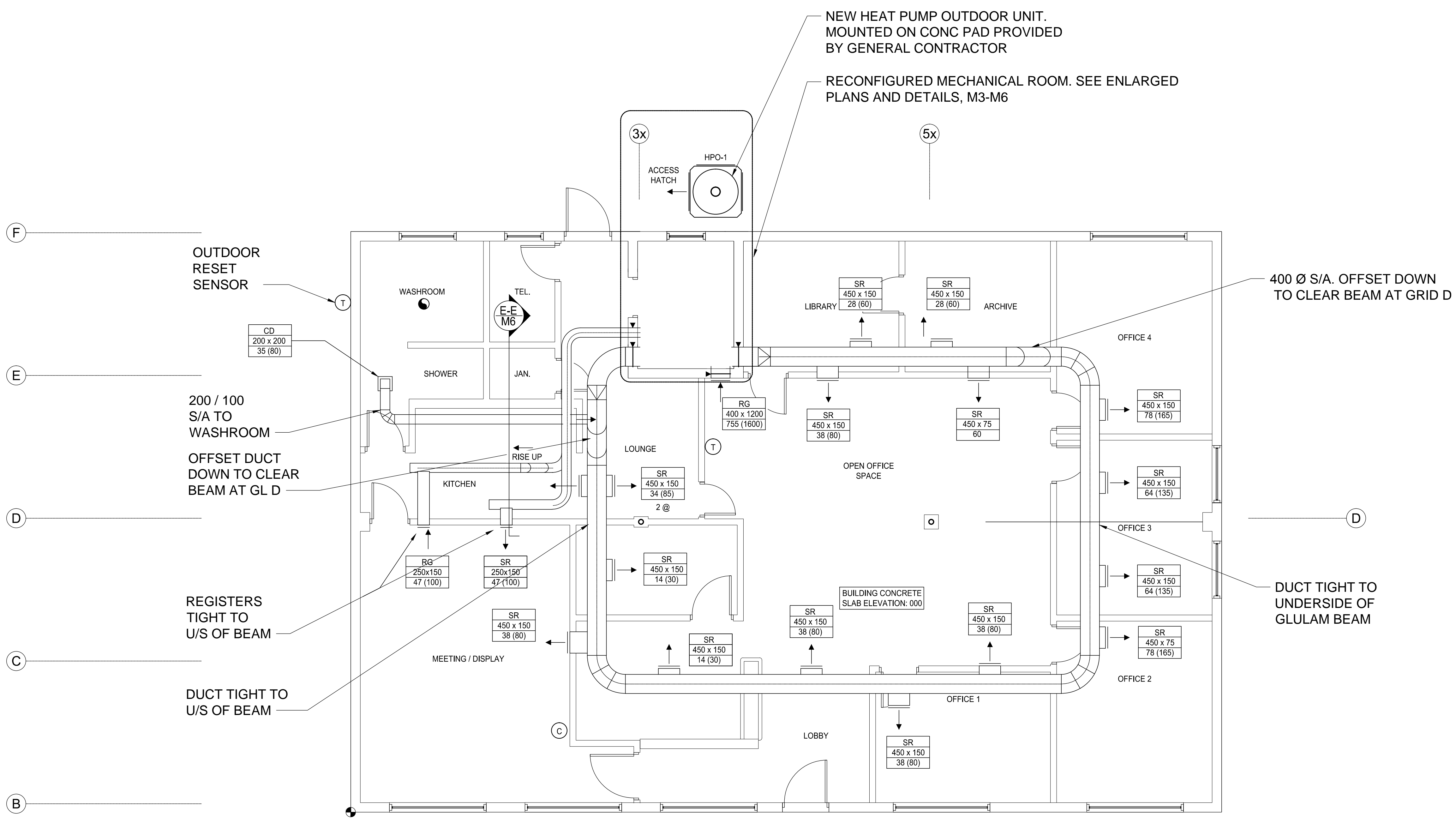
FLOOR PLAN - MECHANICAL SCALE 1:50
