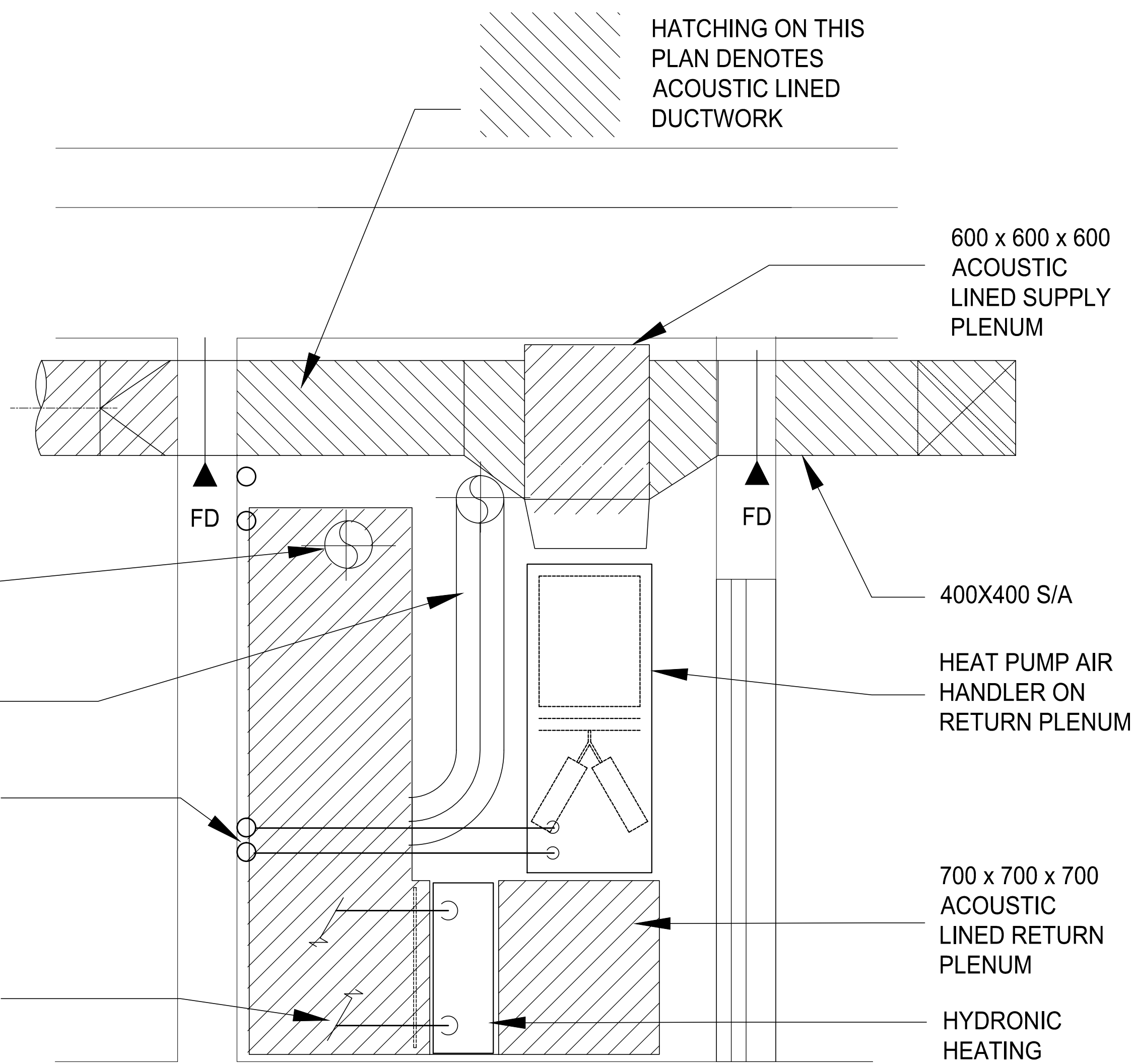
D-D MECHANICAL ROOM SECTION SCALE 1:16
