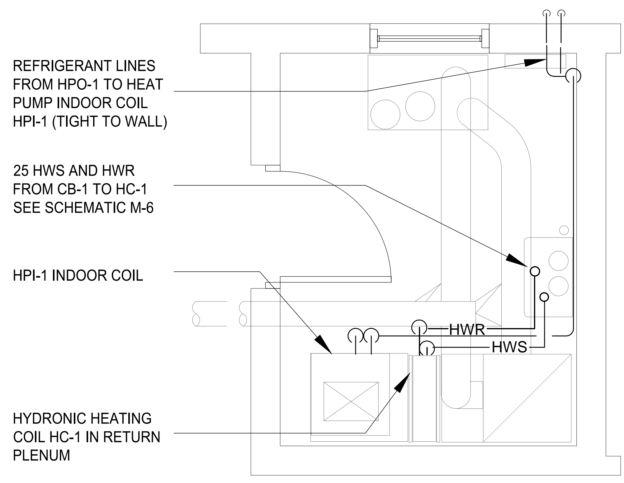
MECHANICAL ROOM PLAN - PIPING SCALE 1:16
