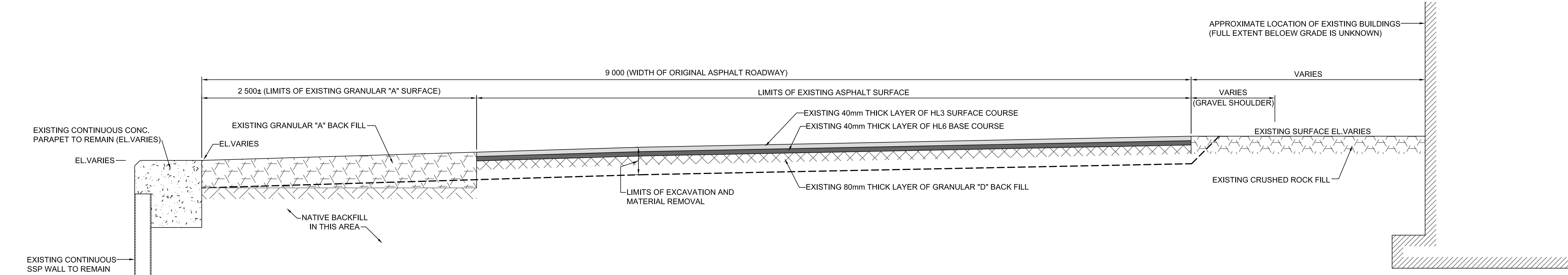
31 TYP. SECTION OF EXISTING PAVING CONDITIONS ALONG DOCK WALL SCALE: 1:20
