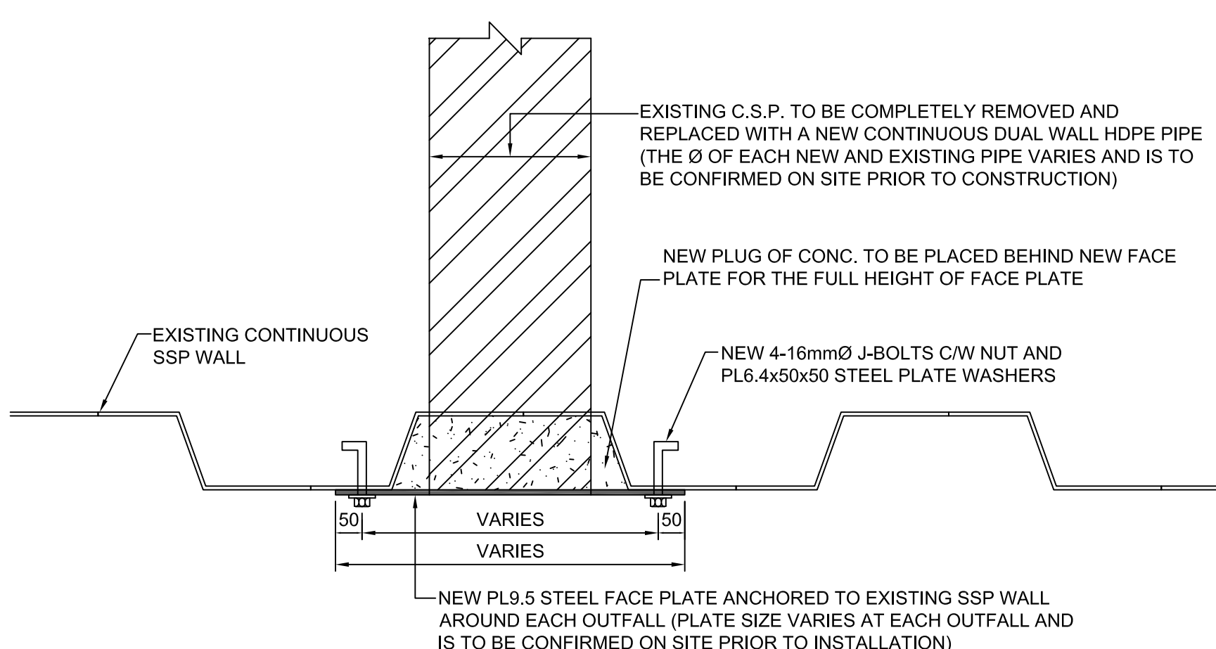
36 TYP. OUTFALL PIPE REPAIR PLAN DETAIL (FISHERMENS BASIN) SCALE: 1:10
