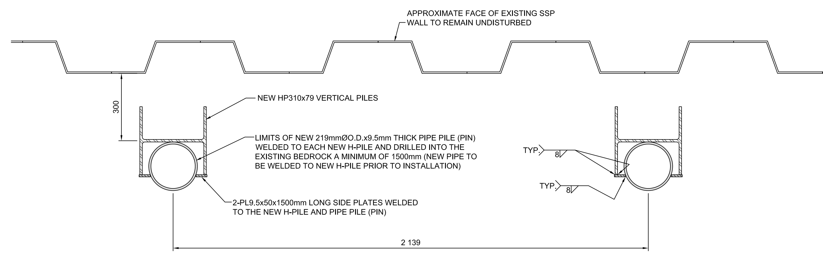
47 11/11 TYP. SECTION OF H-PILE PIN CONNECTION (JETTY 3 & 7) SCALE: 1:10
