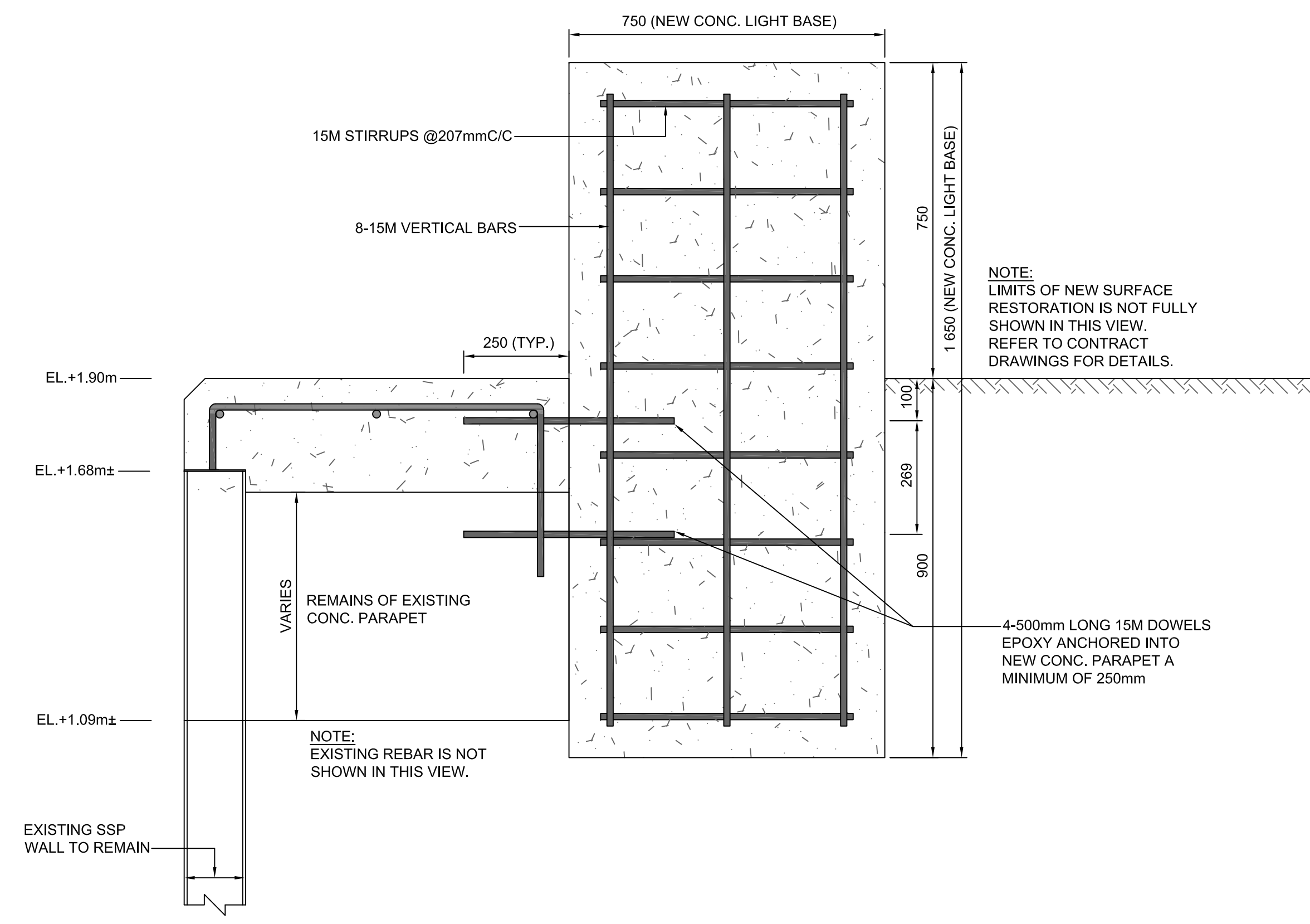
51 19/19 TYP. SECTION OF NEW CONC. BASE FOR LIGHT POLE (EAST WALL) SCALE: 1:10
