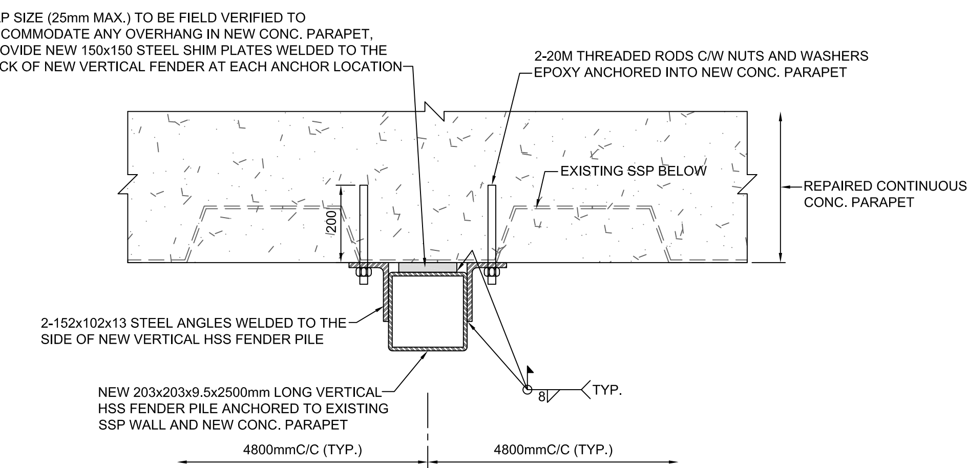
41 NEW VERTICAL FENDER TO CONC. PARAPET CONNECTION DETAIL (EAST WALL) SCALE: 1:10
