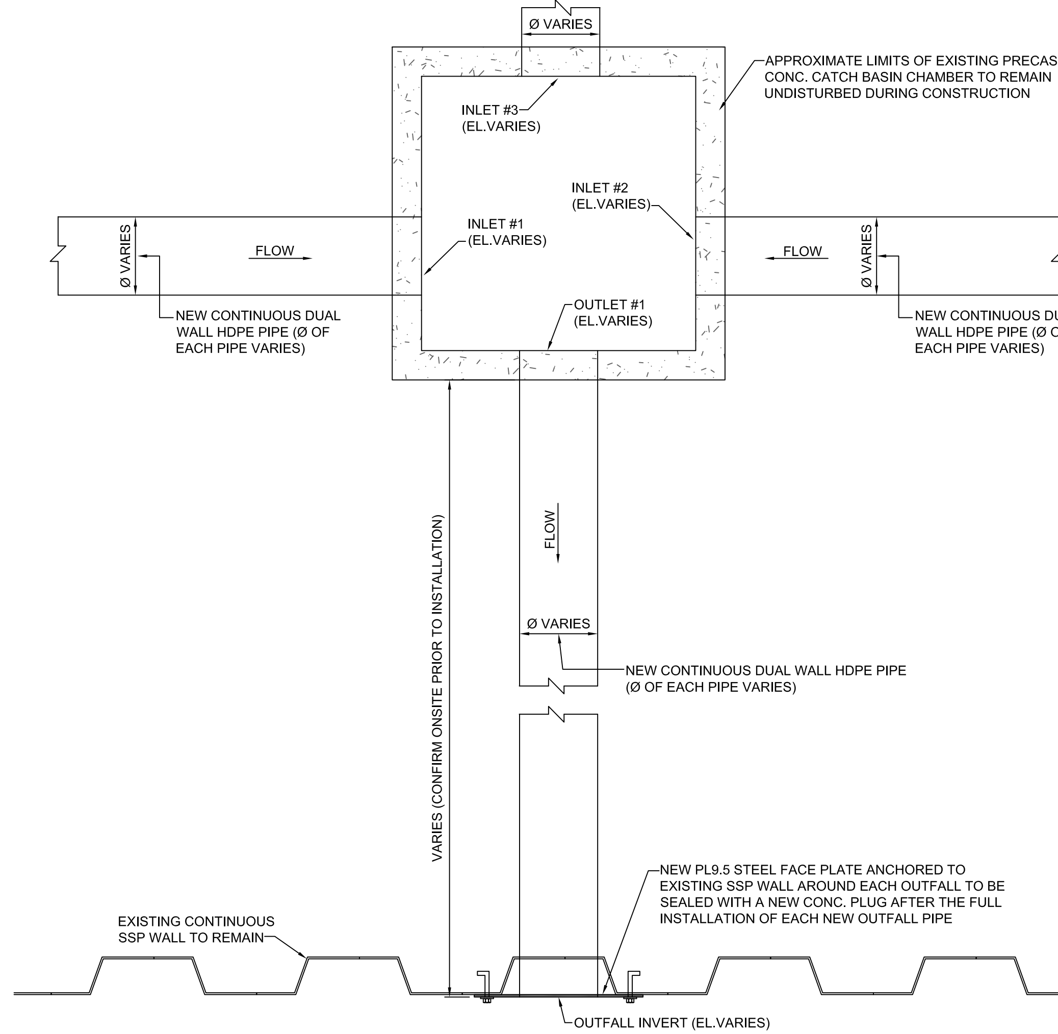
CONFIGURATION LAYOUT OF NEW OUTFALL PIPE REPAIRS AND INVERT SCHEDULE REFERENCE SCALE: 1:15
