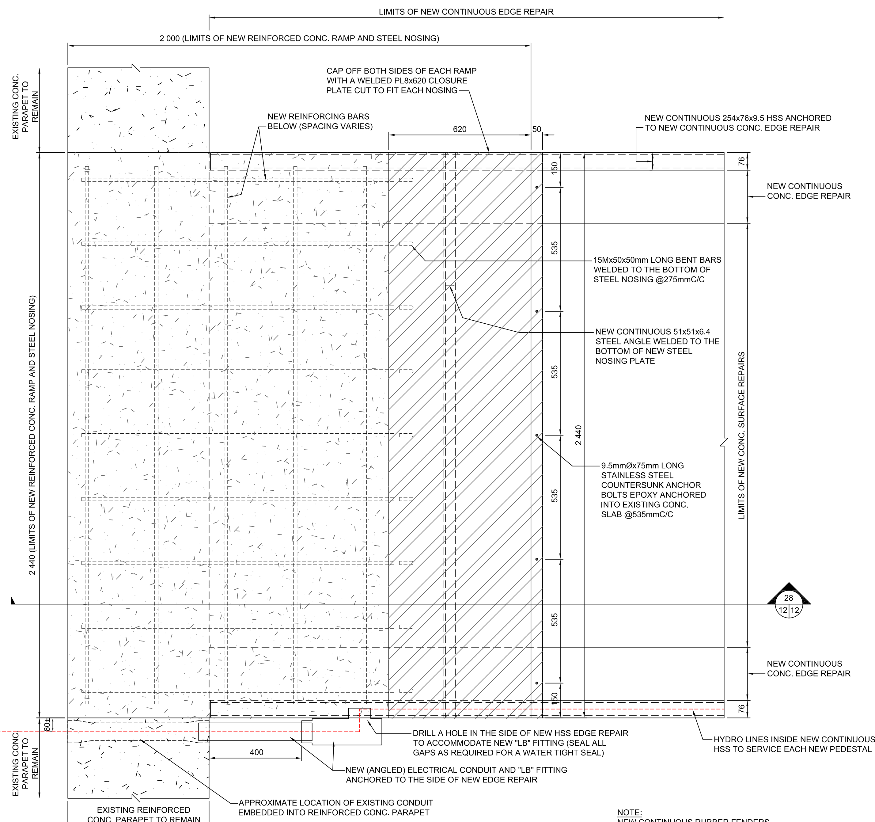
27 TYP. CONC. RAMP REPAIR DETAIL (JETTY 2,4,6) SCALE: 1:10
