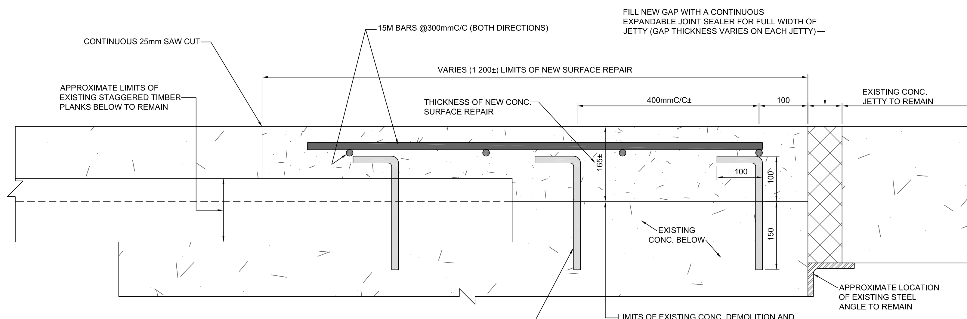
26 11/11 TYP. CONC. SURFACE REPAIR DETAIL (JETTY 2,4,6) SCALE: 1:5
