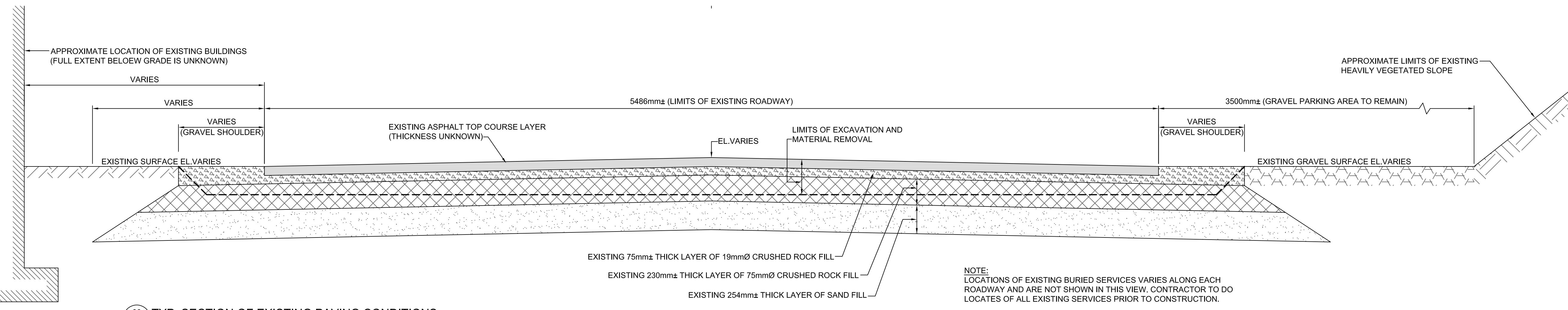
30 TYP. SECTION OF EXISTING PAVING CONDITIONS SCALE: 1:20
