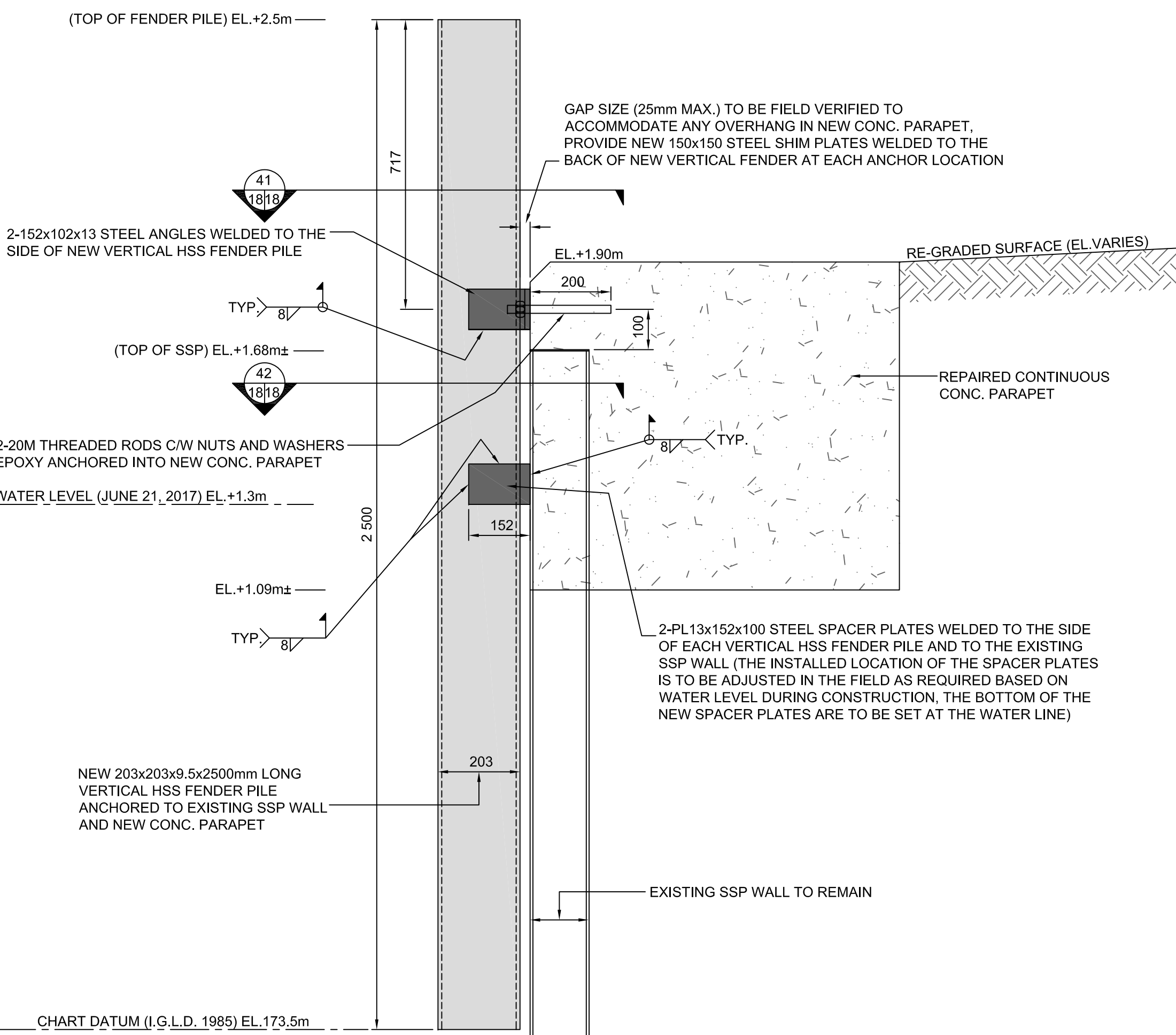
40 TYP. SECTION OF NEW VERTICAL FENDER (EAST WALL) SCALE: 1:10
