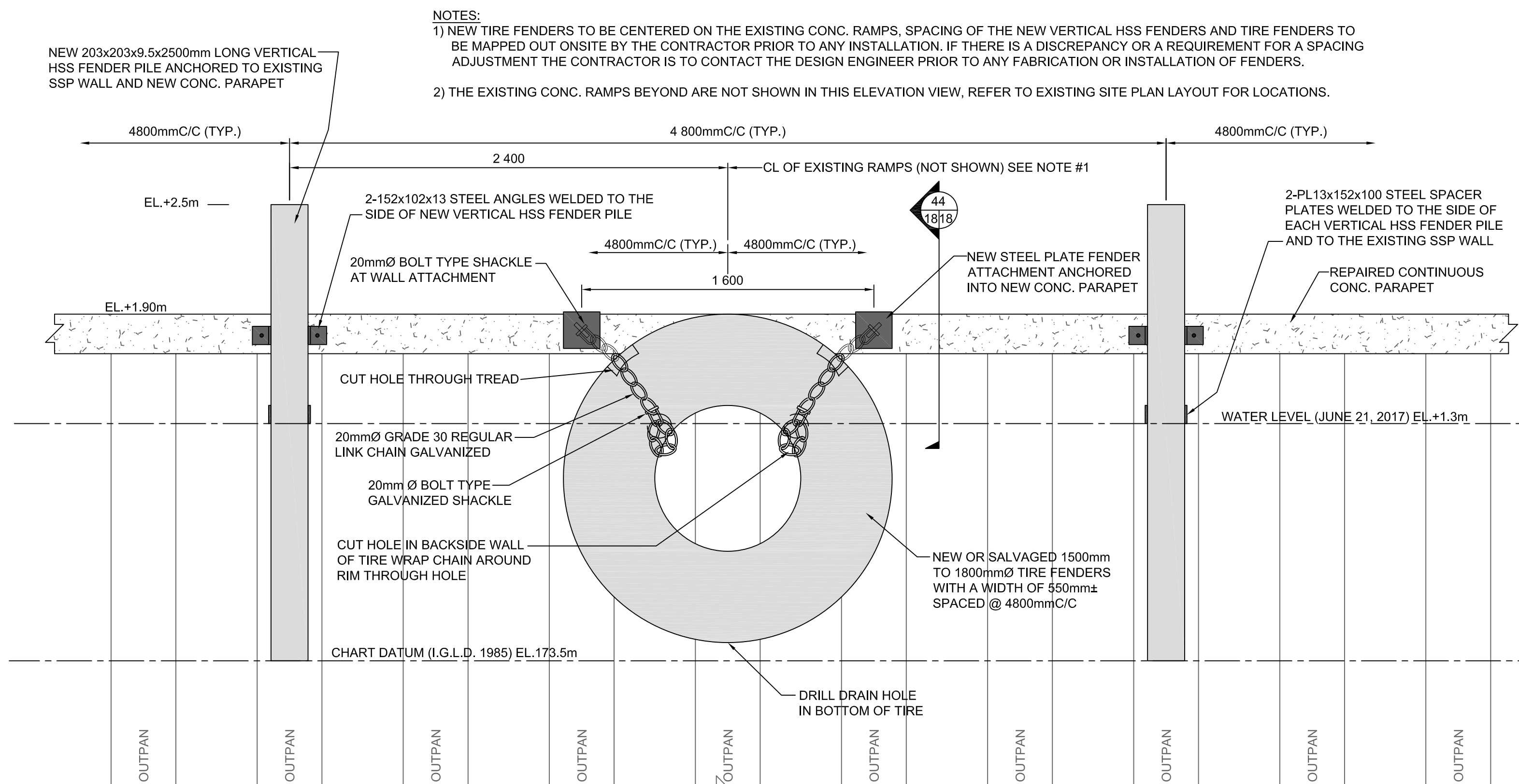
43 TYP. ELEVATION VIEW OF NEW TIRE FENDER (EAST WALL) SCALE: 1:20
