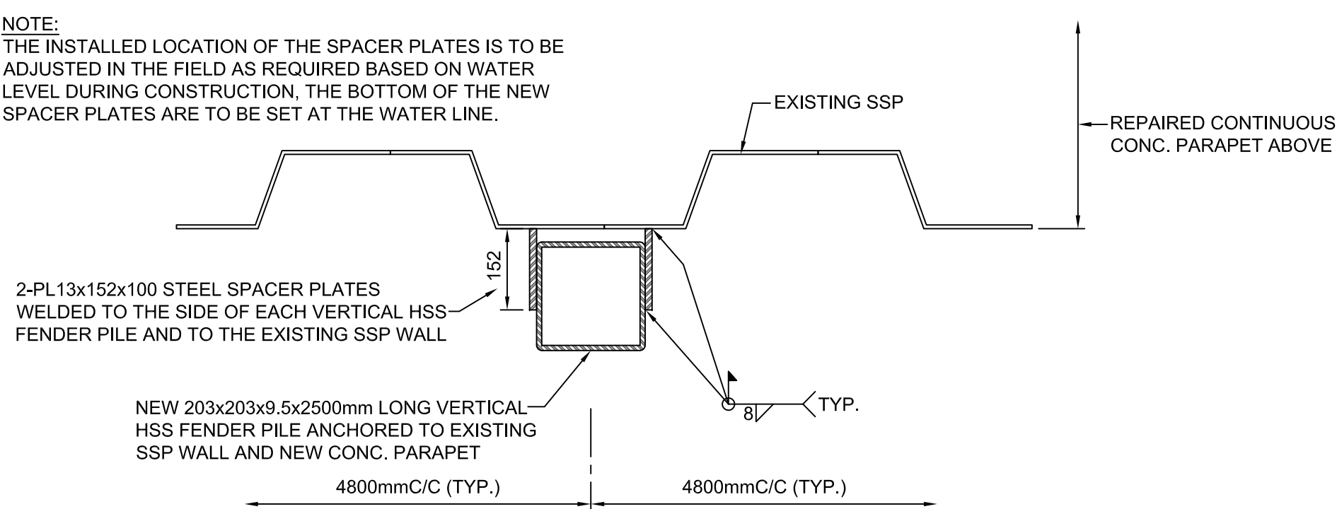
42 NEW VERTICAL FENDER TO SSP WALL CONNECTION DETAIL (EAST WALL) SCALE: 1:10
