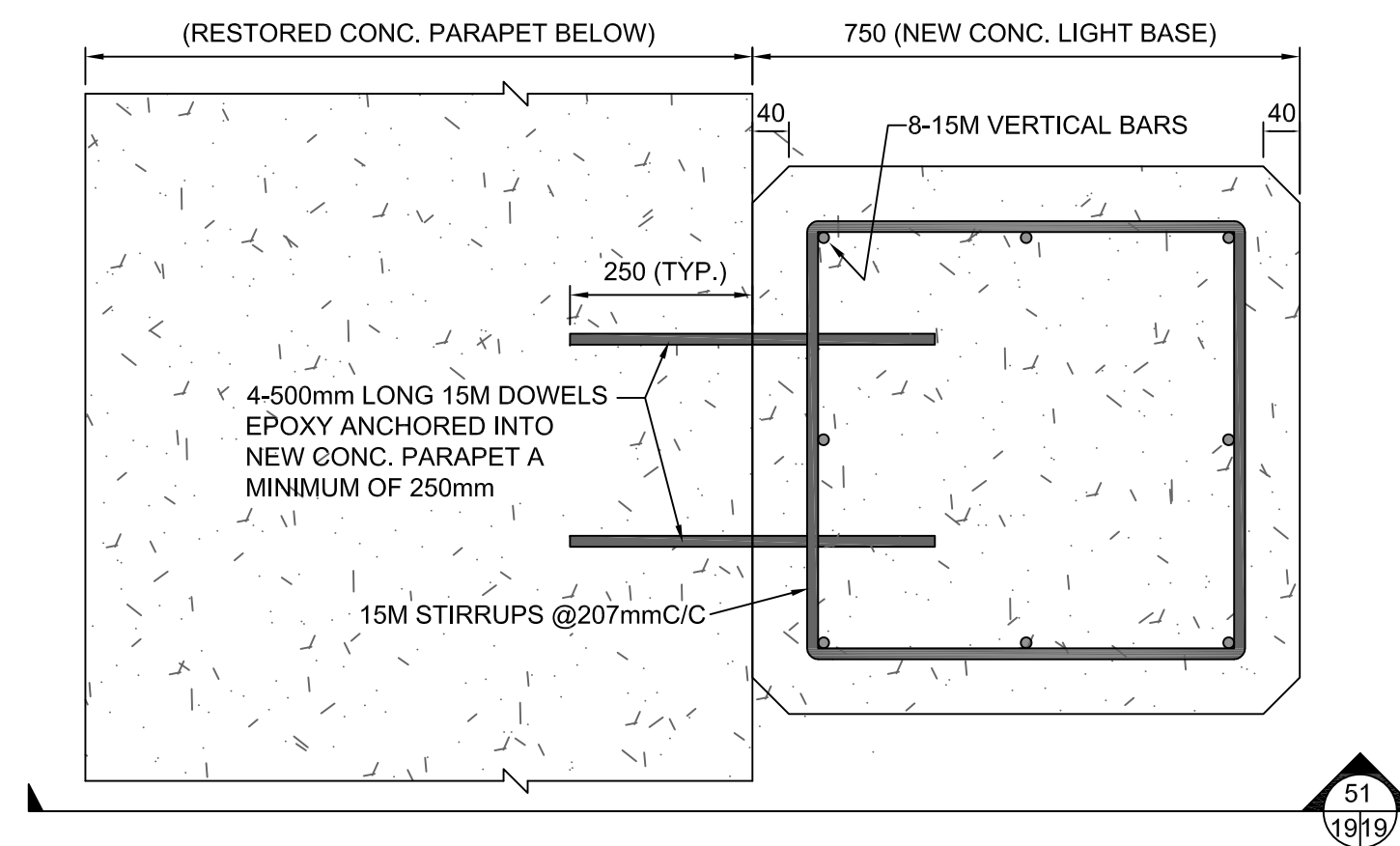
50 17/19 TYP. SECTION OF NEW CONC. BASE FOR LIGHT POLE (EAST WALL) SCALE: 1:10
