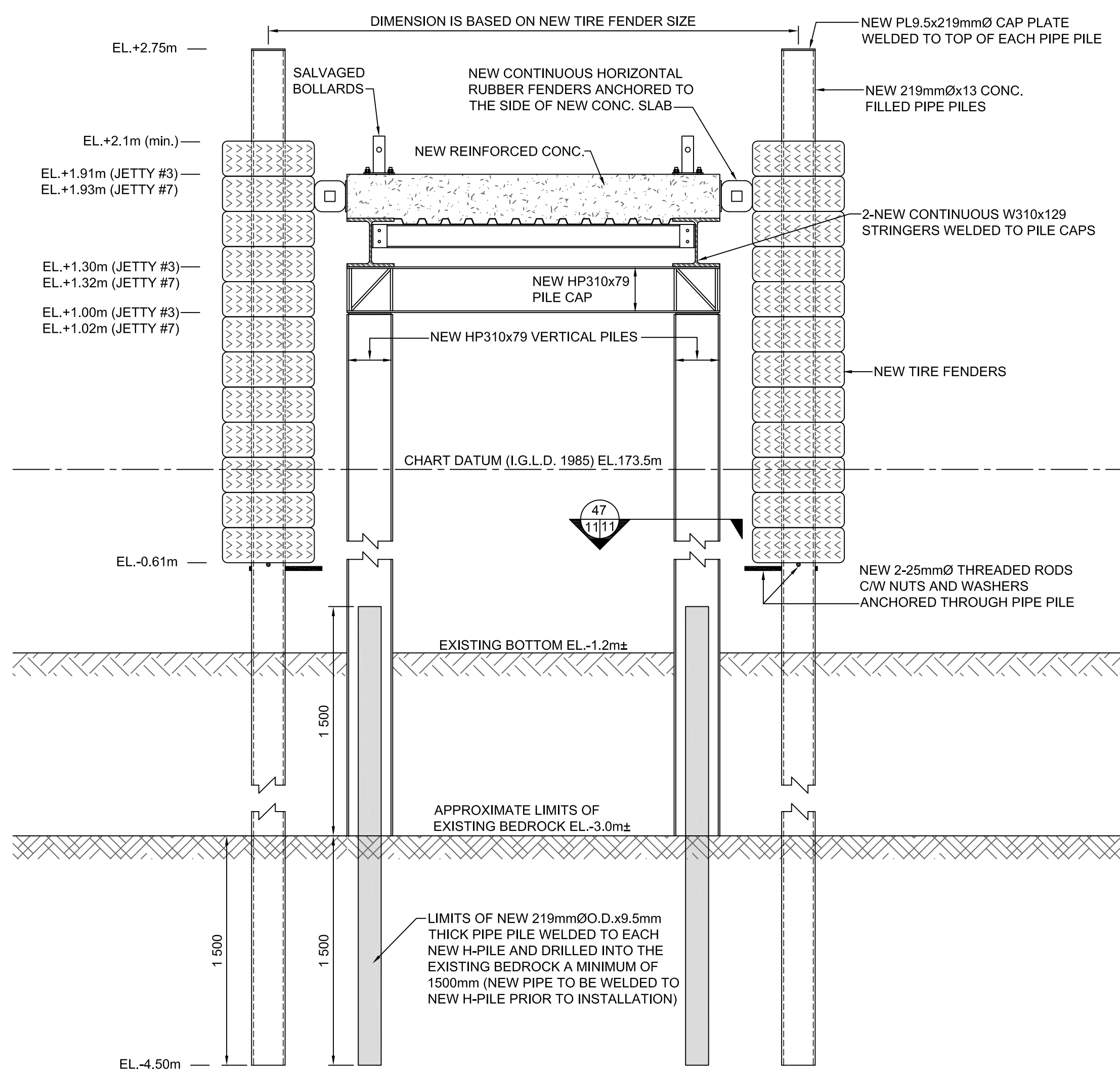
46 8/11 TYP. SECTION OF REPAIRED JETTY #3 & 7 SCALE: 1:25
