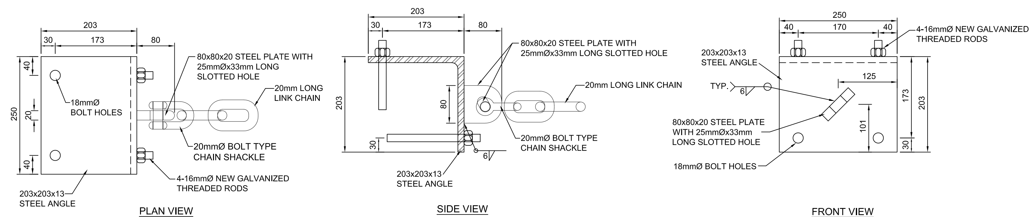
45 STEEL ANGLE FENDER ATTACHMENT DETAIL SCALE: 1:5
