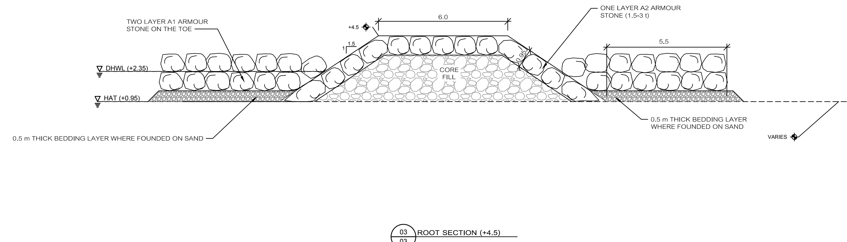
03 ROOT SECTION (+4.5)
