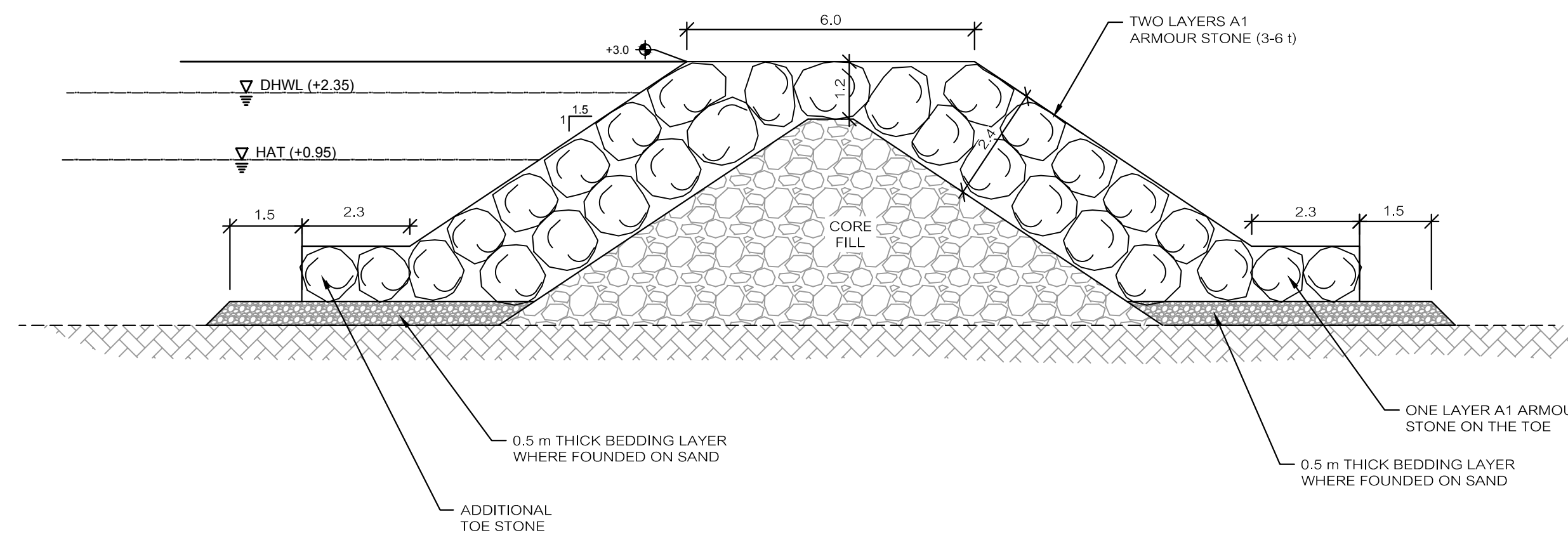
01 HEAD SECTION
