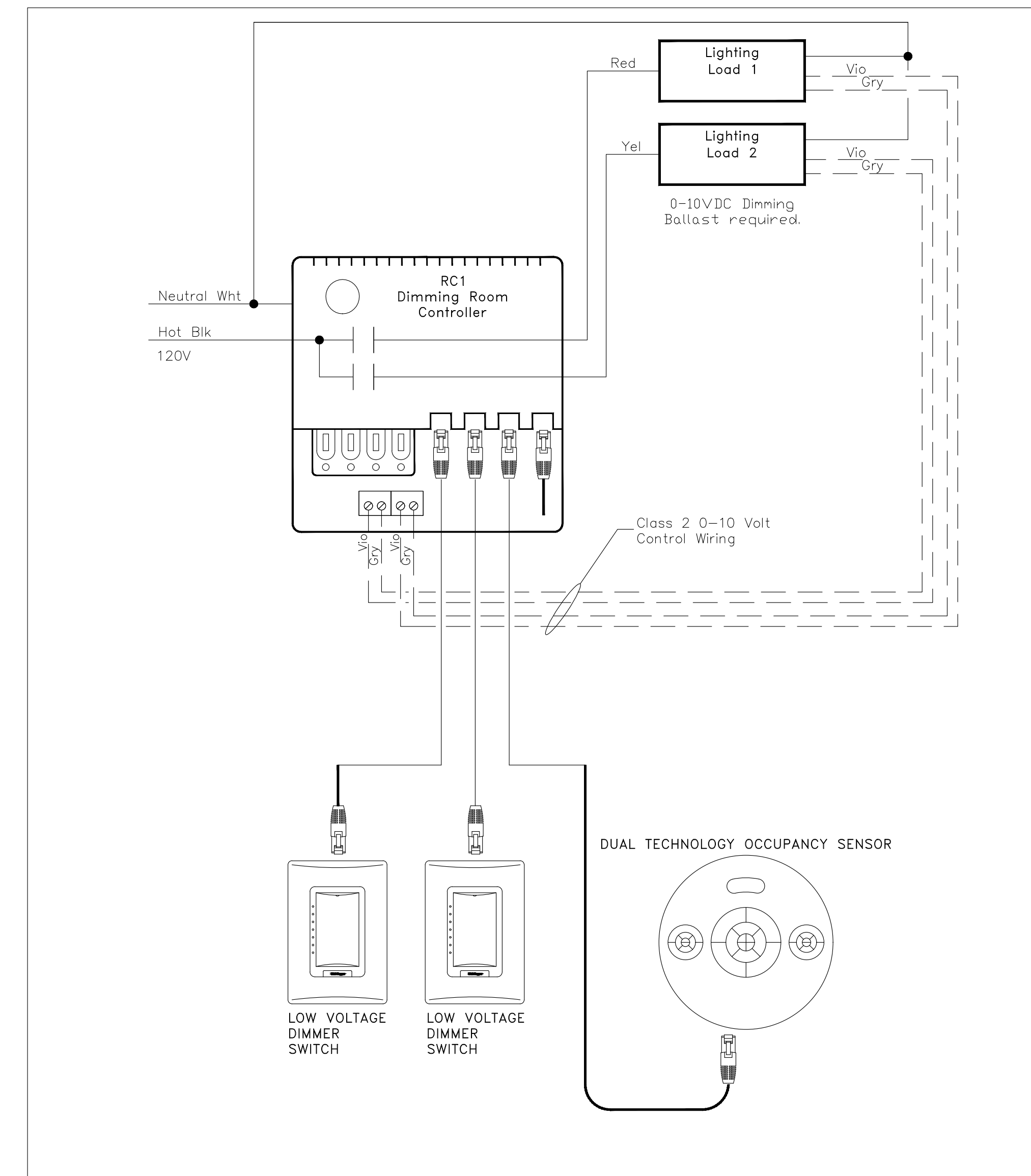
1 TYPICAL LIGHTING CONTROL DETAIL SCALE: N.T.S.
