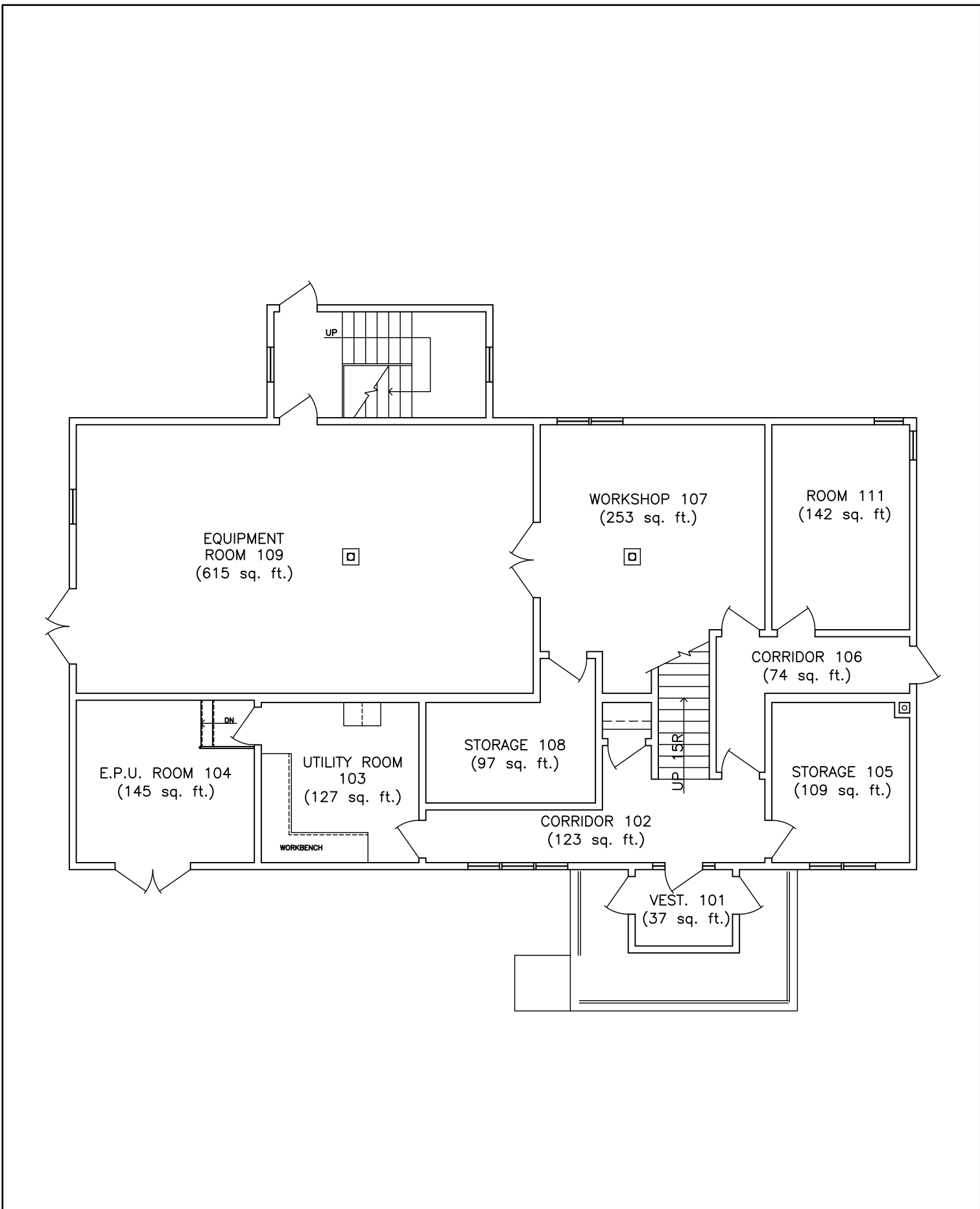
Port Aux Basques MCTS Centre - Level 1 Janitorial Services Contract - Drawing # 11O1101F02101
