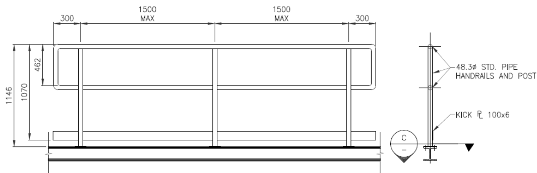
TYPICAL HANDRAIL DETAIL
