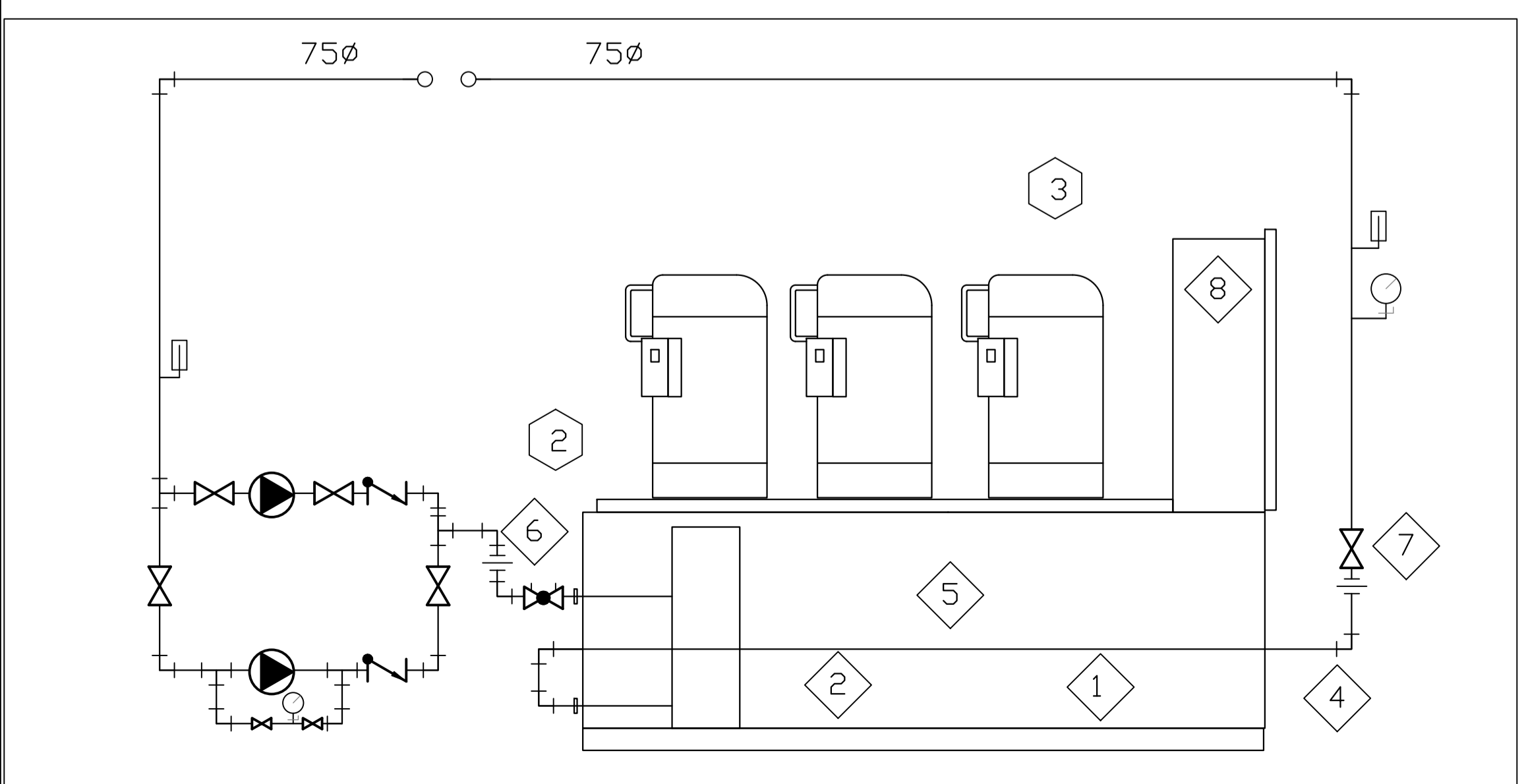
NEW INSTALLATION - SCHEMATIC
