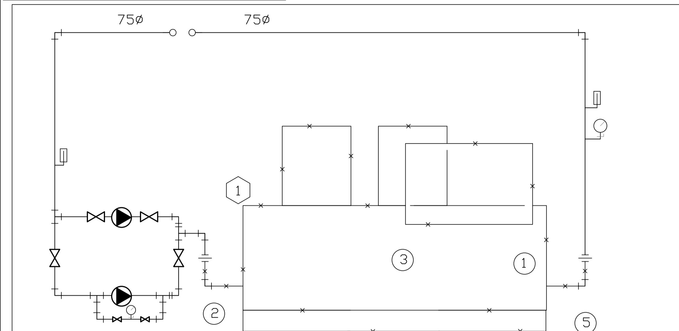
EXISTING AND DEMOLITION - SCHEMATIC
