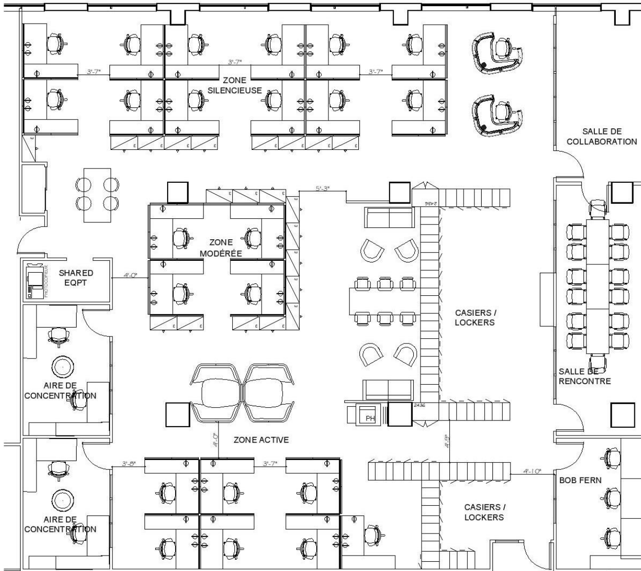
Floor plan:
